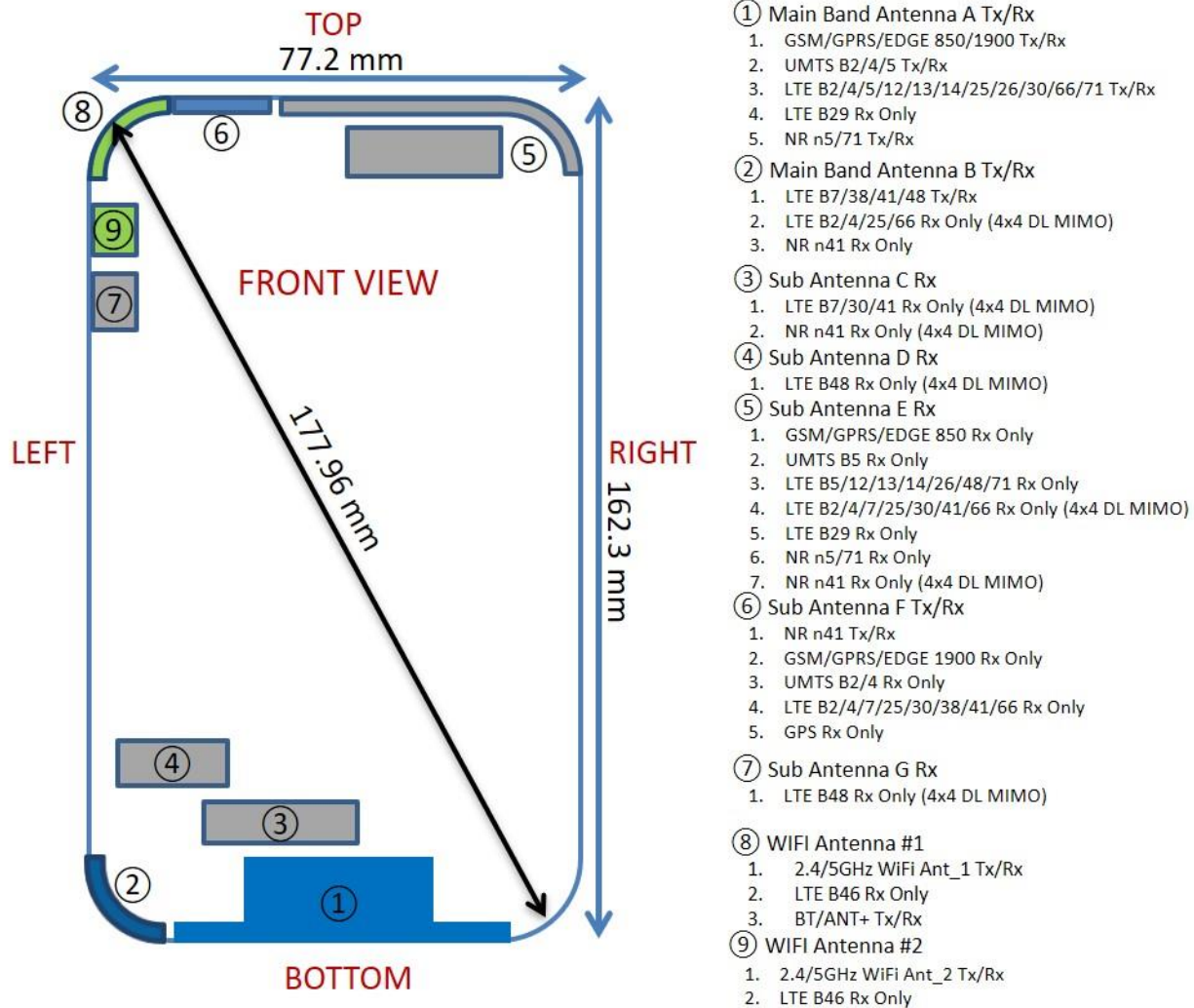
Figure E-1 DUT Antenna Locations
