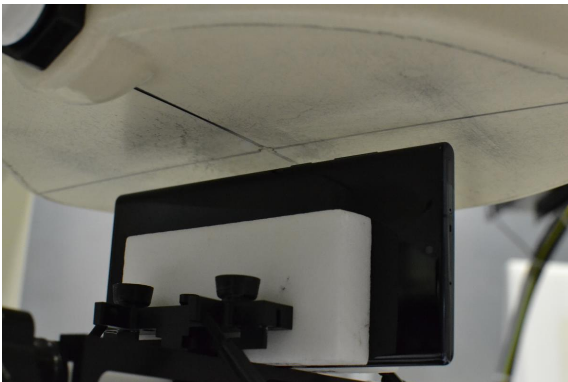
SAR Test Setup Photo 10 – Left Side at 10 mm
