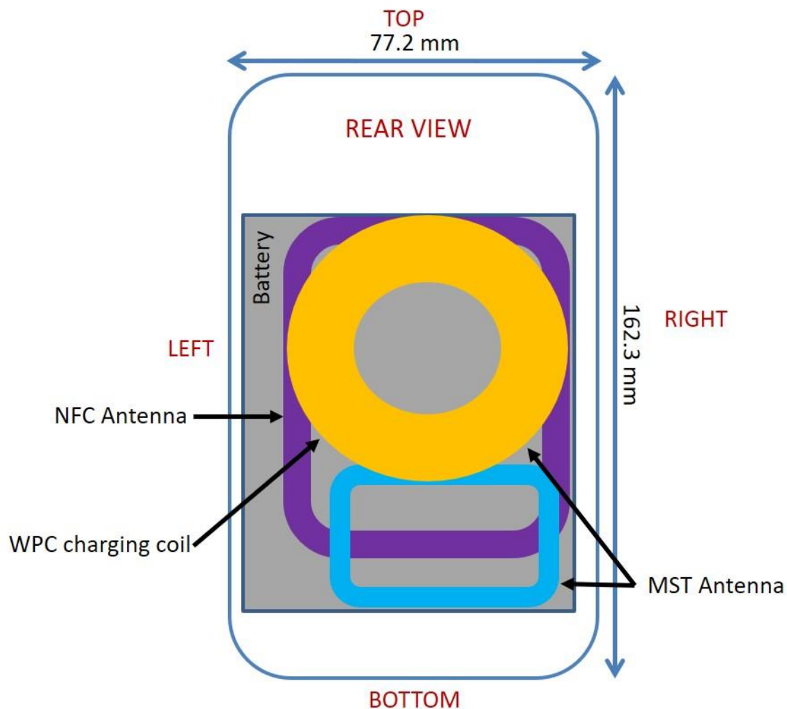
Figure E-2 NFC Antenna Locations
