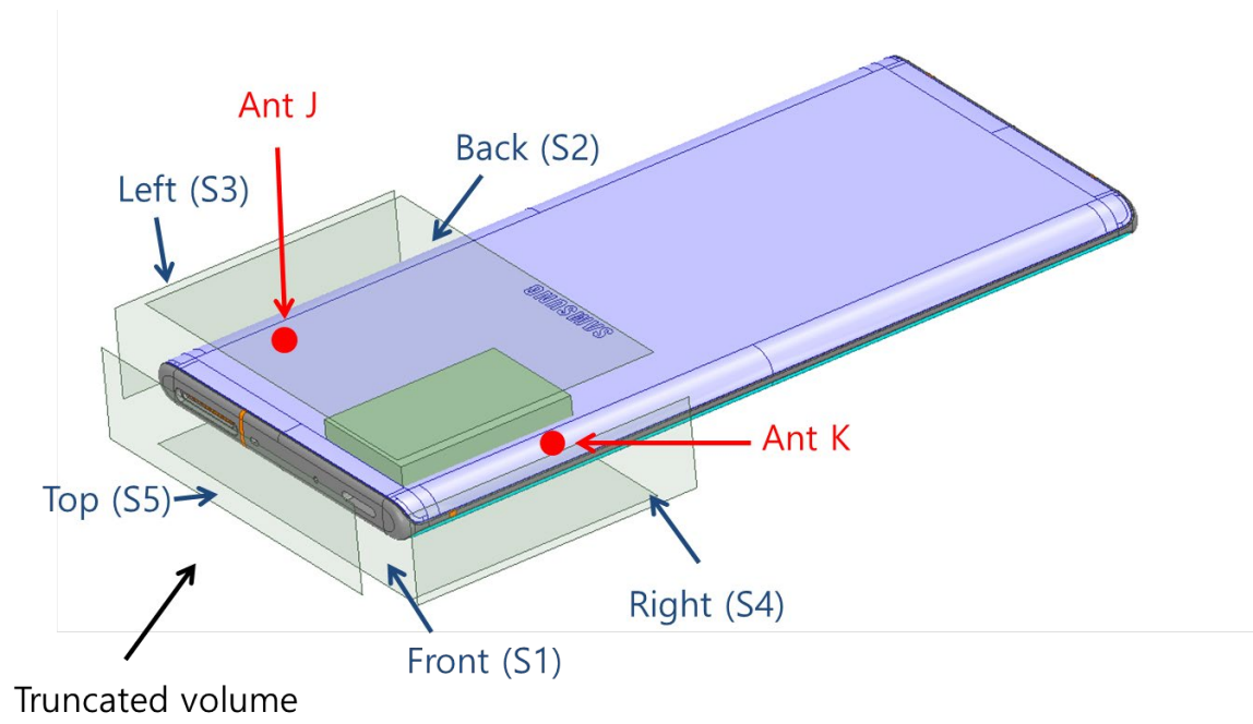
(a) Ant J and Ant K
