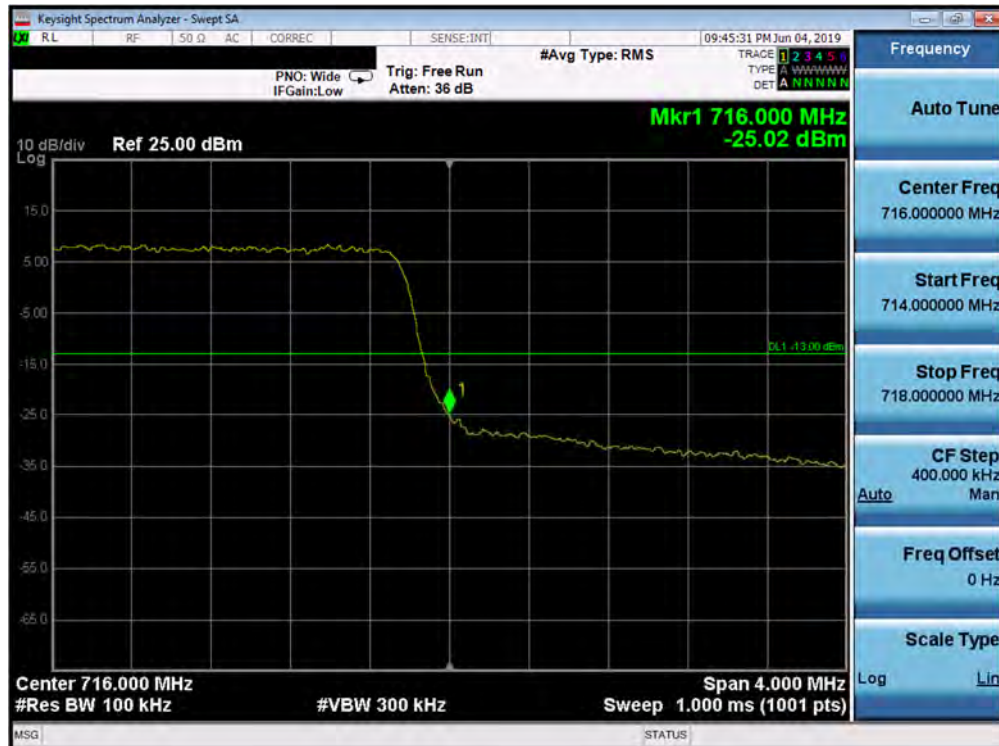
Plot 7-187. Upper Band Edge Plot (Band 12 - 5.0MHz QPSK - Full RB Configuration)
