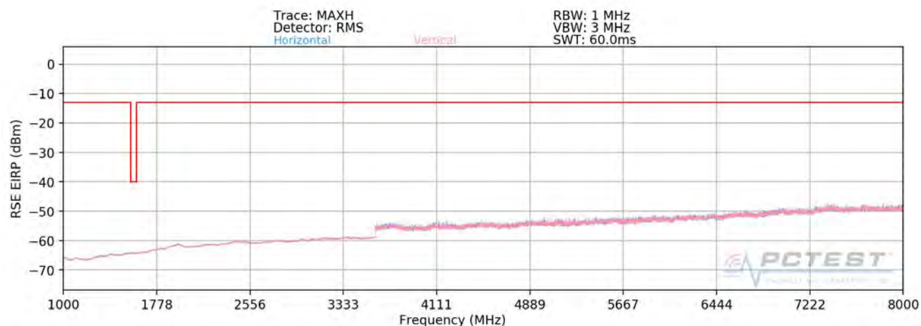
Plot 7-363. Radiated Spurious Plot above 1GHz (Band 13)
