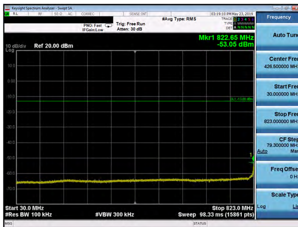
Plot 7-332. Conducted Spurious Plot (Band 5 – 10.0MHz QPSK – PCC 1/49 SCC 1/0 – Low Channel)
