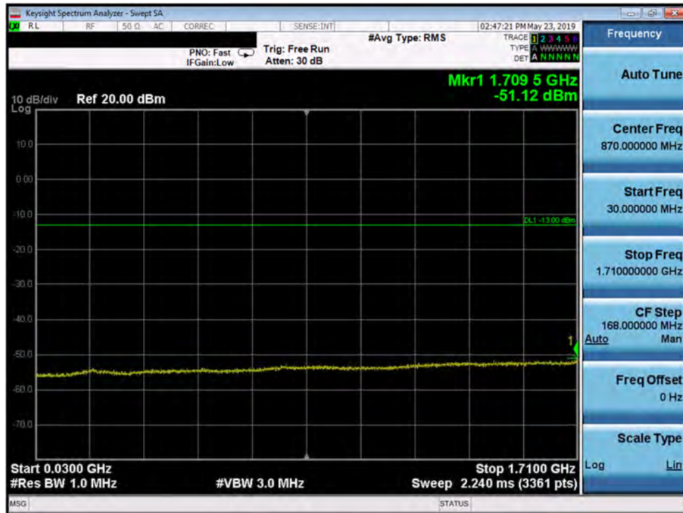
Plot 7-354. Conducted Spurious Plot (Band 66 – 20.0MHz QPSK – PCC 1/0 SCC 1/99 – High Channel)
