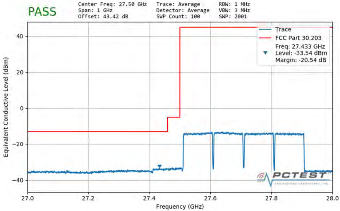
Plot 7-501. Lower Band Edge Plot (4CC 400MHz QPSK Full RB)
