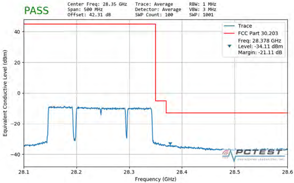
Plot 7-449. Upper Band Edge Plot (4CC 200MHz QPSK Full RB)
