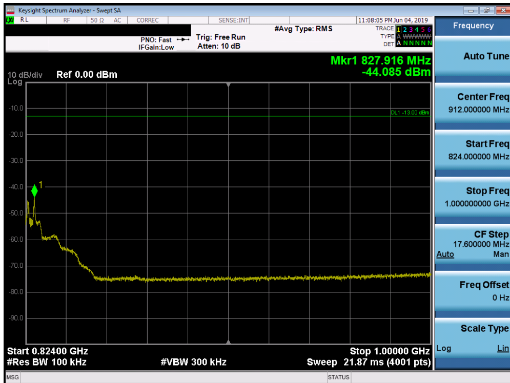
Plot 7-22. Conducted Spurious Plot (LTE Band 26, 15.0MHz QPSK – RB Size 1, RB Offset 0)
