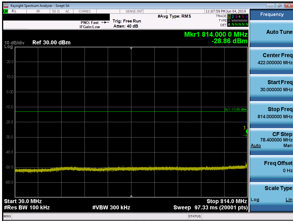
Plot 7-21. Conducted Spurious Plot (LTE Band 26, 15.0MHz QPSK – RB Size 1, RB Offset)
