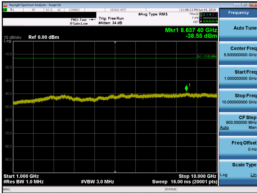
Plot 7-23. Conducted Spurious Plot (LTE Band 26, 15.0MHz QPSK – RB Size 1, RB Offset 0)
