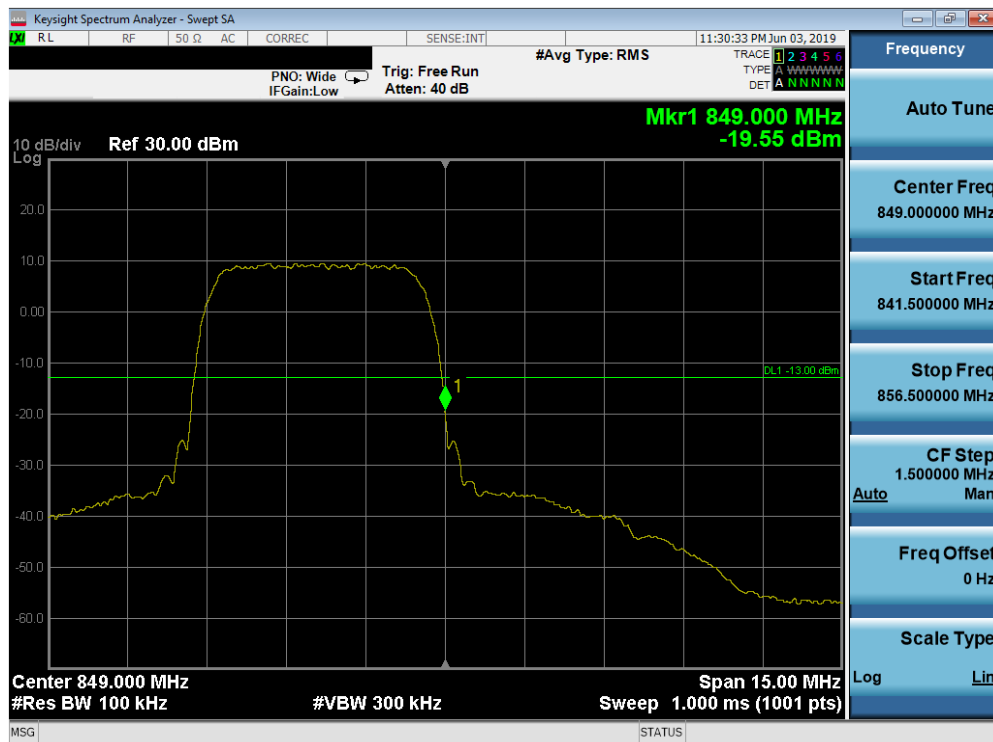
Plot 7-77. Band Edge Plot (Cellular WCDMA Mode - High Channel)
