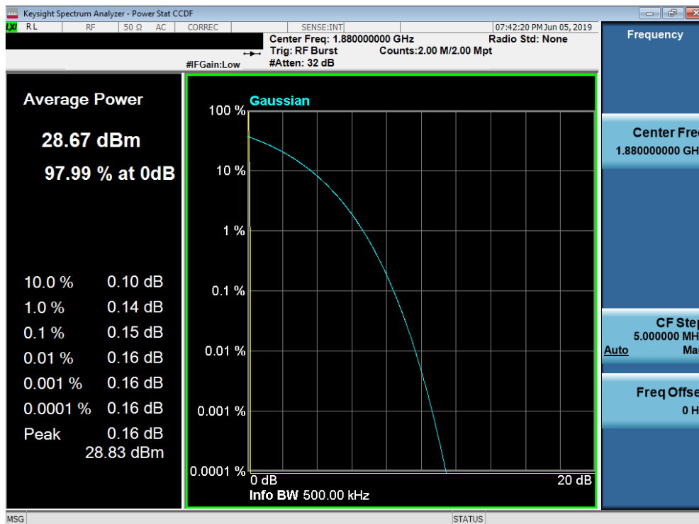
Plot 7-82. Peak-Average Ratio Plot (PCS GPRS Mode)
