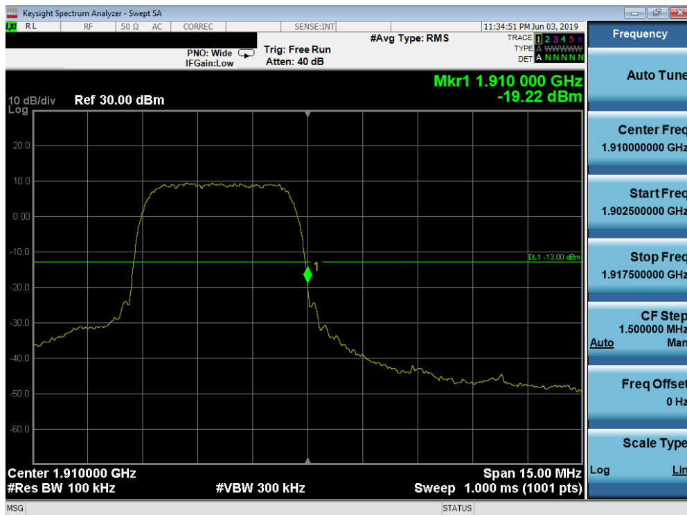
Plot 7-80. Band Edge Plot (PCS WCDMA Mode - High Channel)
