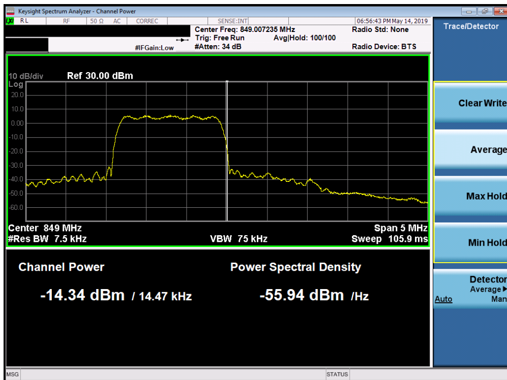
Plot 7-70. Band Edge Plot (Cellular CDMA Mode - High Channel)
