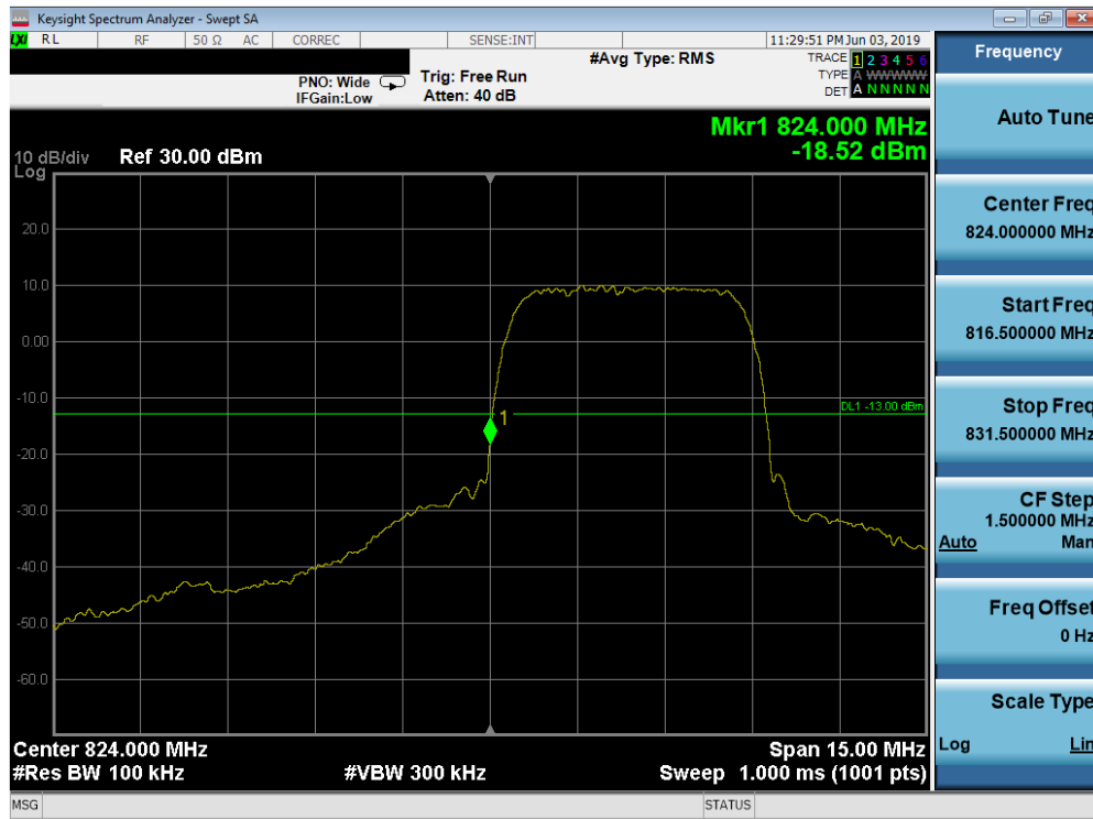
Plot 7-76. Band Edge Plot (Cellular WCDMA Mode - Low Channel)
