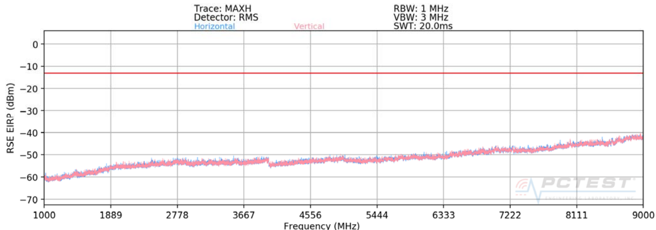
Plot 7-88. Radiated Spurious Plot above 1GHz (Cellular WCDMA Mode)
