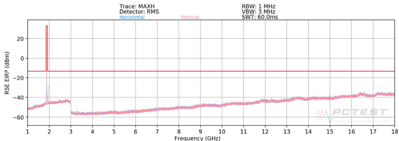
Plot 7-90. Radiated Spurious Plot above 1GHz (PCS CDMA Mode)
