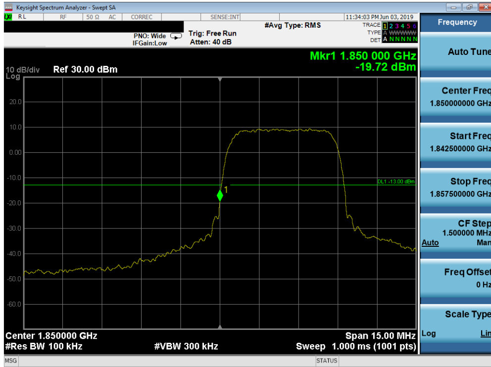
Plot 7-78. Band Edge Plot (PCS WCDMA Mode - Low Channel)
