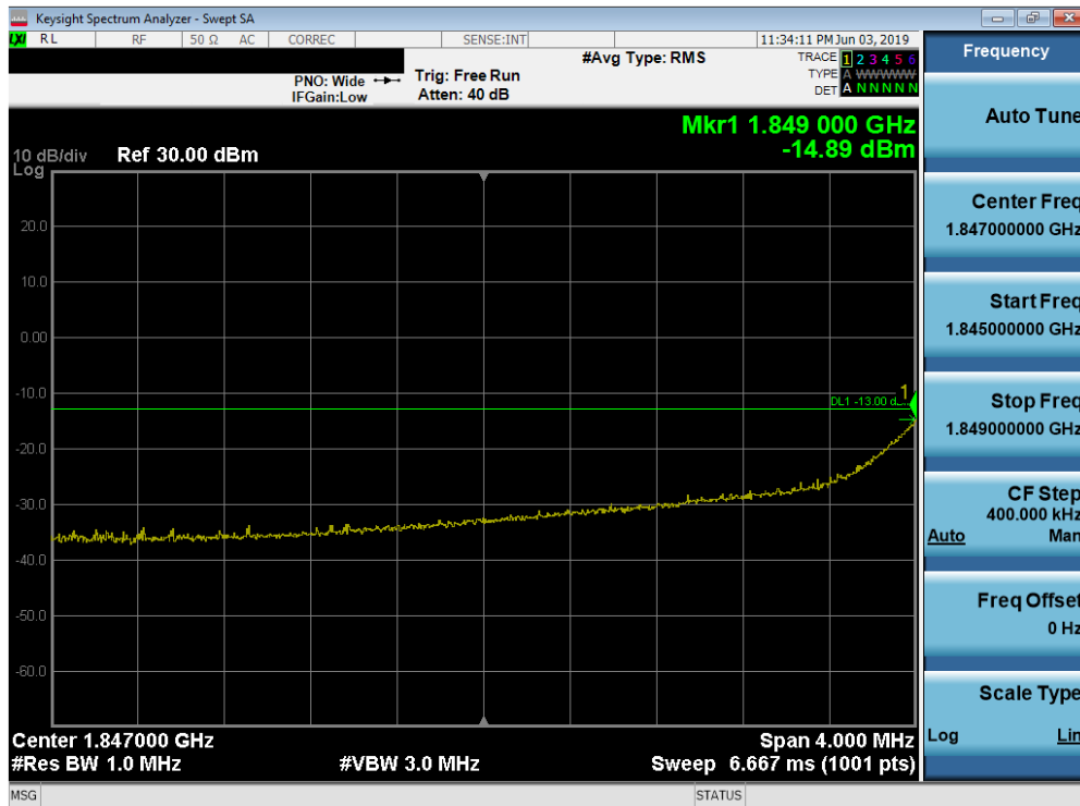
Plot 7-79. 4MHz Span Plot (PCS WCDMA Mode - Low Channel)
