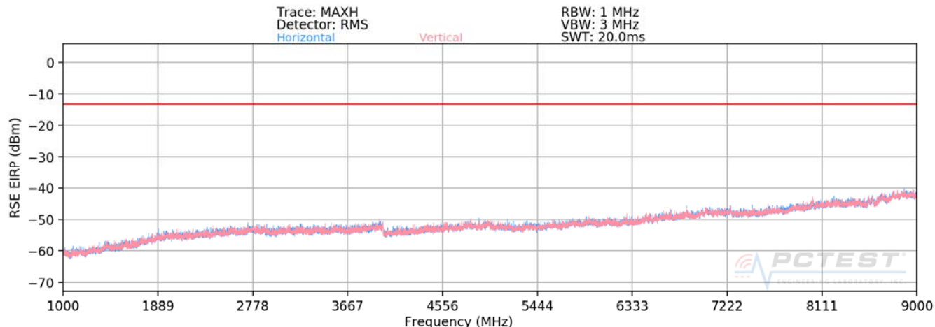
Plot 7-87. Radiated Spurious Plot above 1GHz (Cellular CDMA Mode)
