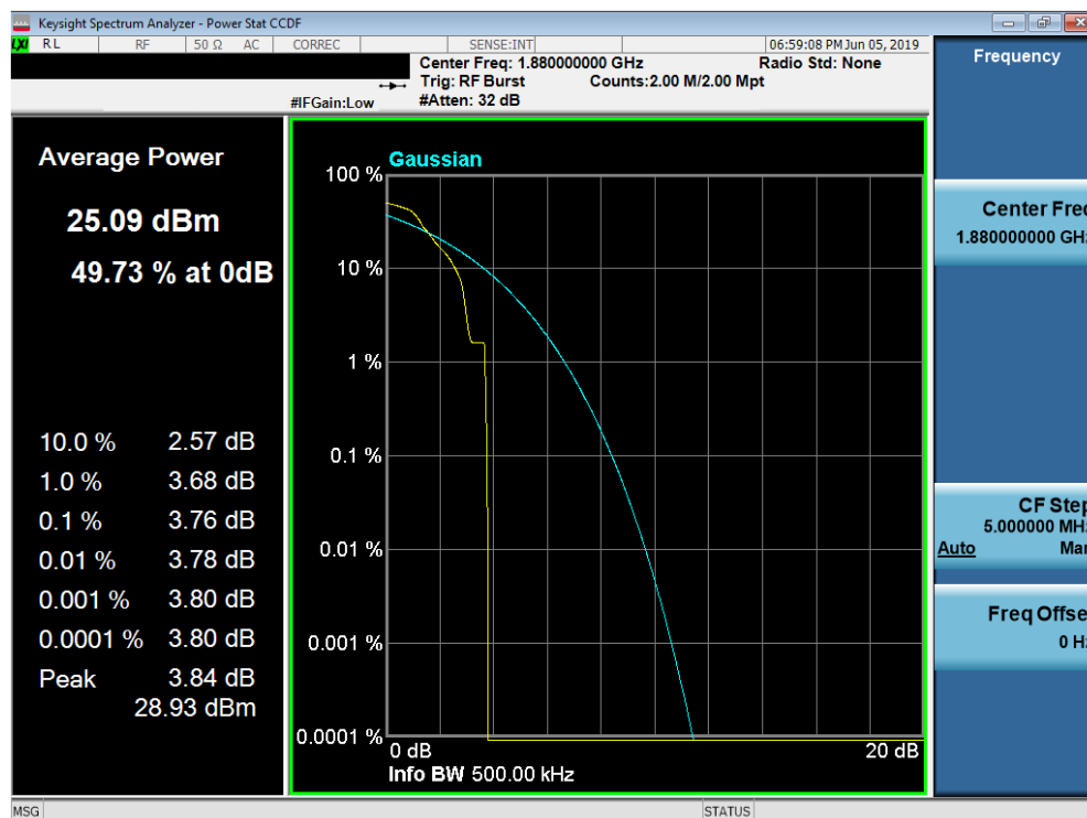
Plot 7-83. Peak-Average Ratio Plot (PCS EDGE Mode)
