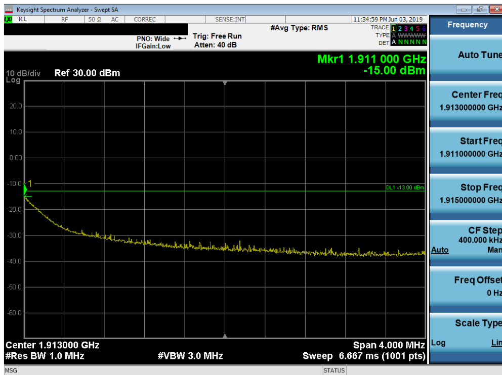
Plot 7-81. 4MHz Span Plot (PCS WCDMA Mode - High Channel)
