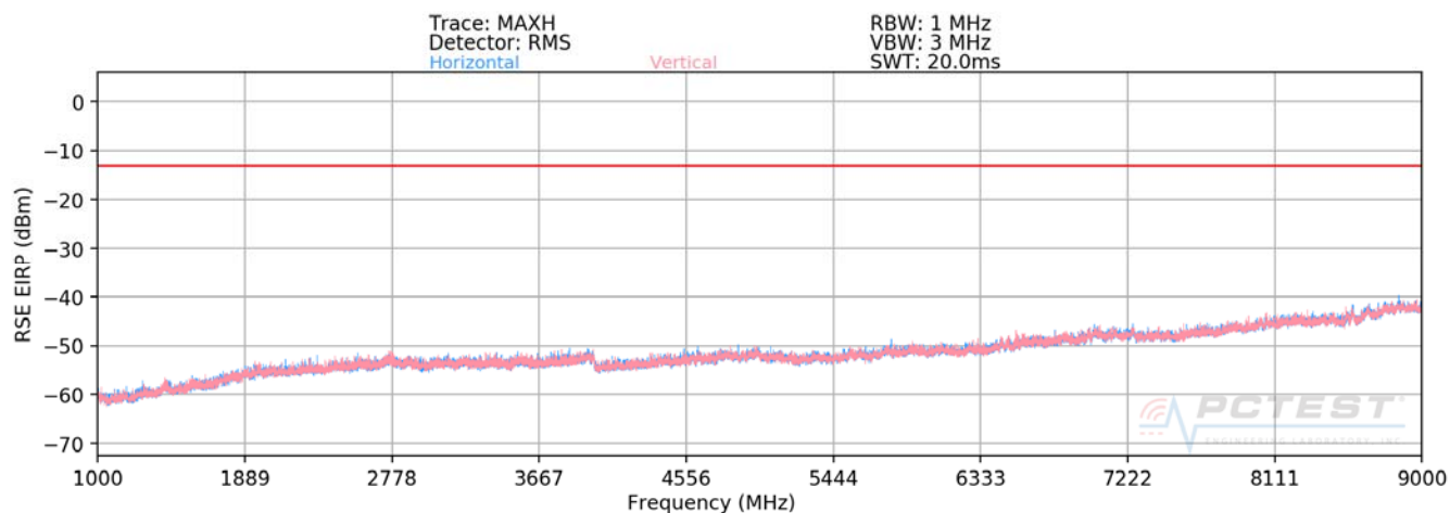
Plot 7-86. Radiated Spurious Plot above 1GHz (Cellular GPRS Mode)
