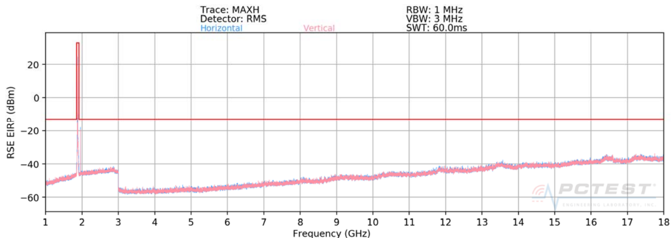
Plot 7-91. Radiated Spurious Plot above 1GHz (PCS WCDMA Mode)
