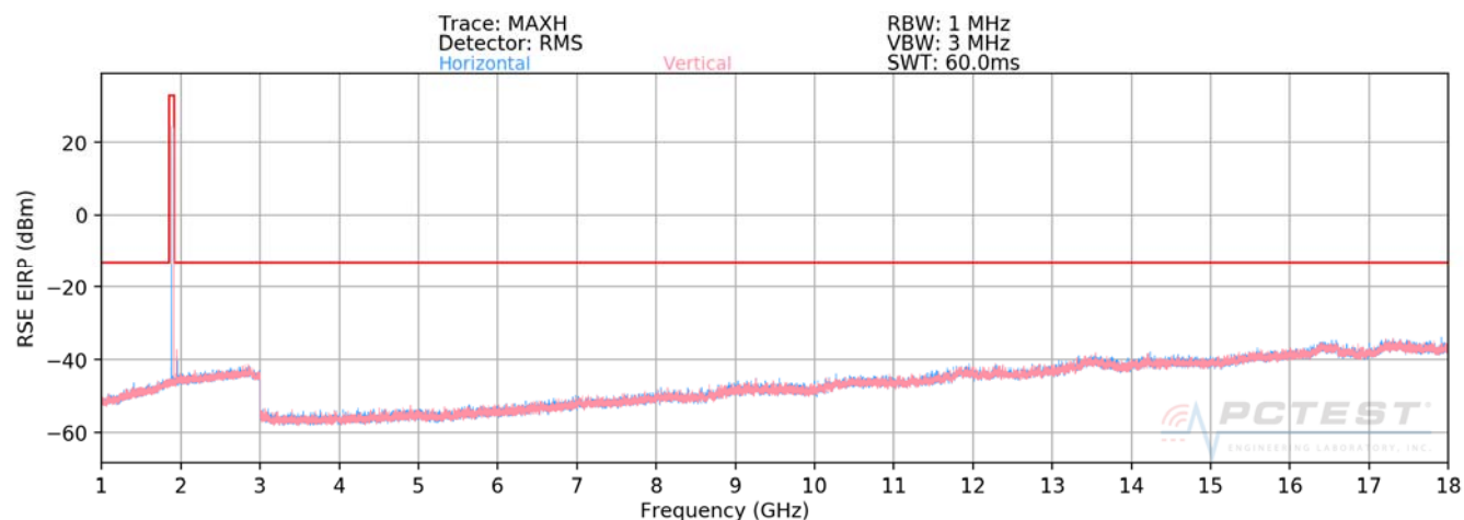
Plot 7-89. Radiated Spurious Plot above 1GHz (PCS GPRS Mode)
