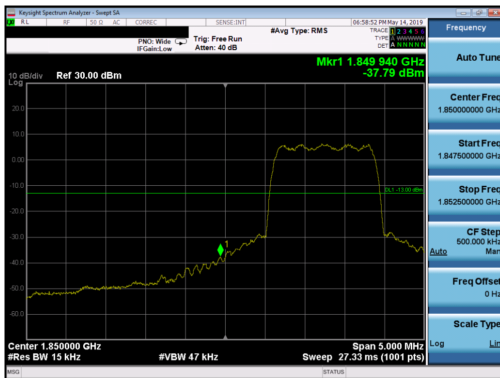
Plot 7-72. Band Edge Plot (PCS CDMA Mode - Low Channel)
