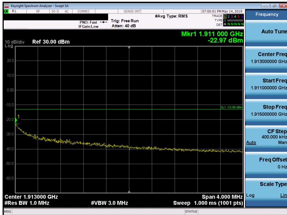
Plot 7-75. 4MHz Span Plot (PCS CDMA Mode - High Channel)
