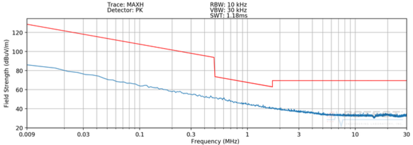
ot 7-10. Radiated Spurious Plot 9kHz – 30MHz (Pol. X – Digitizer Mode 2)
