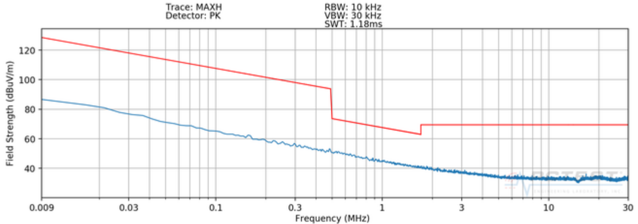
ot 7-7. Radiated Spurious Plot 9kHz – 30MHz (Pol. X – Digitizer Mode 1)
