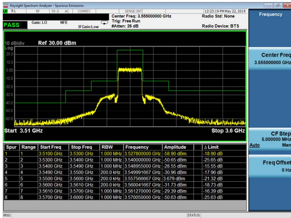
Plot 7-35. Lower Channel Edge Plot (Band 48 - 10.0MHz QPSK - Full RB Configuration)
