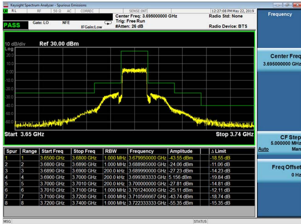
Plot 7-37. Upper Channel Edge Plot (Band 48 - 10.0MHz QPSK - Full RB Configuration)
