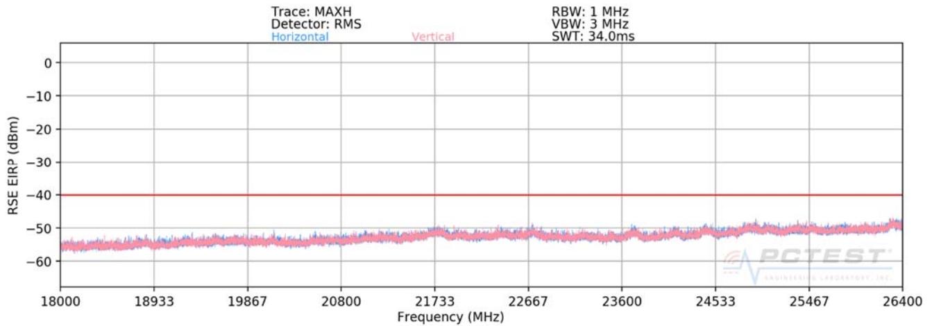
Plot 7-45. Radiated Spurious Plot 18 - 26.5GHz (Band 48)
