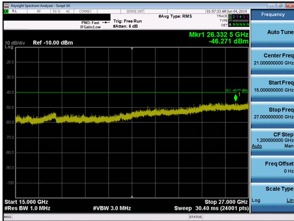
Plot 7-31. Conducted Spurious Plot (Band 48 - 20.0MHz QPSK - RB Size 1, RB Offset 99 - High Channel)
