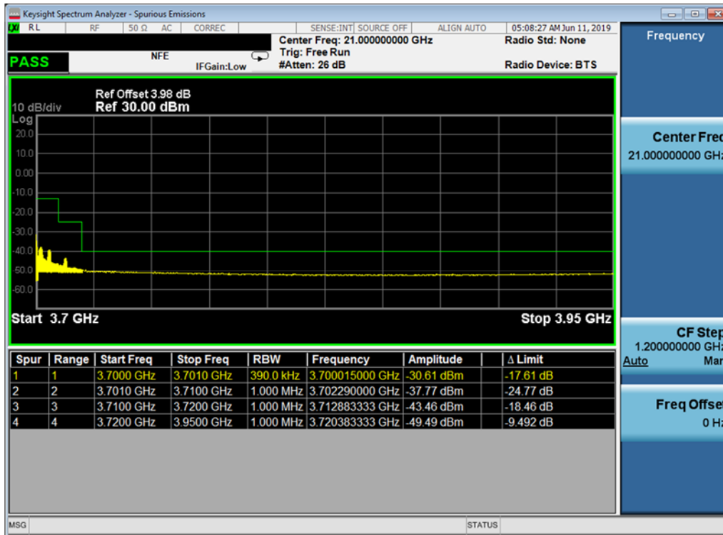
Plot 7-29. Conducted Spurious Plot (Band 48 - 20.0MHz QPSK - RB Size 1, RB Offset 99 – High Channel)
