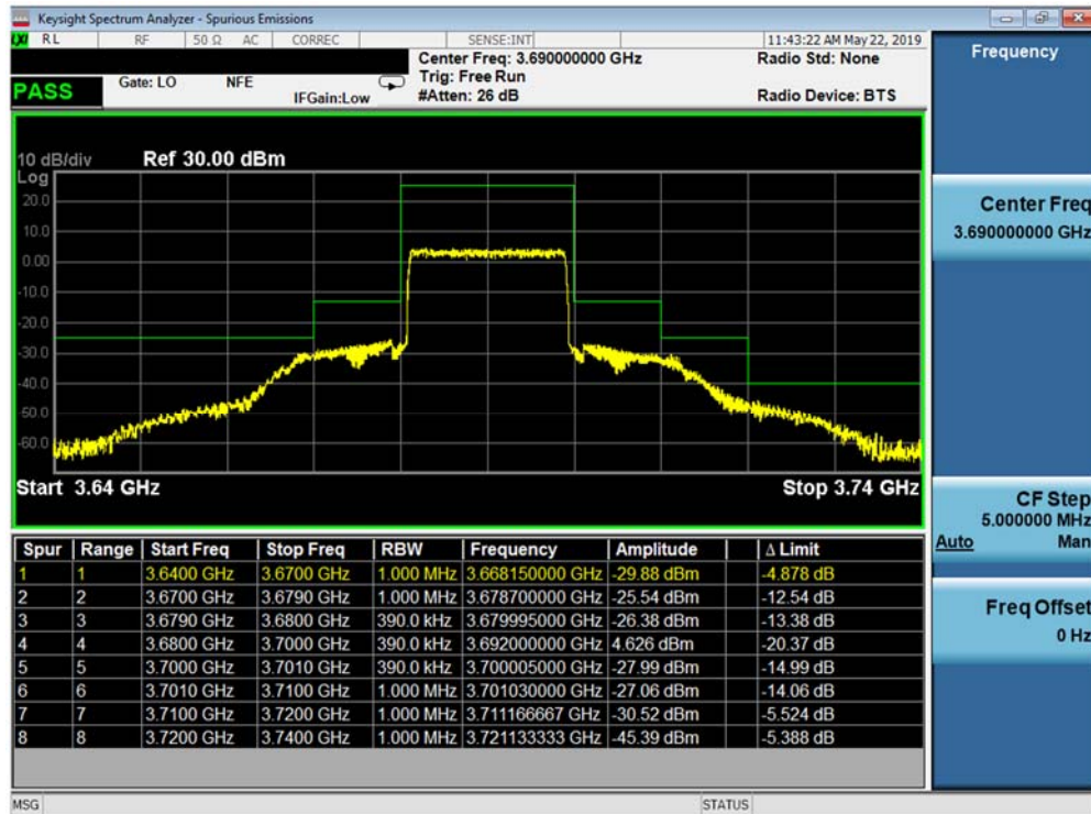
Plot 7-43. Upper Channel Edge Plot (Band 48 - 20.0MHz QPSK - Full RB Configuration)
