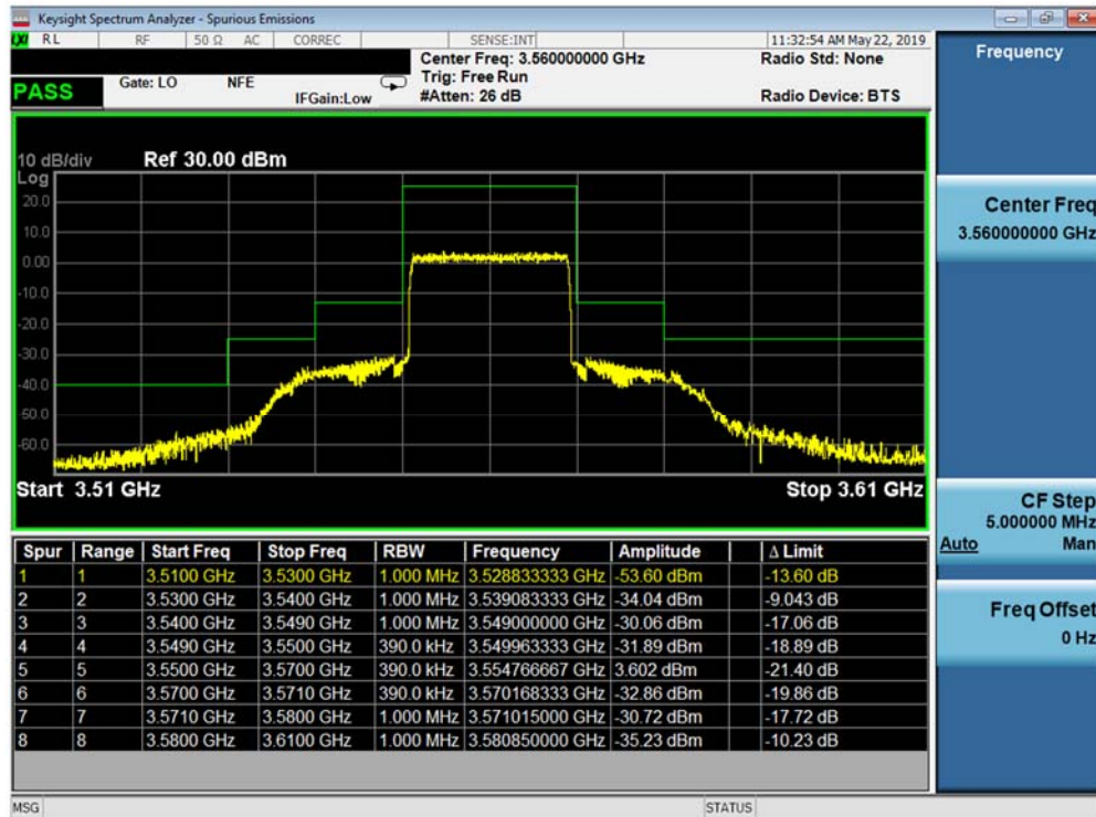
Plot 7-41. Lower Channel Edge Plot (Band 48 - 20.0MHz QPSK - Full RB Configuration)
