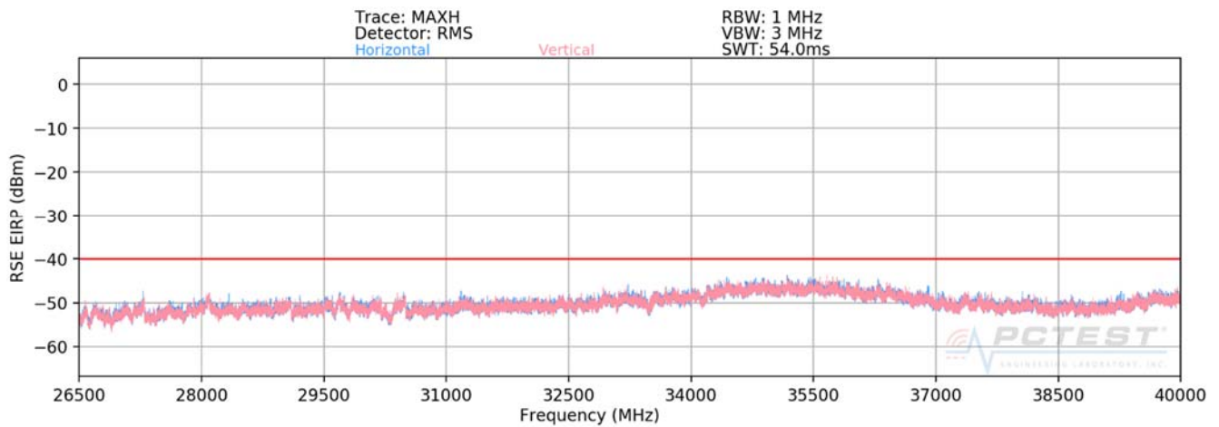
Plot 7-46. Radiated Spurious Plot 26.5 - 40GHz (Band 48)
