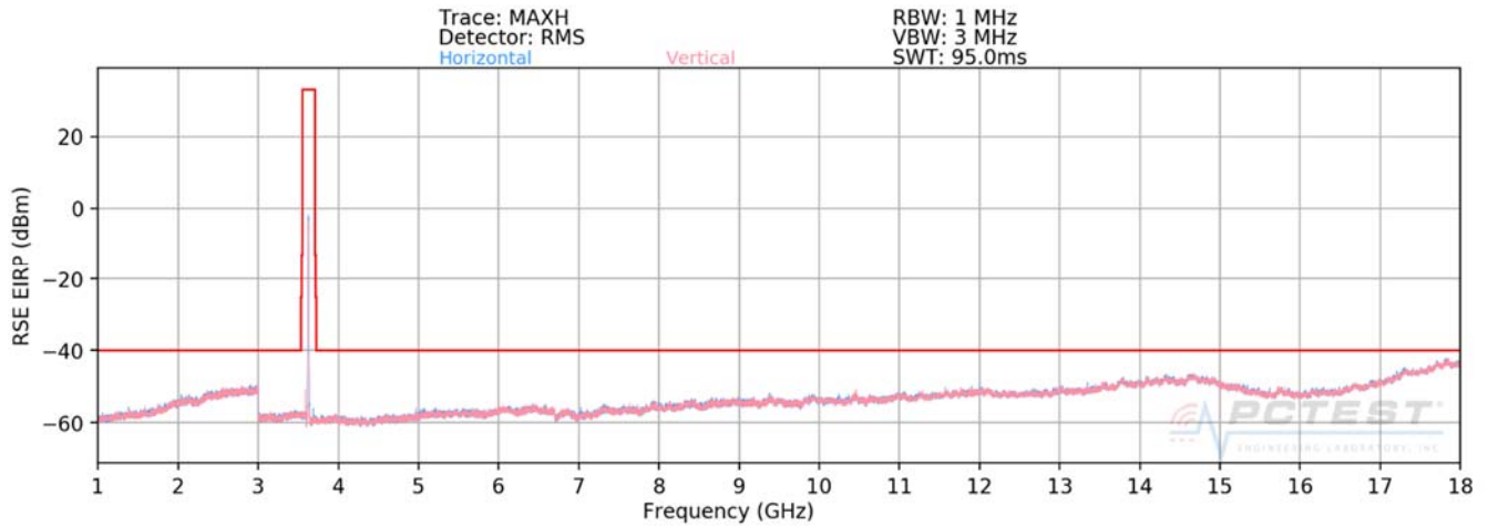
Plot 7-44. Radiated Spurious Plot 1 - 18GHz (Band 48)
