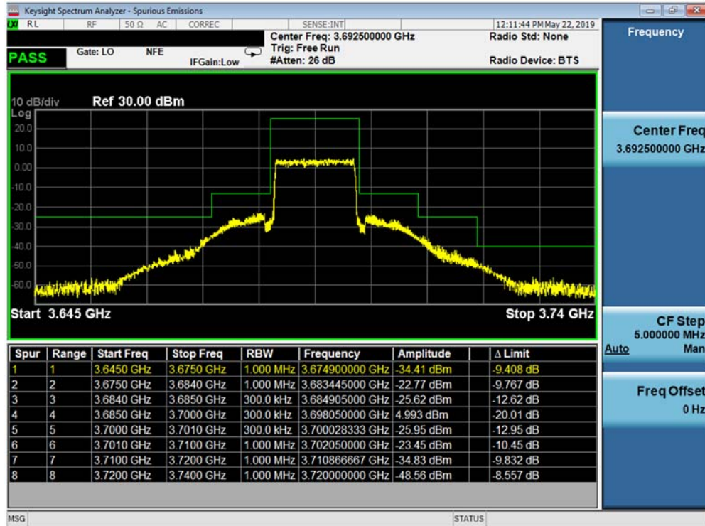
Plot 7-40. Upper Channel Edge Plot (Band 48 - 15.0MHz QPSK - Full RB Configuration)
