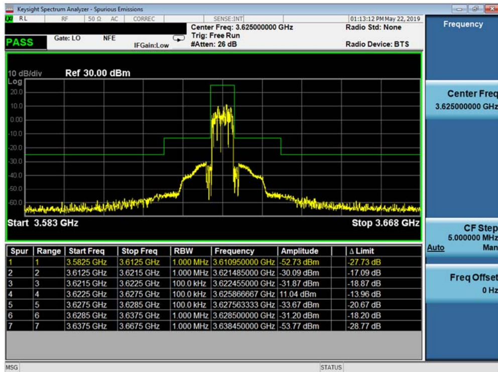
Plot 7-33. Mid Channel Edge Plot (Band 48 - 5.0MHz QPSK - Full RB Configuration)
