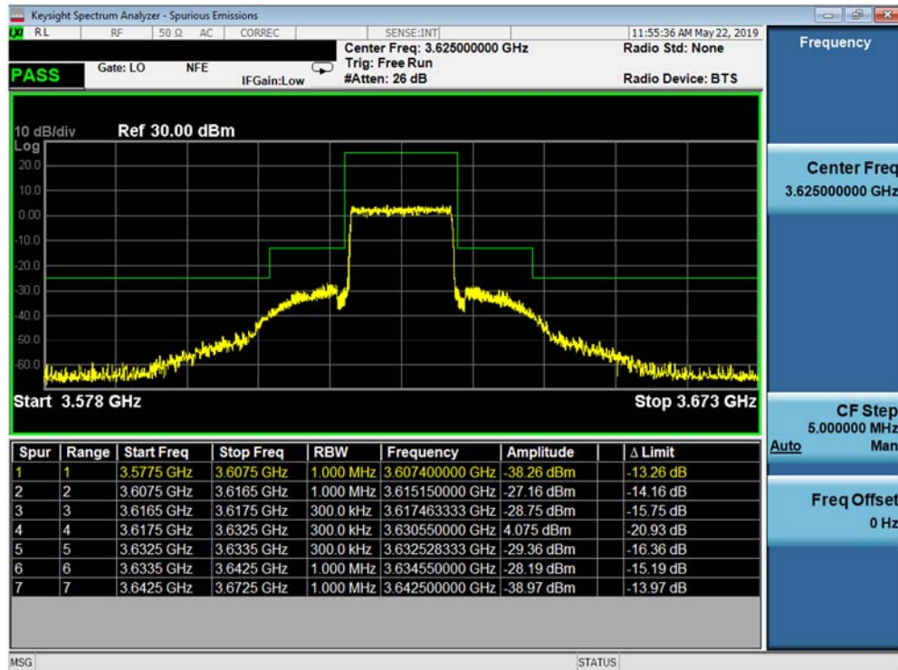
Plot 7-39. Mid Channel Edge Plot (Band 48 - 15.0MHz QPSK - Full RB Configuration)
