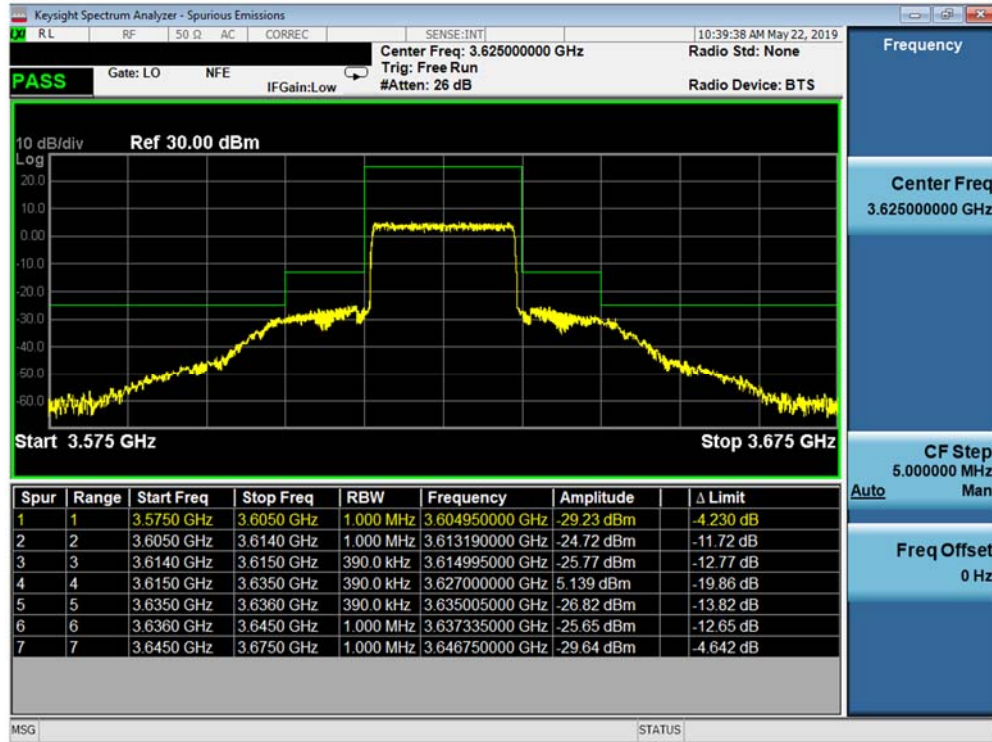
Plot 7-42. Mid Channel Edge Plot (Band 48 - 20.0MHz QPSK - Full RB Configuration)
