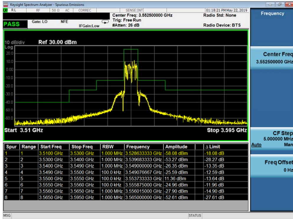
Plot 7-32. Lower Channel Edge Plot (Band 48 - 5.0MHz QPSK - Full RB Configuration)
