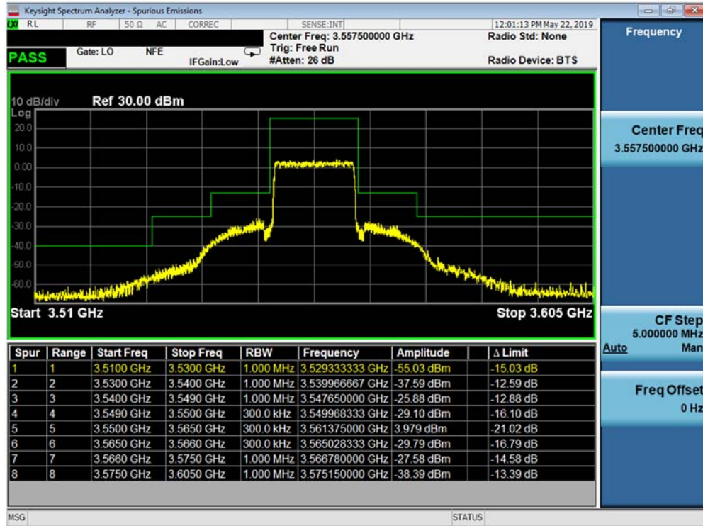
Plot 7-38. Lower Channel Edge Plot (Band 48 - 15.0MHz QPSK - Full RB Configuration)
