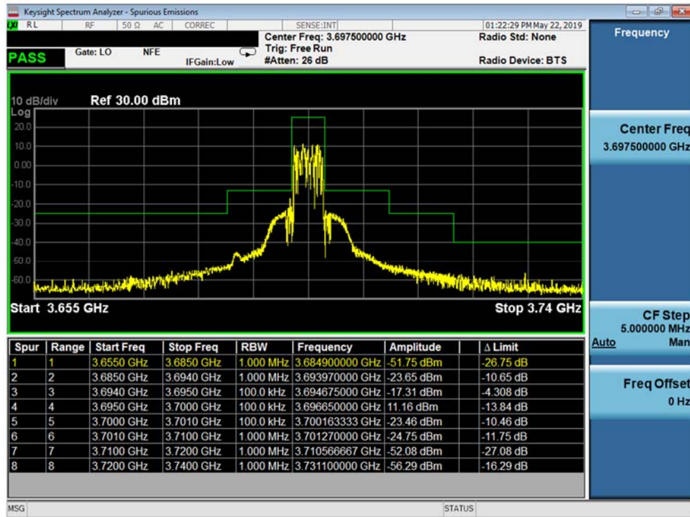
Plot 7-34. Upper Channel Edge Plot (Band 48 - 5.0MHz QPSK - Full RB Configuration)
