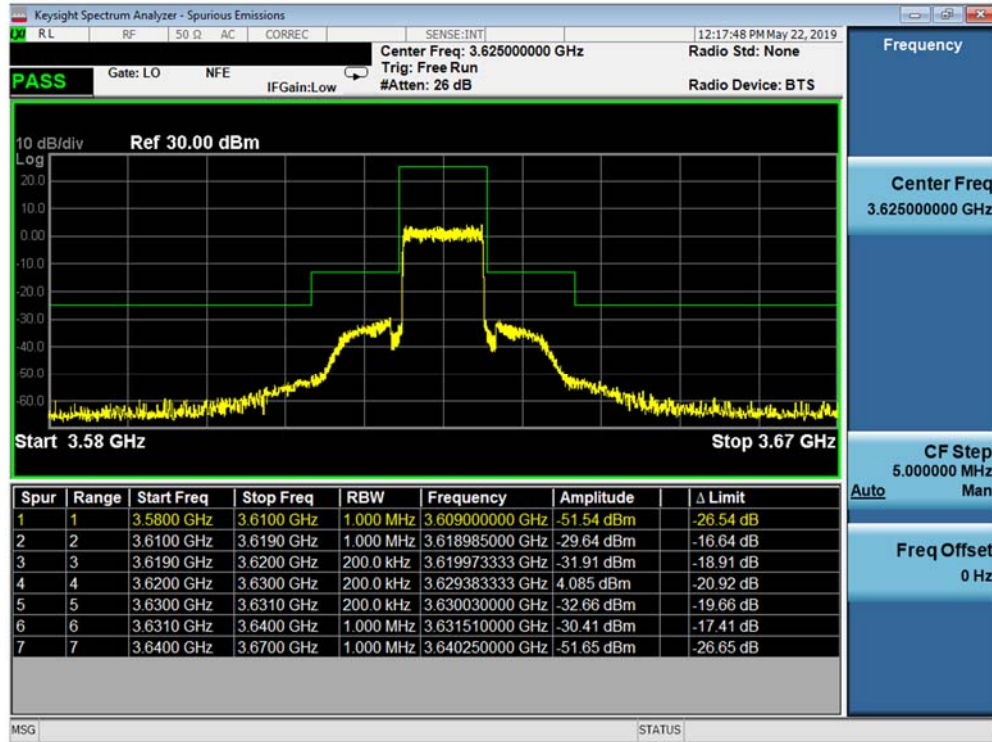
Plot 7-36. Mid Channel Edge Plot (Band 48 - 10.0MHz QPSK - Full RB Configuration)
