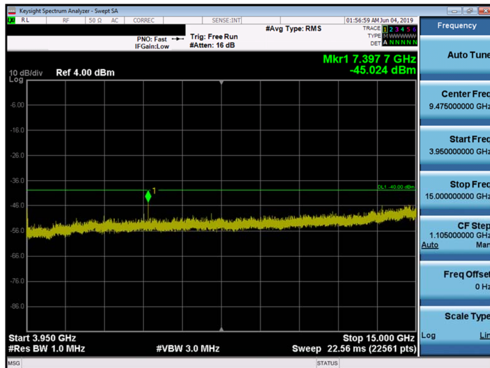
Plot 7-30. Conducted Spurious Plot (Band 48 - 20.0MHz QPSK - RB Size 1, RB Offset 99 - High Channel)
