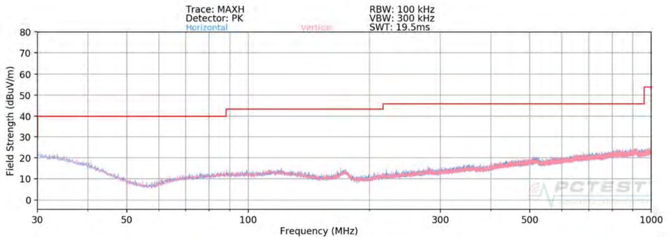
Plot 7-425. Radiated Spurious Plot below 1GHz MIMO (802.11ax – 242 Tones – U3 Ch. 157)
