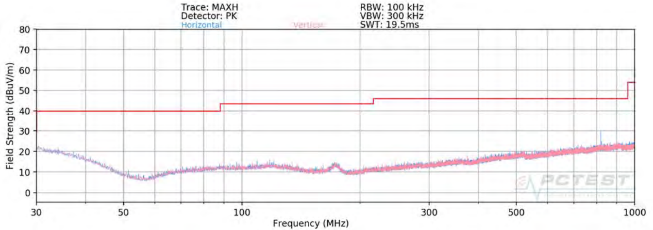
Plot 7-424. Radiated Spurious Plot below 1GHz MIMO (802.11ax – 26 Tones – U3 Ch. 157)
