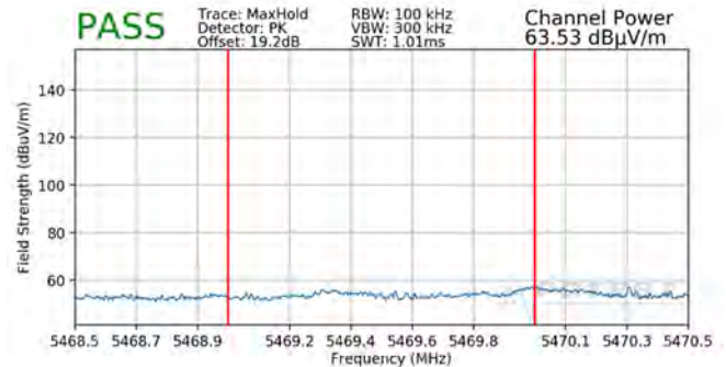
Plot 7-415. Radiated Lower Band Edge Plot MIMO (Peak – UNII Band 2C – 484 Tones)
