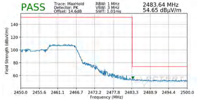
Plot 7-112. Radiated Restricted Upper Band Edge Measurement SISO ANT2 (Peak – 106 Tones)
