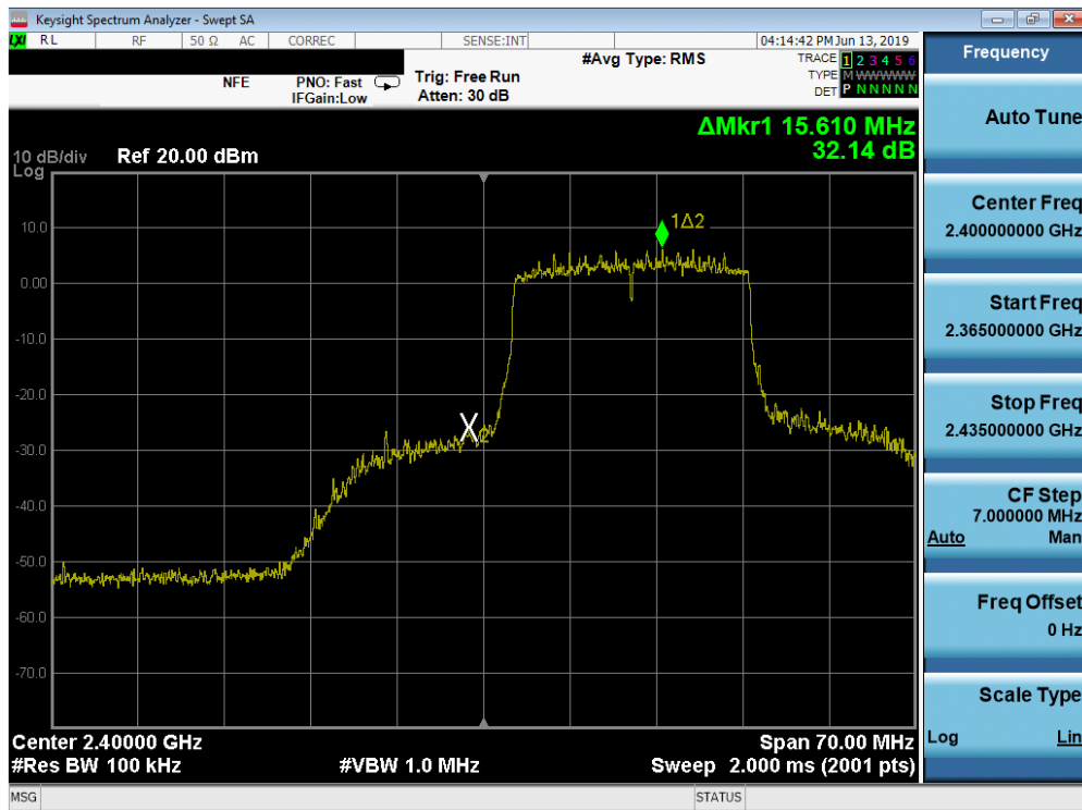
Plot 7-43. Band Edge Plot SISO ANT2 (802.11ax OFDMA – 242 Tones – Ch. 1)
