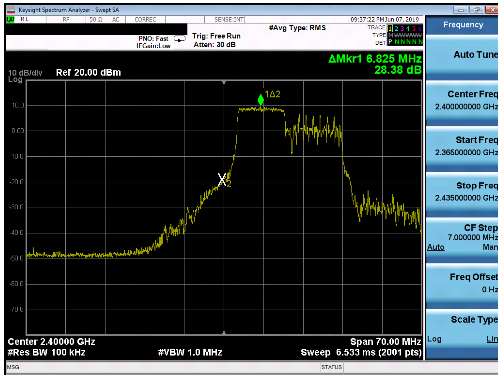
Plot 7-37. Band Edge Plot SISO ANT1 (802.11ax OFDMA – 106 Tones – Ch. 1)
