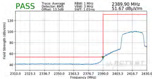
Plot 7-101. Radiated Restricted Lower Band Edge Measurement SISO ANT1 (Average – 242 Tones)
