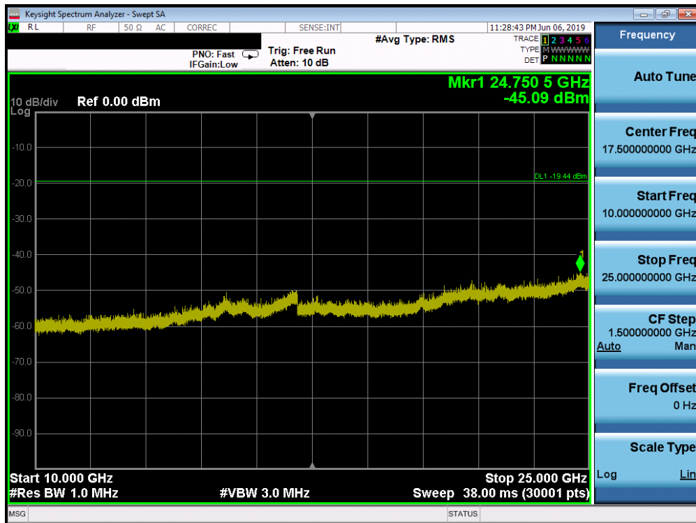
Plot 7-48. Conducted Spurious Plot SISO ANT1 (802.11ax OFDMA – 26 Tones – Ch. 6)
