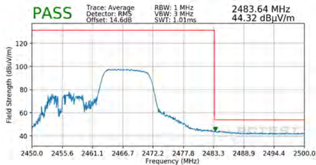
Plot 7-113. Radiated Restricted Upper Band Edge Measurement SISO ANT2 (Average – 106 Tones)
