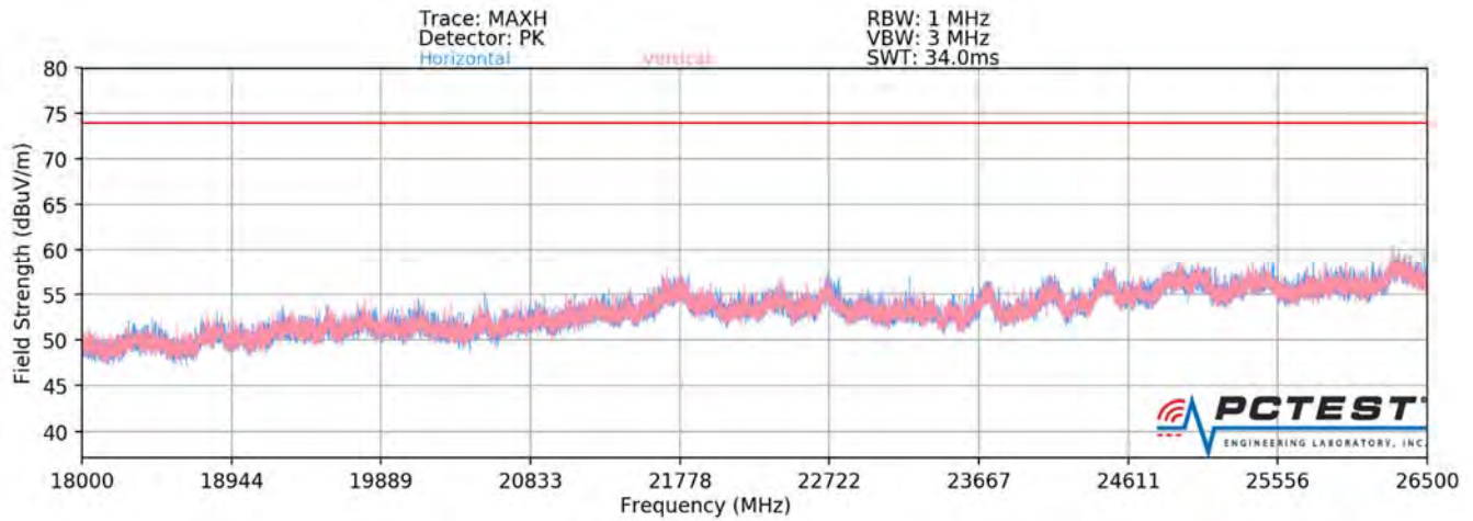
Plot 7-75. Radiated Spurious Plot above 18GHz SISO ANT1 (802.11ax OFDMA – 26 Tones)
