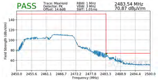
Plot 7-98. Radiated Restricted Upper Band Edge Measurement SISO ANT1 (Peak – 106 Tones)
