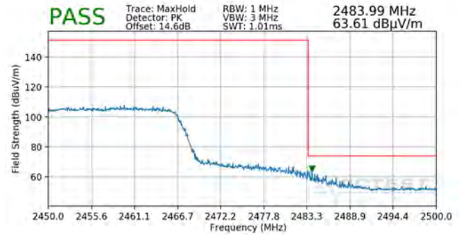
Plot 7-136. Radiated Restricted Upper Band Edge Measurement MIMO (Peak – 242 Tones)
