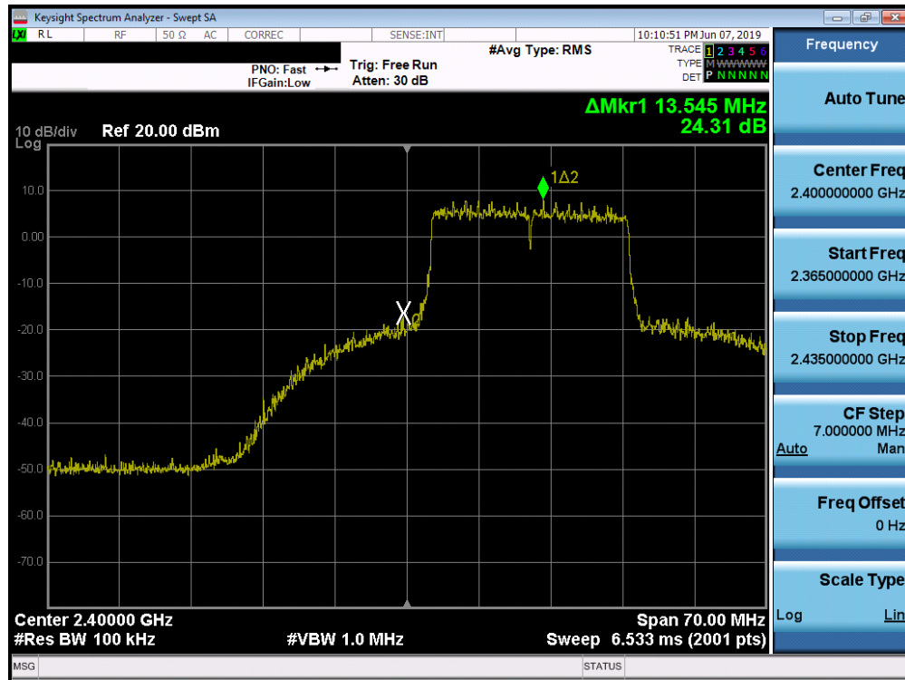
Plot 7-39. Band Edge Plot SISO ANT1 (802.11ax OFDMA – 242 Tones – Ch. 1)
