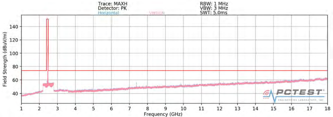
Plot 7-71. Radiated Spurious Plot above 1GHz SISO ANT1 (802.11ax OFDMA – 26 Tones – Ch. 11)
