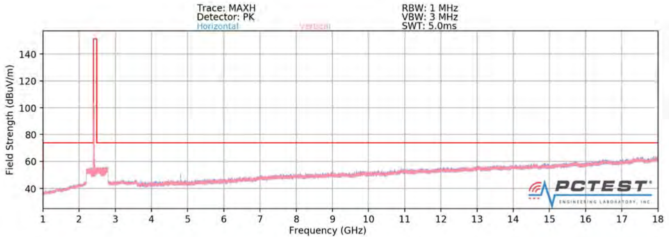
Plot 7-77. Radiated Spurious Plot above 1GHz SISO ANT2 (802.11ax OFDMA – 26 Tones – Ch. 1)
