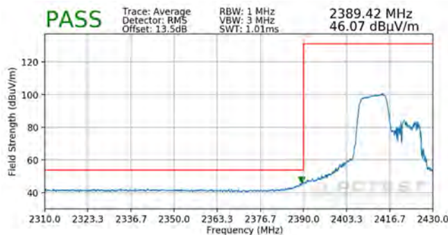
Plot 7-125. Radiated Restricted Lower Band Edge Measurement MIMO (Average – 106 Tones)
