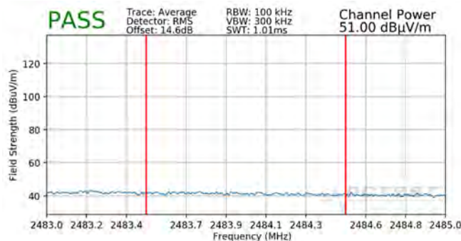
Plot 7-105. Radiated Restricted Upper Band Edge Measurement SISO ANT1 (Average – 242 Tones)
