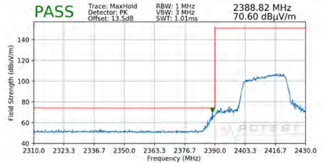
Plot 7-100. Radiated Restricted Lower Band Edge Measurement SISO ANT1 (Peak – 242 Tones)
