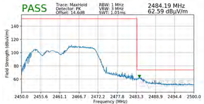
Plot 7-130. Radiated Restricted Upper Band Edge Measurement MIMO (Peak – 106 Tones)
