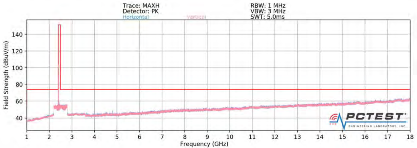
Plot 7-78. Radiated Spurious Plot above 1GHz SISO ANT2 (802.11ax OFDMA – 26 Tones – Ch. 6)
