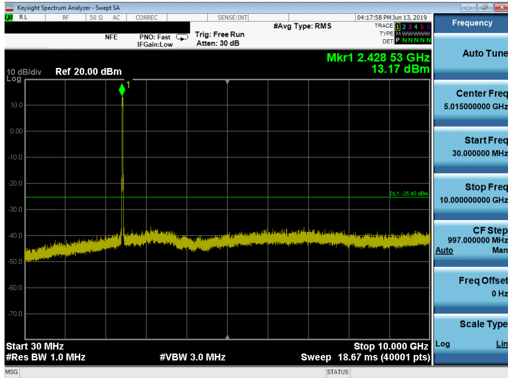
Plot 7-65. Conducted Spurious Plot SISO ANT2 (802.11ax OFDMA – 242 Tones – Ch. 6)
