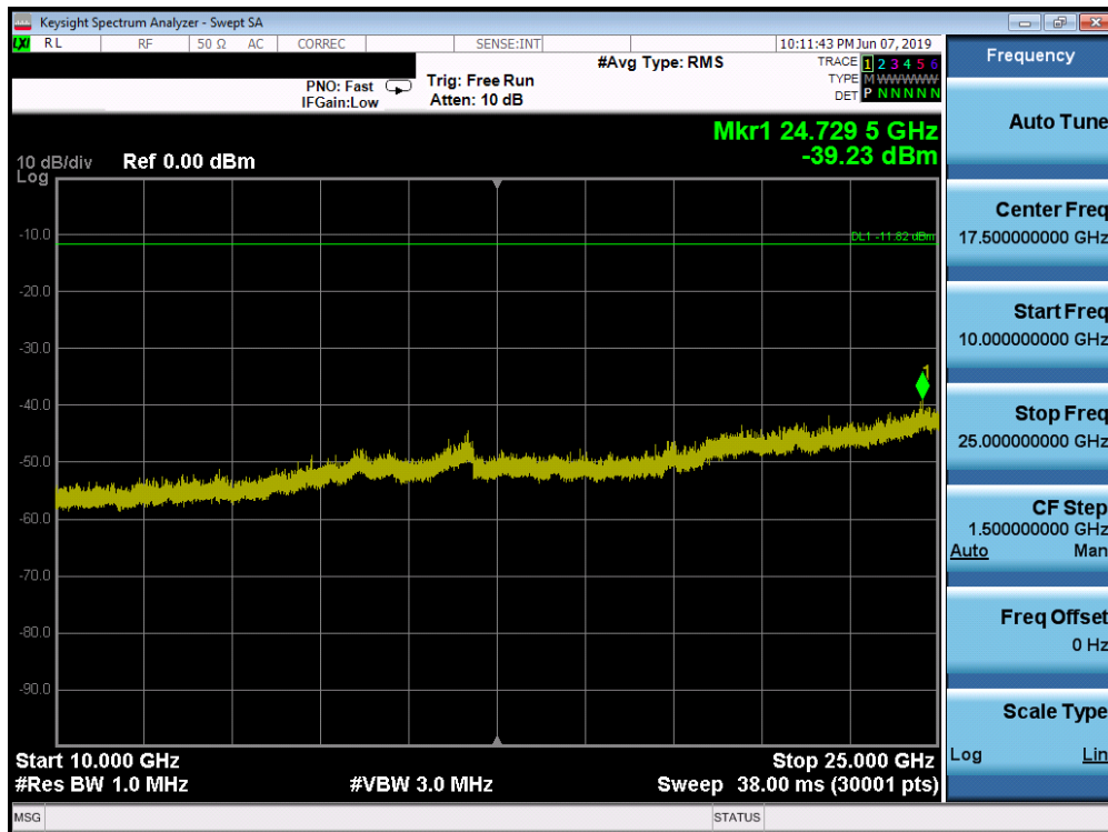
Plot 7-52. Conducted Spurious Plot SISO ANT1 (802.11ax OFDMA – 242 Tones – Ch. 1)
