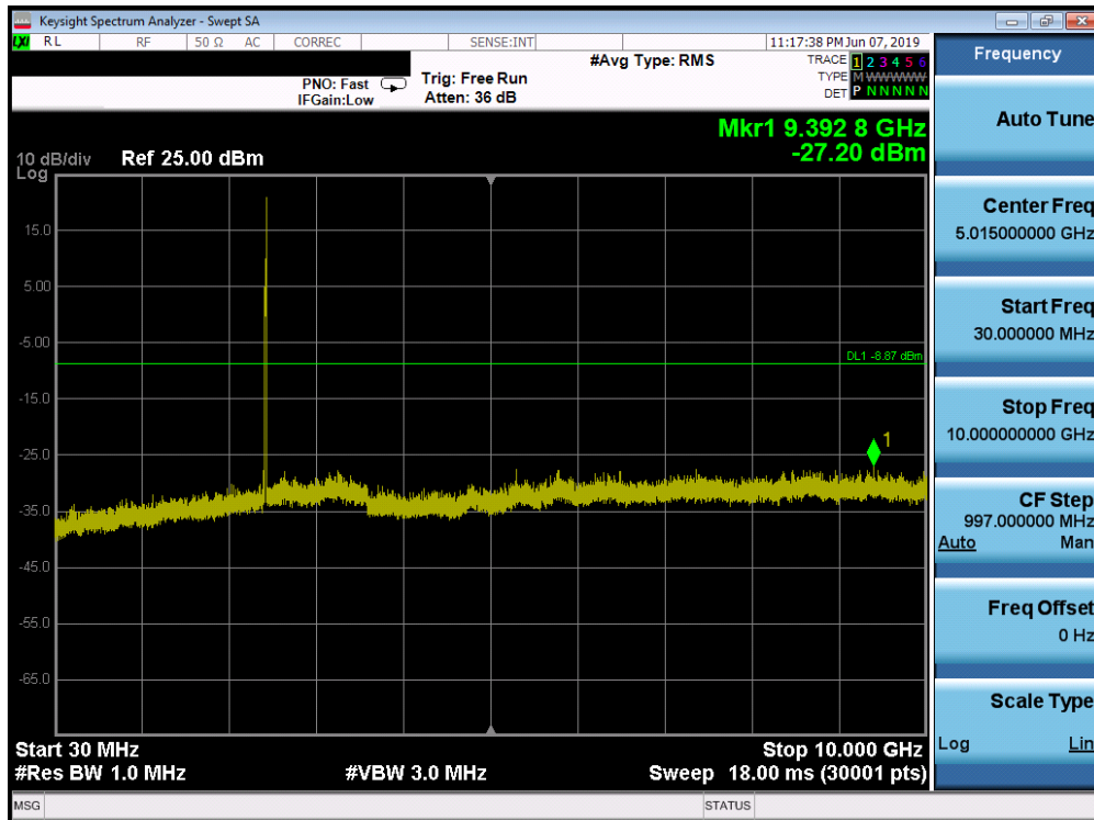
Plot 7-59. Conducted Spurious Plot SISO ANT2 (802.11ax OFDMA – 26 Tones – Ch. 6)
