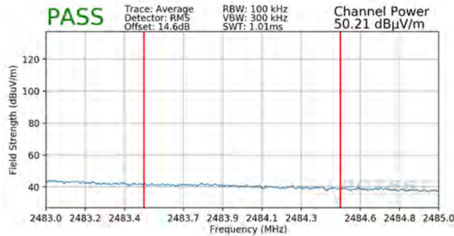
Plot 7-103. Radiated Restricted Upper Band Edge Measurement SISO ANT1 (Average – 242 Tones)
