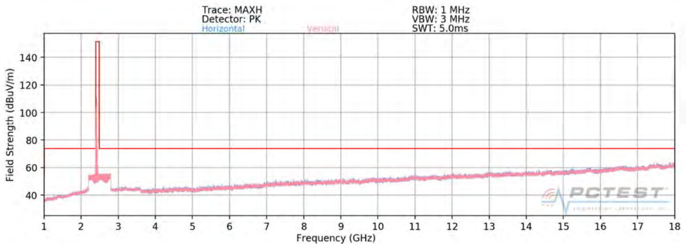
Plot 7-72. Radiated Spurious Plot above 1GHz SISO ANT1 (802.11ax OFDMA – 242 Tones – Ch. 1)
