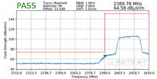
Plot 7-132. Radiated Restricted Lower Band Edge Measurement MIMO (Peak – 242 Tones)
