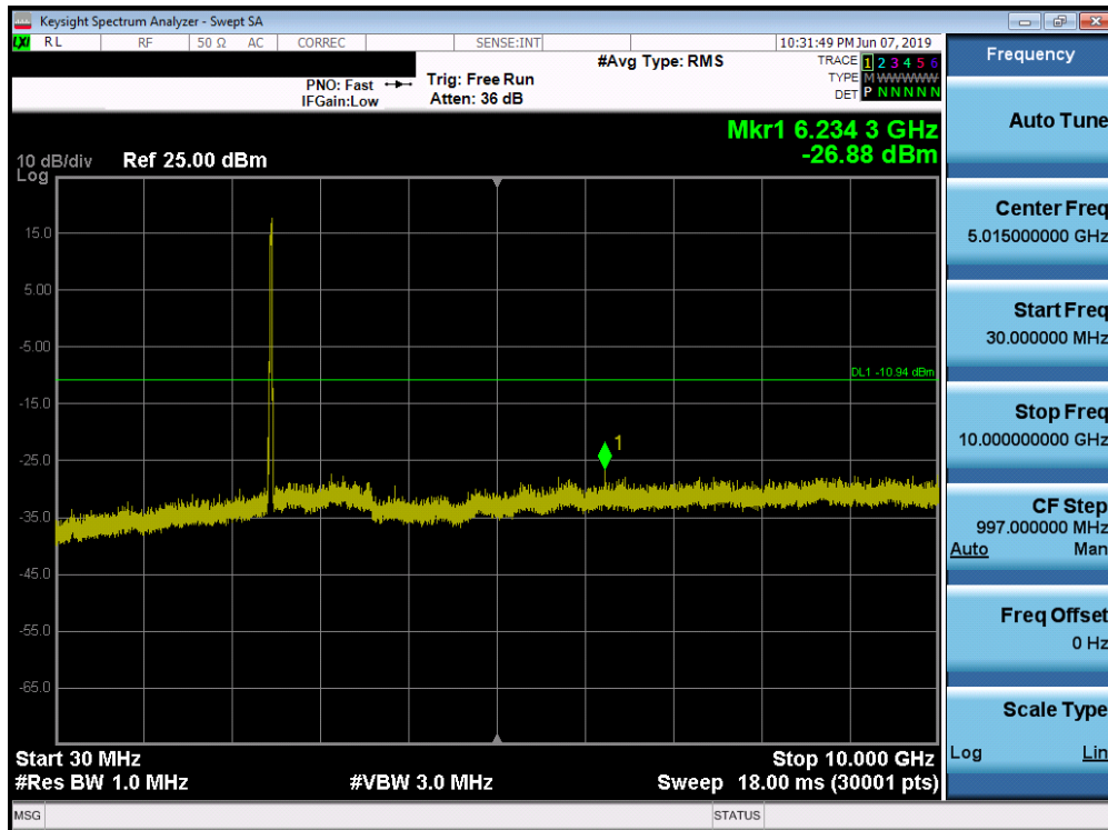
Plot 7-55. Conducted Spurious Plot SISO ANT1 (802.11ax OFDMA – 242 Tones – Ch. 11)
