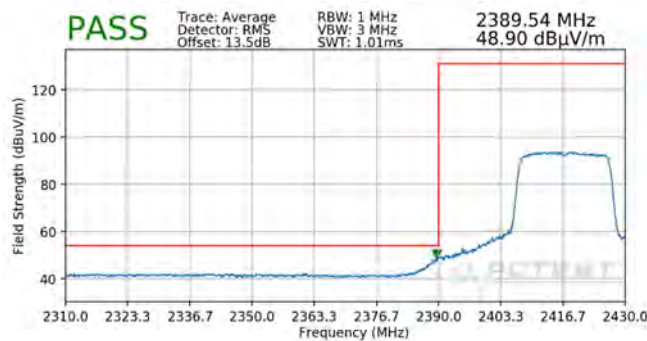
Plot 7-117. Radiated Restricted Lower Band Edge Measurement SISO ANT2 (Average – 242 Tones)
