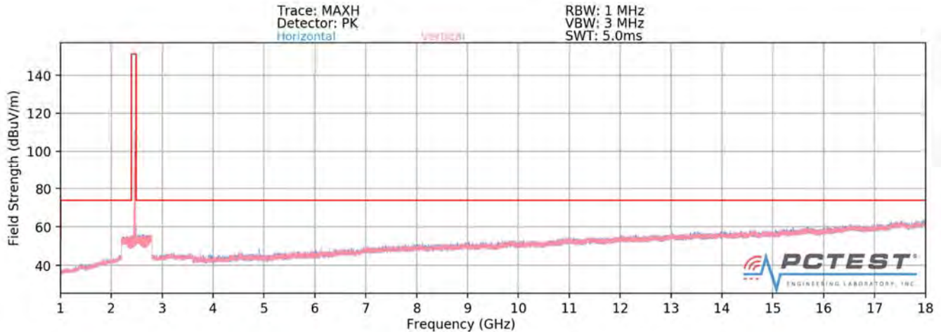
Plot 7-79. Radiated Spurious Plot above 1GHz SISO ANT2 (802.11ax OFDMA – 26 Tones – Ch. 11)
