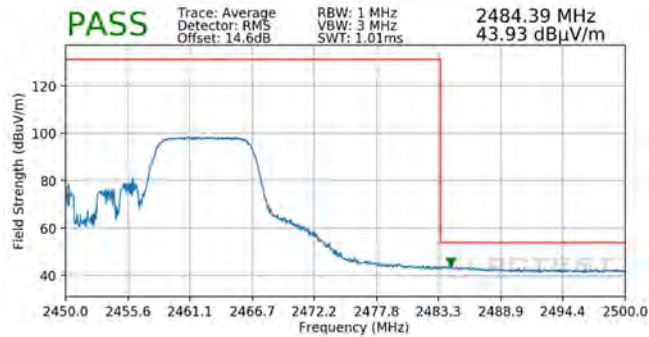
Plot 7-111. Radiated Restricted Upper Band Edge Measurement SISO ANT2 (Average – 106 Tones)
