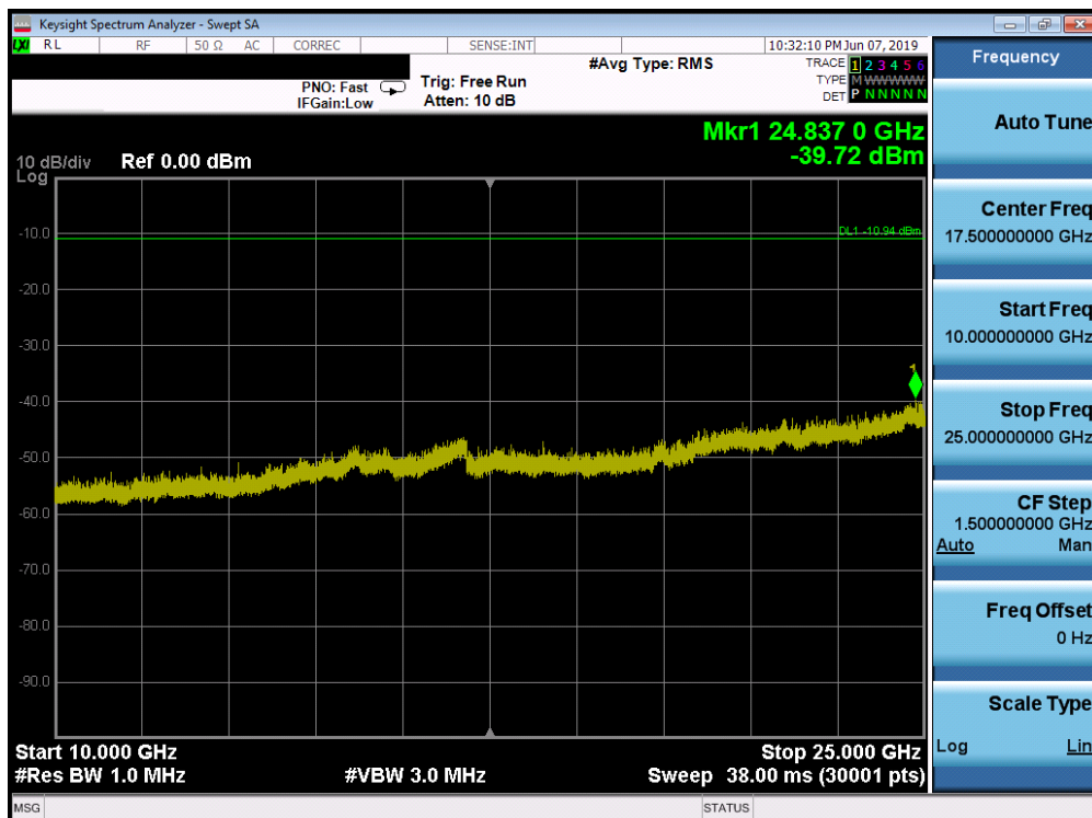
Plot 7-56. Conducted Spurious Plot SISO ANT1 (802.11ax OFDMA – 242 Tones – Ch. 11)
