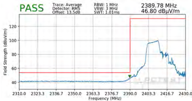
Plot 7-93. Radiated Restricted Lower Band Edge Measurement SISO ANT1 (Average – 106 Tones)
