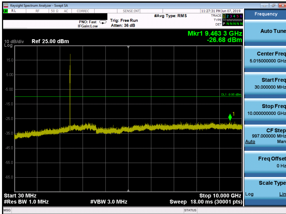
Plot 7-61. Conducted Spurious Plot SISO ANT2 (802.11ax OFDMA – 26 Tones – Ch. 11)
