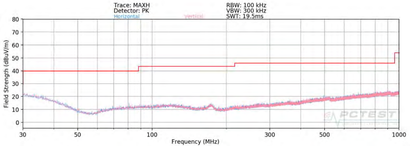
Plot 7-139. Radiated Spurious Plot below 1GHz MIMO (26 Tones)
