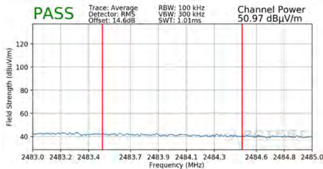
Plot 7-137. Radiated Restricted Upper Band Edge Measurement MIMO (Average – 242 Tones)
