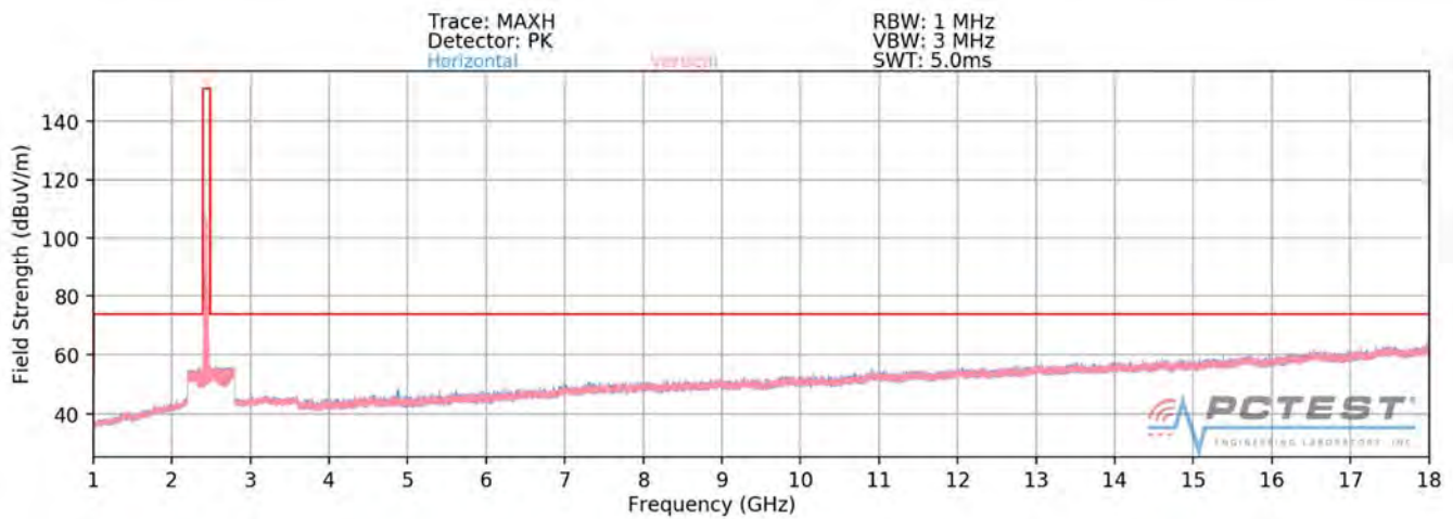
Plot 7-73. Radiated Spurious Plot above 1GHz SISO ANT1 (802.11ax OFDMA – 242 Tones – Ch. 6)
