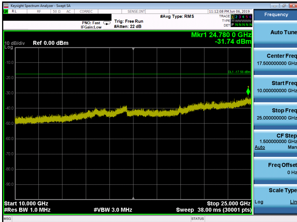
Plot 7-46. Conducted Spurious Plot SISO ANT1 (802.11ax OFDMA – 26 Tones – Ch. 1)
