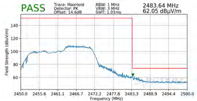
Plot 7-114. Radiated Restricted Upper Band Edge Measurement SISO ANT2 (Peak – 106 Tones)
