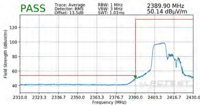
Plot 7-107. Radiated Restricted Lower Band Edge Measurement SISO ANT2 (Average – 106 Tones)
