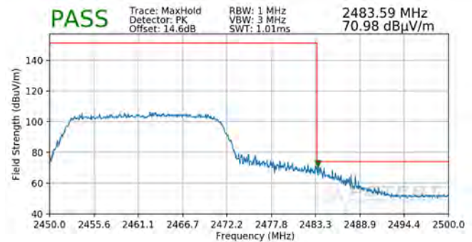
Plot 7-122. Radiated Restricted Upper Band Edge Measurement SISO ANT2 (Peak – 242 Tones)
