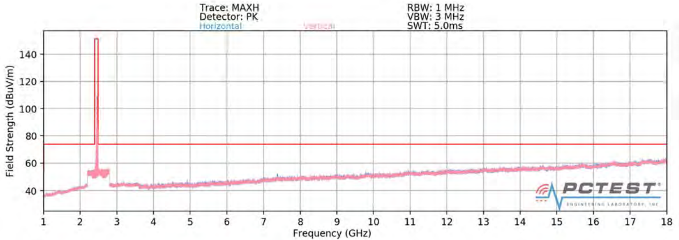
Plot 7-74. Radiated Spurious Plot above 1GHz SISO ANT1 (802.11ax OFDMA – 242 Tones – Ch. 11)
