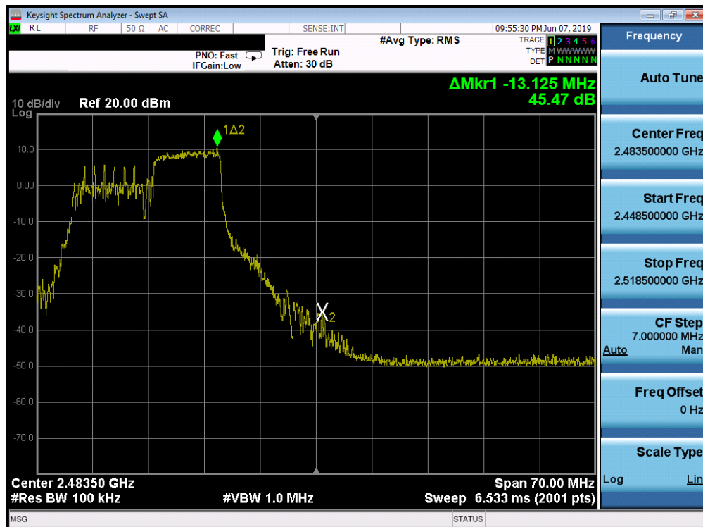
Plot 7-38. Band Edge Plot SISO ANT1 (802.11ax OFDMA – 106 Tones – Ch. 11)
