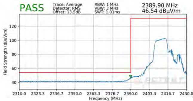
Plot 7-95. Radiated Restricted Lower Band Edge Measurement SISO ANT1 (Average – 106 Tones)
