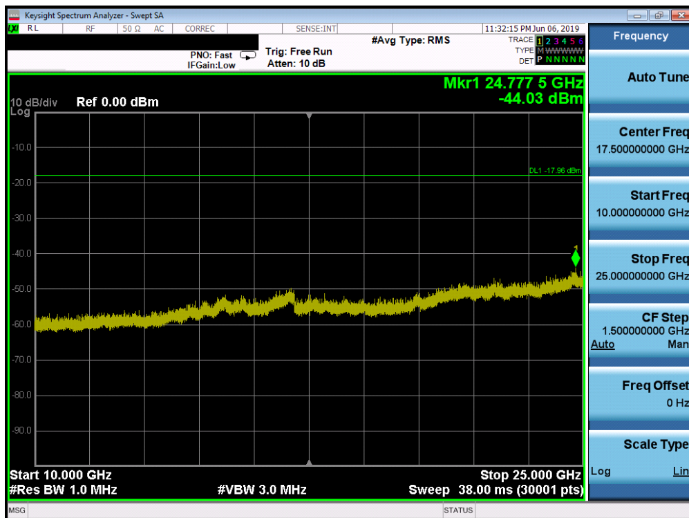
Plot 7-50. Conducted Spurious Plot SISO ANT1 (802.11ax OFDMA – 26 Tones – Ch. 11)
