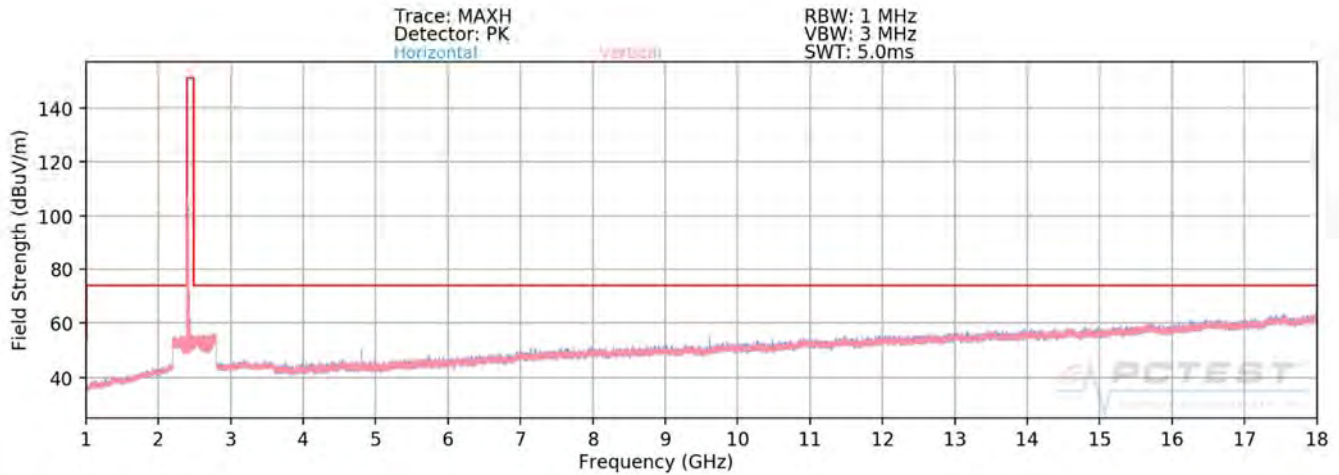
Plot 7-69. Radiated Spurious Plot above 1GHz SISO ANT1 (802.11ax OFDMA – 26 Tones – Ch. 1)
