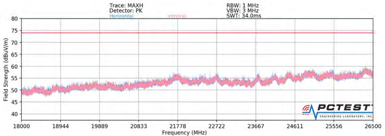
Plot 7-76. Radiated Spurious Plot above 18GHz SISO ANT1 (802.11ax OFDMA – 242 Tones)
