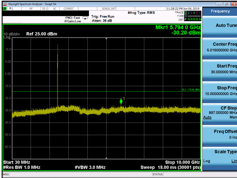
Plot 7-47. Conducted Spurious Plot SISO ANT1 (802.11ax OFDMA – 26 Tones – Ch. 6)
