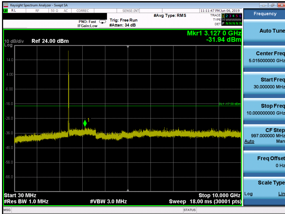
Plot 7-45. Conducted Spurious Plot SISO ANT1 (802.11ax OFDMA – 26 Tones – Ch. 1)
