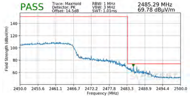
Plot 7-104. Radiated Restricted Upper Band Edge Measurement SISO ANT1 (Peak – 242 Tones)
