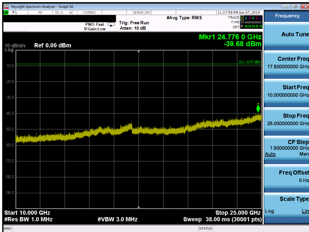
Plot 7-60. Conducted Spurious Plot SISO ANT2 (802.11ax OFDMA – 26 Tones – Ch. 6)
