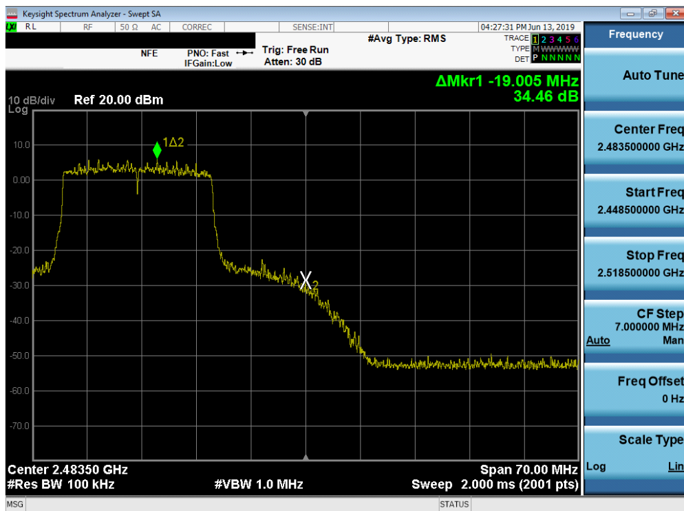
Plot 7-44. Band Edge Plot SISO ANT2 (802.11ax OFDMA – 242 Tones – Ch. 11)
