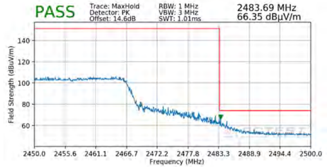
Plot 7-120. Radiated Restricted Upper Band Edge Measurement SISO ANT2 (Peak – 242 Tones)
