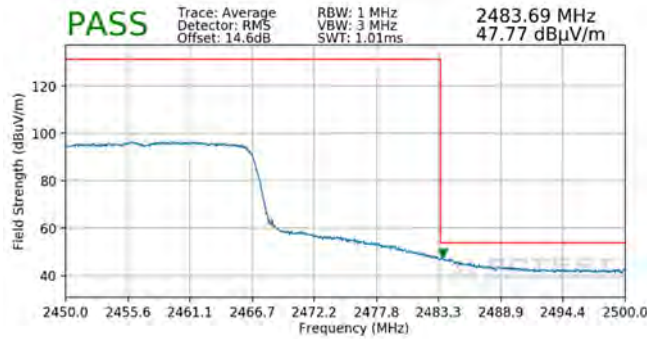
Plot 7-135. Radiated Restricted Upper Band Edge Measurement MIMO (Average – 242 Tones)
