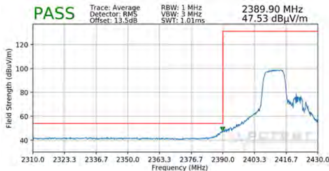
Plot 7-109. Radiated Restricted Lower Band Edge Measurement SISO ANT2 (Average – 106 Tones)
