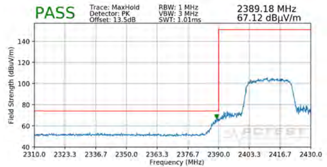
Plot 7-116. Radiated Restricted Lower Band Edge Measurement SISO ANT2 (Peak – 242 Tones)
