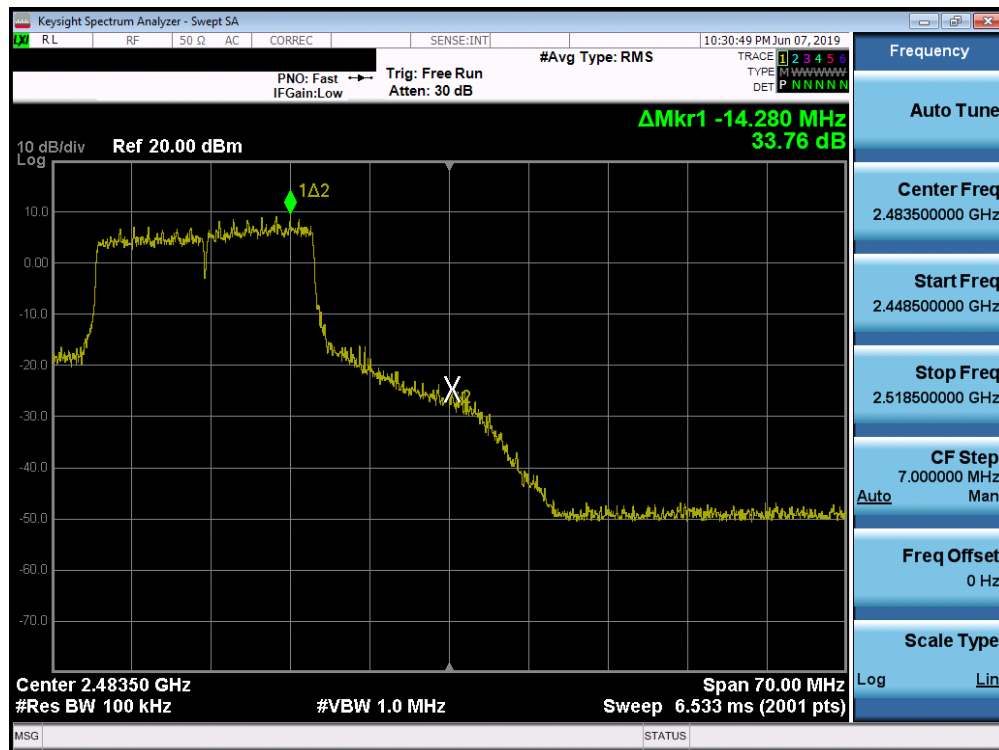
Plot 7-40. Band Edge Plot SISO ANT1 (802.11ax OFDMA – 242 Tones – Ch. 11)
