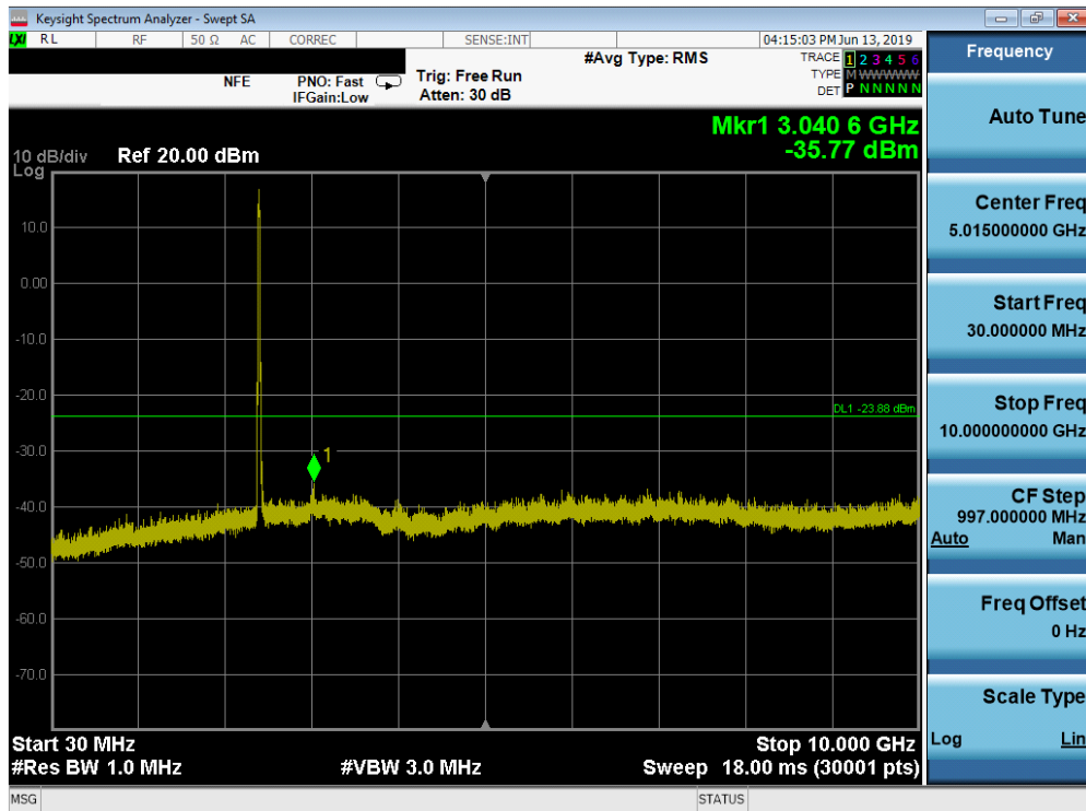
Plot 7-63. Conducted Spurious Plot SISO ANT2 (802.11ax OFDMA – 242 Tones – Ch. 1)
