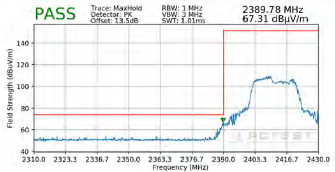
Plot 7-94. Radiated Restricted Lower Band Edge Measurement SISO ANT1 (Peak – 106 Tones)
