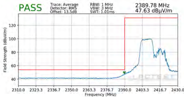
Plot 7-123. Radiated Restricted Lower Band Edge Measurement MIMO (Average – 106 Tones)
