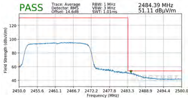
Plot 7-121. Radiated Restricted Upper Band Edge Measurement SISO ANT2 (Average – 242 Tones)
