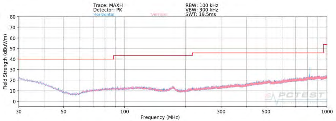
Plot 7-140. Radiated Spurious Plot below 1GHz MIMO (242 Tones)
