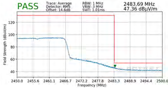
Plot 7-119. Radiated Restricted Upper Band Edge Measurement SISO ANT2 (Average – 242 Tones)
