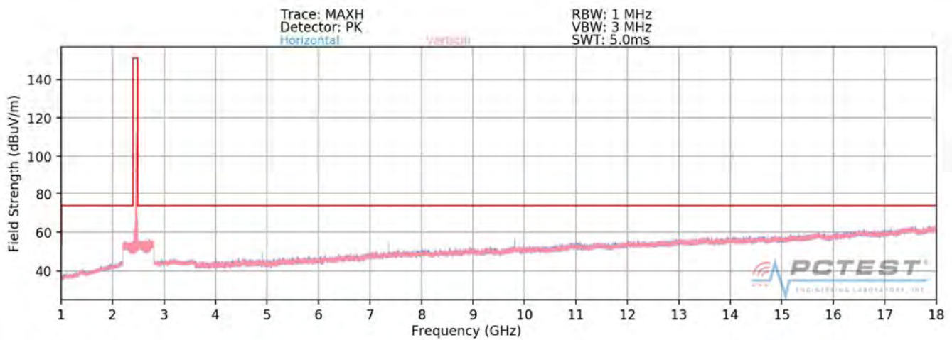
Plot 7-70. Radiated Spurious Plot above 1GHz SISO ANT1 (802.11ax OFDMA – 26 Tones – Ch. 6)
