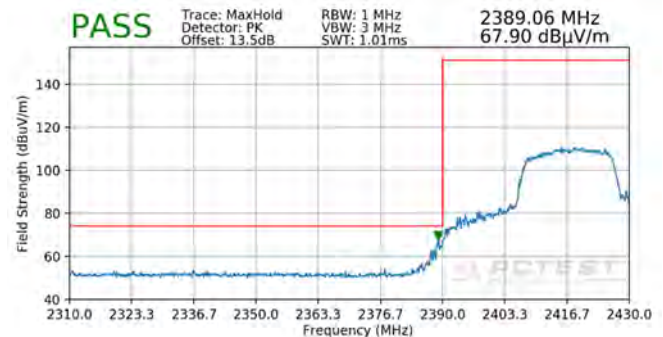
Plot 7-102. Radiated Restricted Lower Band Edge Measurement SISO ANT1 (Peak – 242 Tones)
