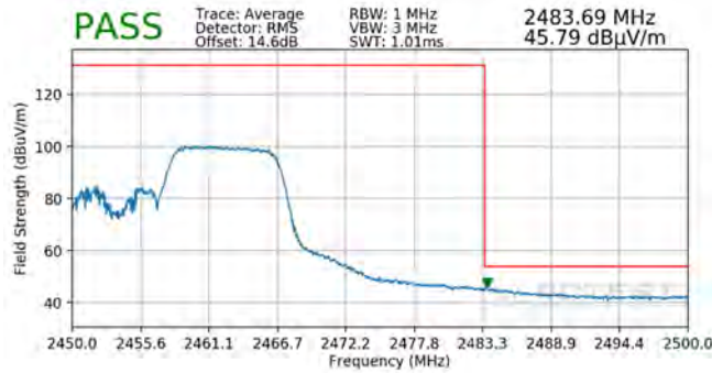
Plot 7-127. Radiated Restricted Upper Band Edge Measurement MIMO (Average – 106 Tones)
