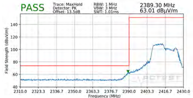
Plot 7-110. Radiated Restricted Lower Band Edge Measurement SISO ANT2 (Peak – 106 Tones)
