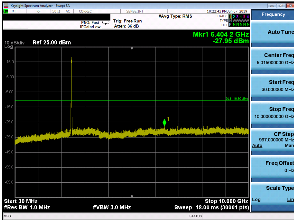
Plot 7-53. Conducted Spurious Plot SISO ANT1 (802.11ax OFDMA – 242 Tones – Ch. 6)
