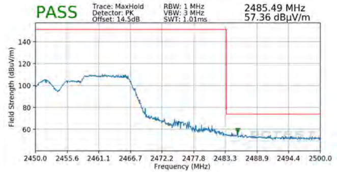
Plot 7-128. Radiated Restricted Upper Band Edge Measurement MIMO (Peak – 106 Tones)
