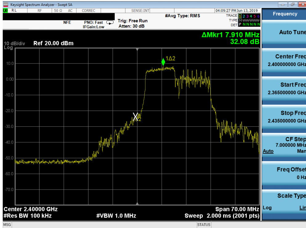
Plot 7-41. Band Edge Plot SISO ANT2 (802.11ax OFDMA – 106 Tones – Ch. 1)
