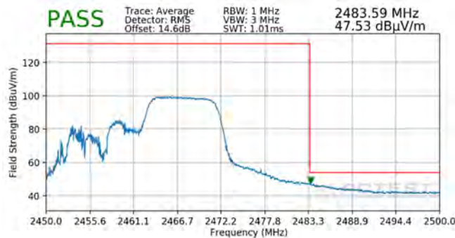
Plot 7-129. Radiated Restricted Upper Band Edge Measurement MIMO (Average – 106 Tones)
