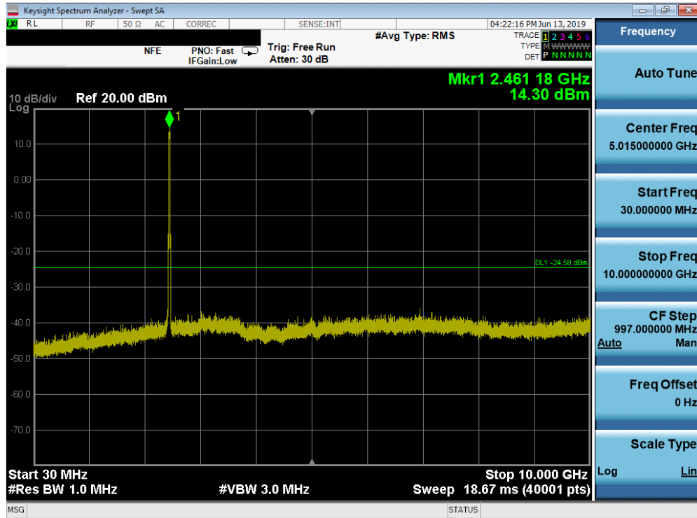
Plot 7-67. Conducted Spurious Plot SISO ANT2 (802.11ax OFDMA – 242 Tones – Ch. 11)
