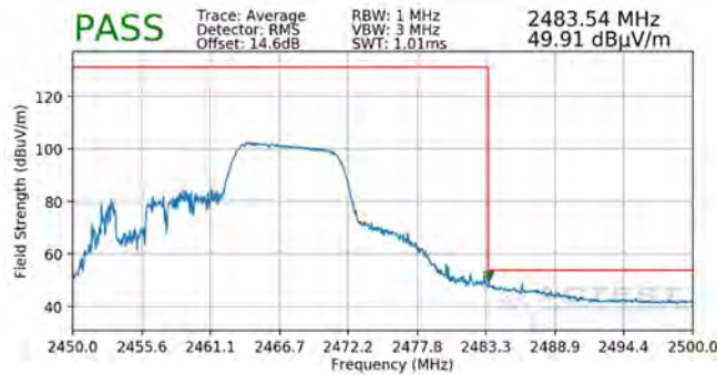
Plot 7-97. Radiated Restricted Upper Band Edge Measurement SISO ANT1 (Average – 106 Tones)
