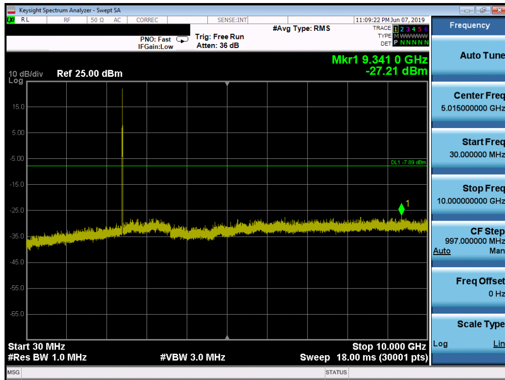
Plot 7-57. Conducted Spurious Plot SISO ANT2 (802.11ax OFDMA - 26 Tones - Ch. 1)
