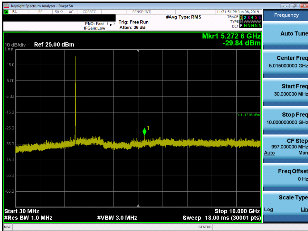
Plot 7-49. Conducted Spurious Plot SISO ANT1 (802.11ax OFDMA – 26 Tones – Ch. 11)
