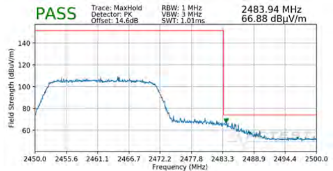
Plot 7-138. Radiated Restricted Upper Band Edge Measurement MIMO (Peak – 242 Tones)
