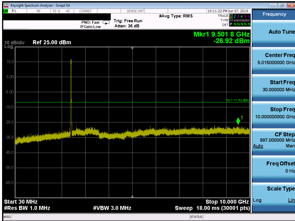
Plot 7-51. Conducted Spurious Plot SISO ANT1 (802.11ax OFDMA – 242 Tones – Ch. 1)
