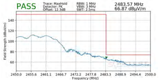
Plot 7-140. Radiated Restricted Upper Band Edge Measurement CDD (Peak)
