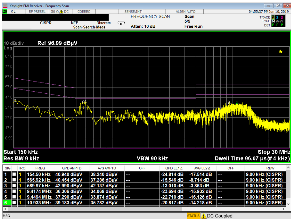
Plot 7-146. Line Conducted Plot with 802.11b (L1) with Travel Adapter
