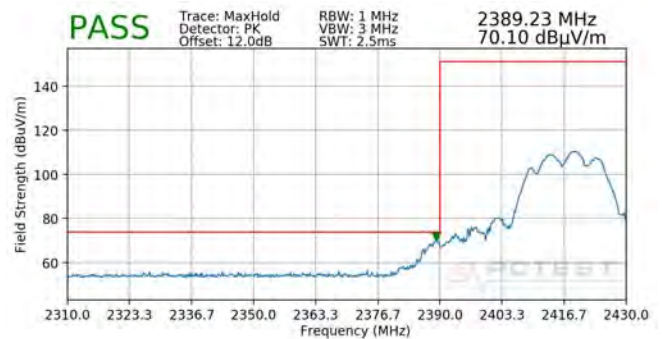
Plot 7-136. Radiated Restricted Lower Band Edge Measurement CDD (Peak)
