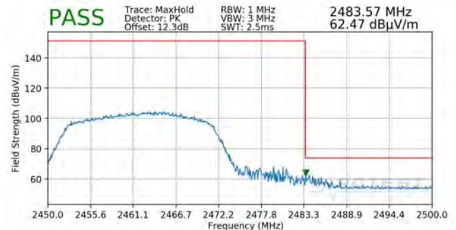
Plot 7-120. Radiated Restricted Upper Band Edge Measurement SISO ANT2 (Peak)
