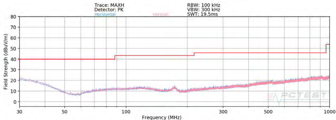
Plot 7-145. Radiated Spurious Plot below 1GHz MIMO
