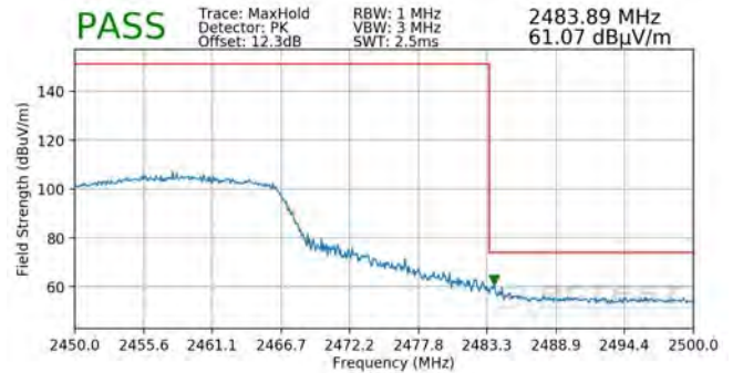
Plot 7-118. Radiated Restricted Upper Band Edge Measurement SISO ANT2 (Peak)
