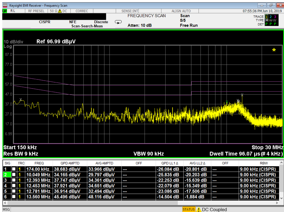
Plot 7-149. Line Conducted Plot with 802.11b (N) with Wireless Charging Pad
