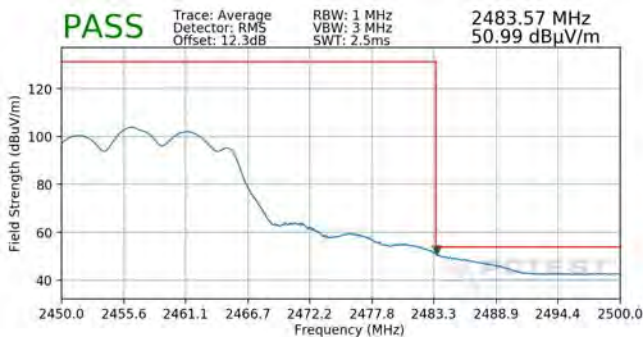
Plot 7-139. Radiated Restricted Upper Band Edge Measurement CDD (Average)
