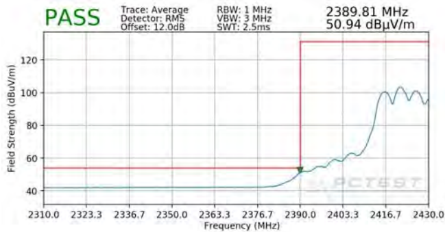
Plot 7-137. Radiated Restricted Lower Band Edge Measurement CDD (Average)
