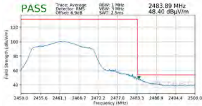
Plot 7-129. Radiated Restricted Upper Band Edge Measurement MIMO (Average)
