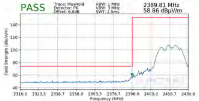
Plot 7-144. Radiated Restricted Band Edge Measurement CDD with WCP (Peak)
