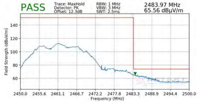
Plot 7-142. Radiated Restricted Upper Band Edge Measurement CDD (Peak)
