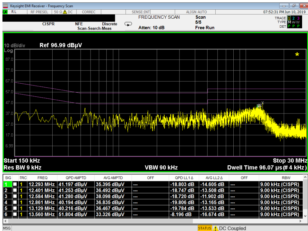
Plot 7-148. Line Conducted Plot with 802.11b (L1) with Wireless Charging Pad
