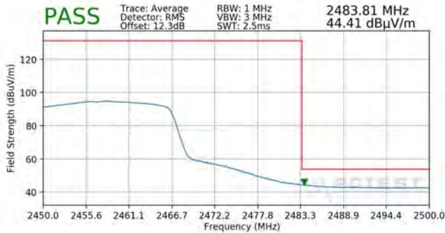
Plot 7-117. Radiated Restricted Upper Band Edge Measurement SISO ANT2 (Average)
