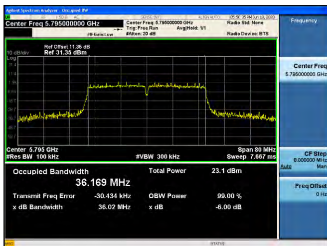
802.11ac(VHT40) (CH.159)
