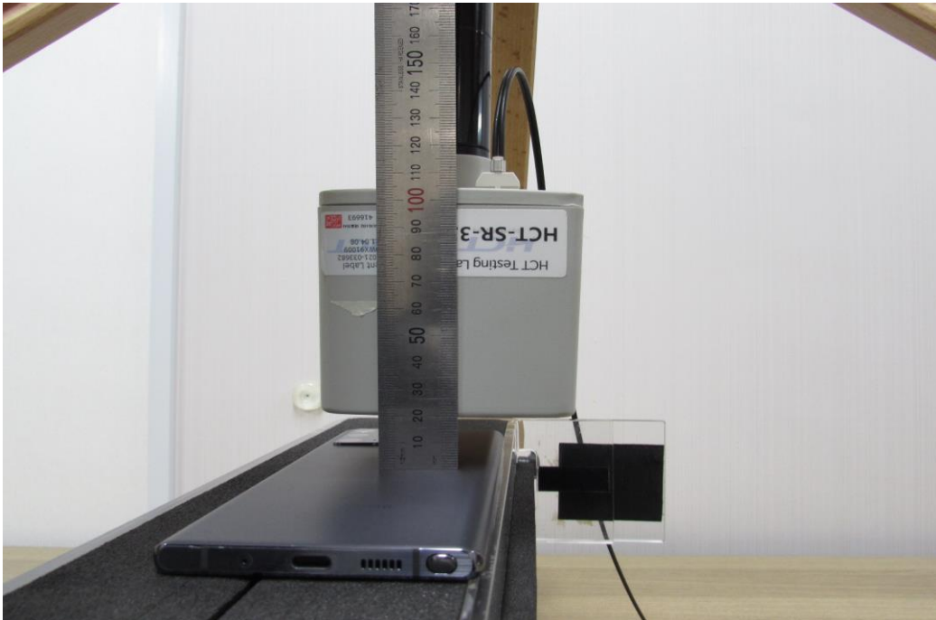
Distance from the rear side of the Device to the center of the Probe from 7.4 cm
