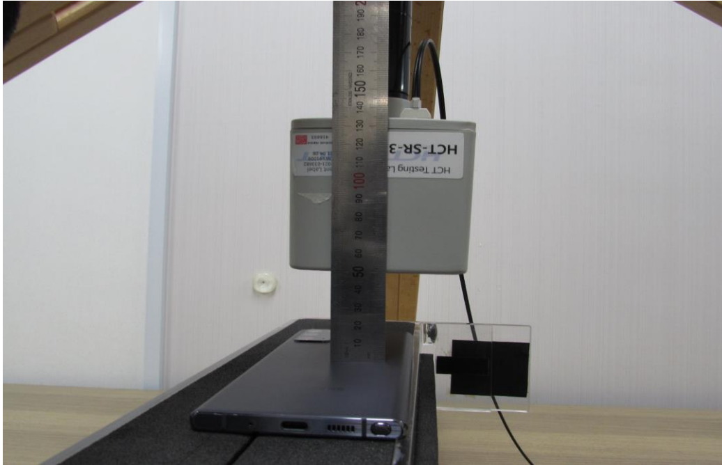
Distance from the rear side of the Device to the center of the Probe from 10.4 cm
