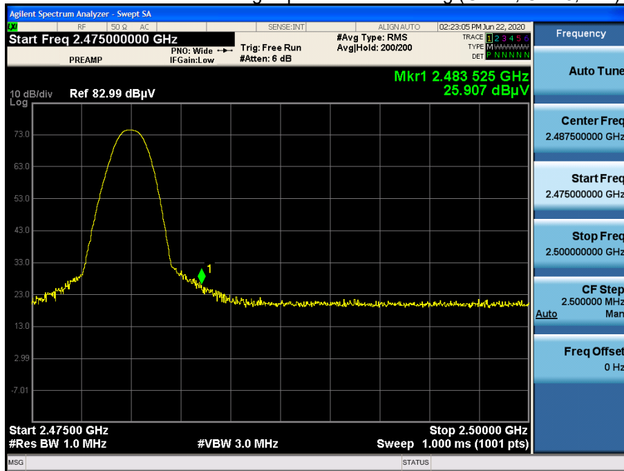
Radiated Restricted Band Edges plot – Peak Reading (GFSK, Ch.78, Z-V)
