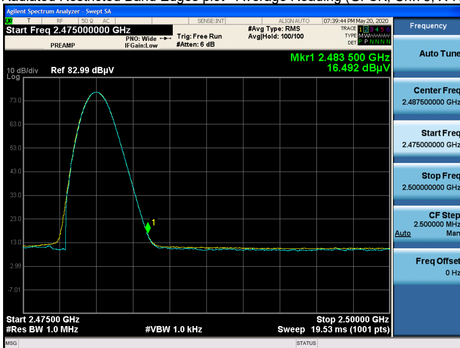
Radiated Restricted Band Edges plot –Average Reading (GFSK, Ch.78, X-H)
