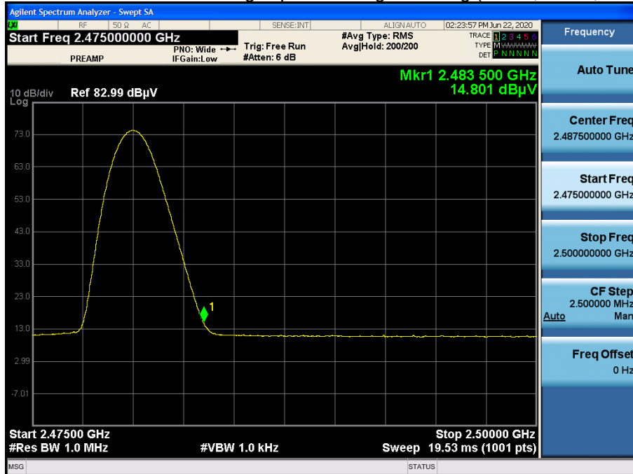
Radiated Restricted Band Edges plot –Average Reading (GFSK, Ch.78, Z-V)
