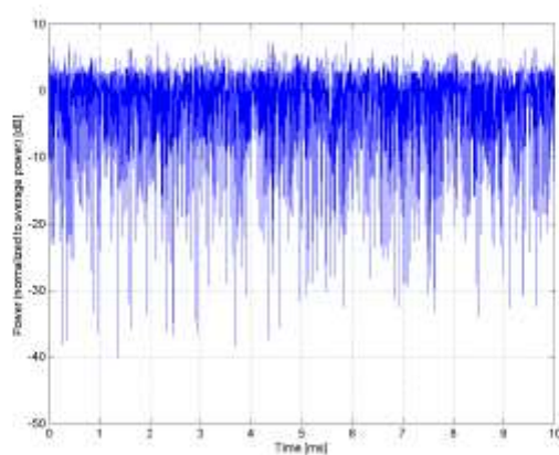
Time Domain
