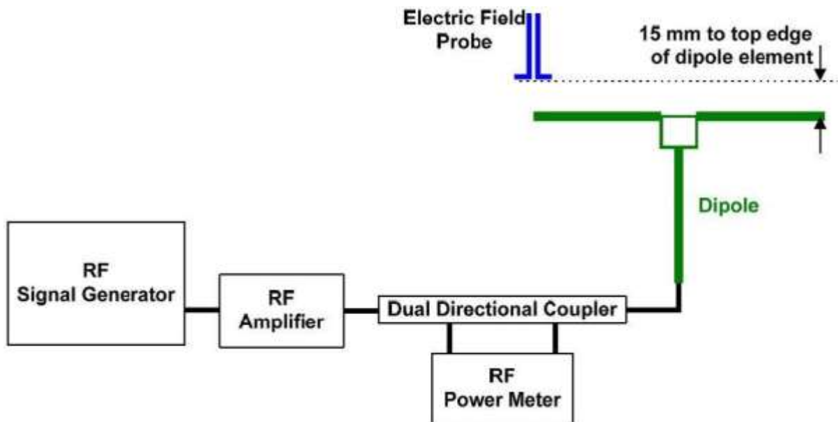
Setup diagram
