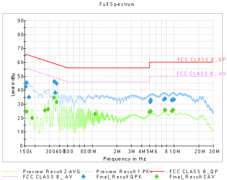
Figure 7: Conducted Emission (150 kHz to 30 MHz), [EUT+TA] Video+Audio, Line(L1)
