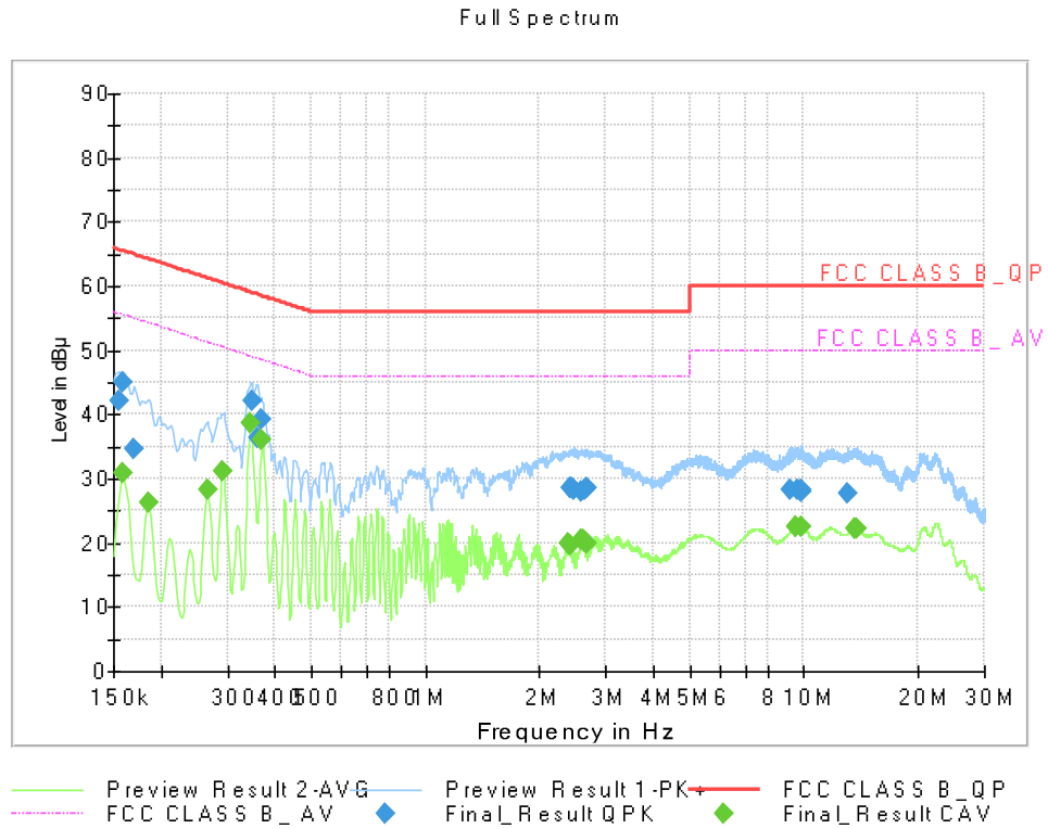
Figure 6: Conducted Emission (150 kHz to 30 MHz), [EUT+TA] LTE B26 Idle(Middle ch)+Rear Camera, Line(N)
