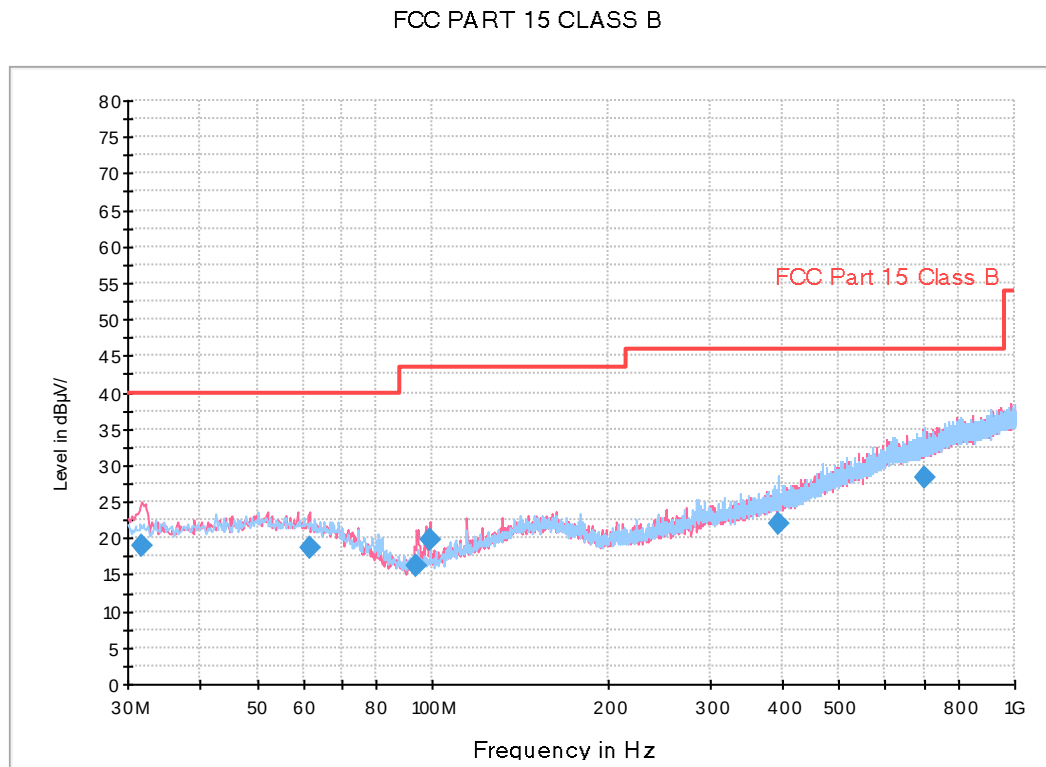
Figure 13: Radiated Emission (30 MHz to 1 GHz), [EUT+Earphone] Video+Audio
