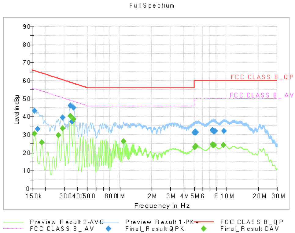
Figure 3: Conducted Emission (150 kHz to 30 MHz), [EUT+TA] LTE B5 Idle(Middle ch)+Front Camera, Line(L1)
