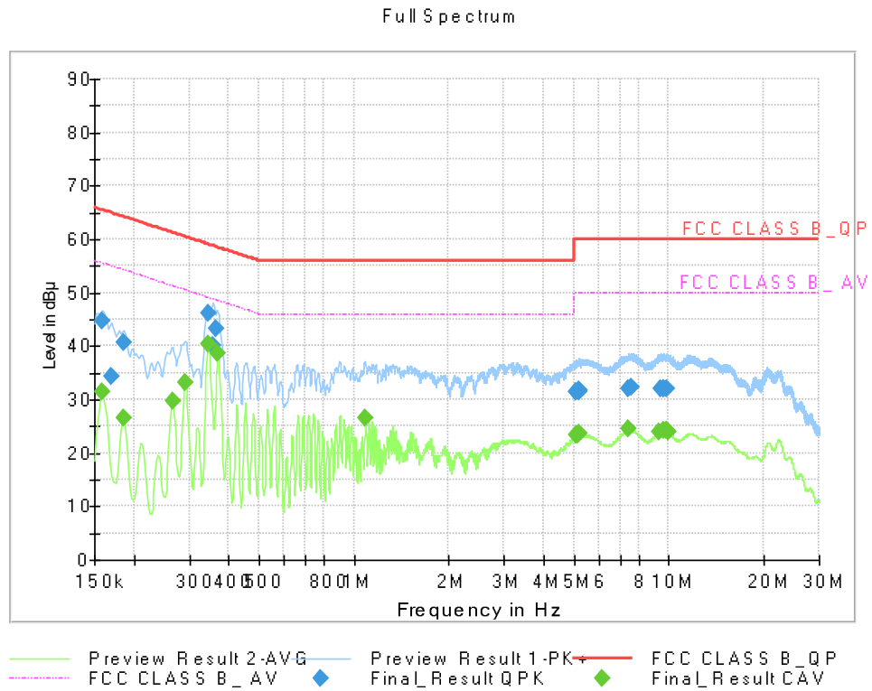
Figure 5: Conducted Emission (150 kHz to 30 MHz), [EUT+TA] LTE B26 Idle(Middle ch)+Rear Camera, Line(L1)
