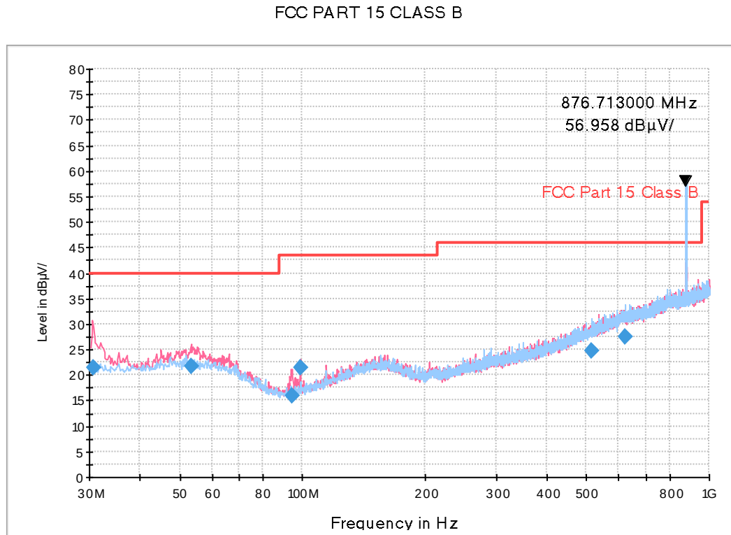
Figure 11: Radiated Emission (30 MHz to 1 GHz), [EUT+TA] LTE B26 Idle(Middle ch)+Rear Camera
