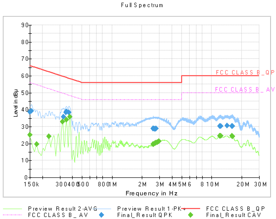
Figure 4: Conducted Emission (150 kHz to 30 MHz), [EUT+TA] LTE B5 Idle(Middle ch)+Front Camera, Line(N)
