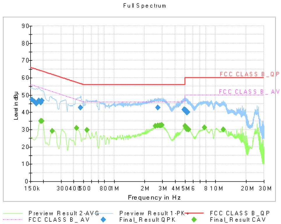
Figure 1: Conducted Emission (150 kHz to 30 MHz), [EUT+PC] Data Communication mode (Internal), Line(L1)
