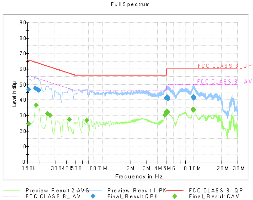
Figure 2: Conducted Emission (150 kHz to 30 MHz), [EUT+PC] Data Communication mode (Internal), Line(N)
