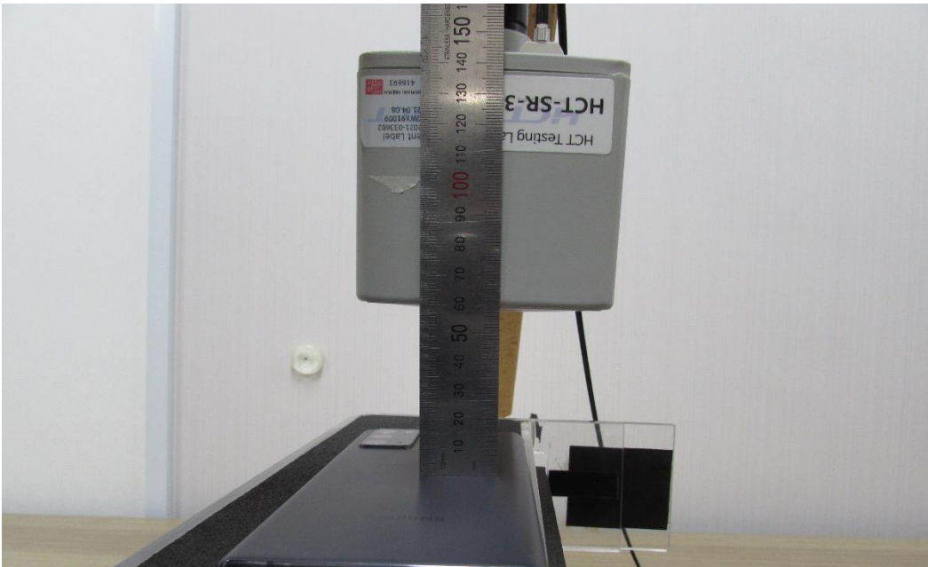
Distance from the rear side of the Device to the center of the Probe from 11.4 cm
