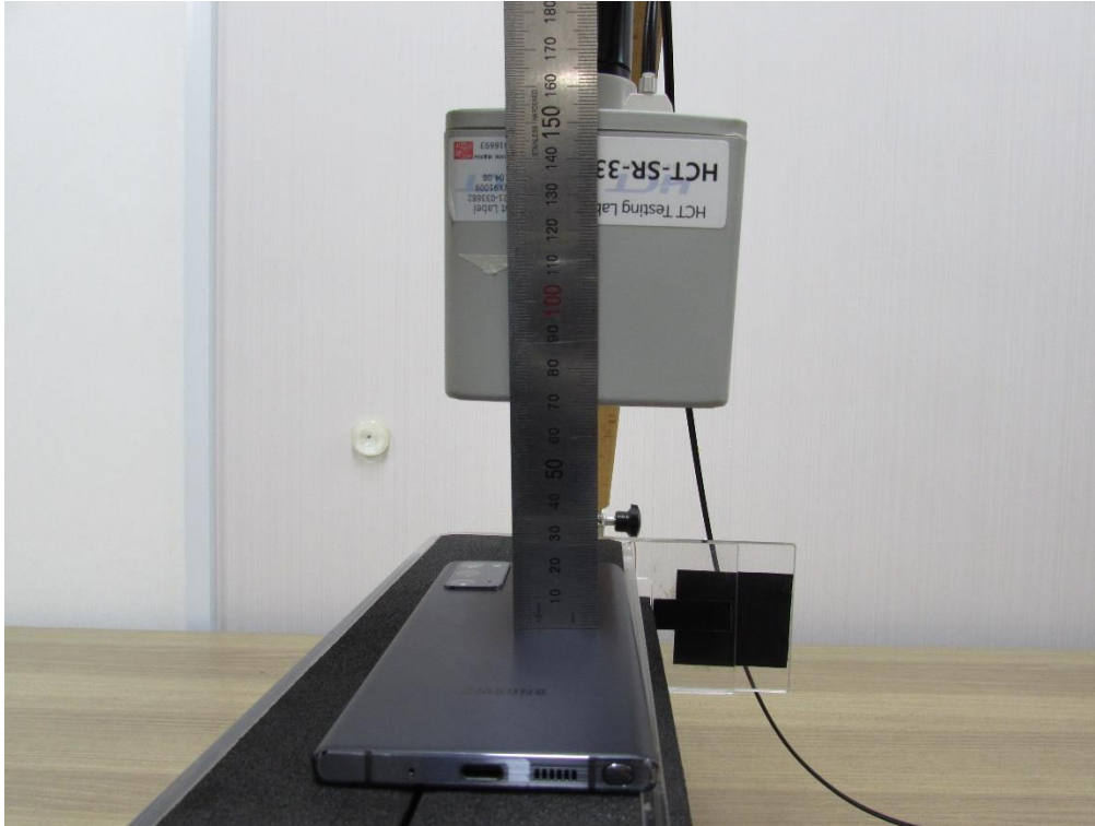
Distance from the rear side of the Device to the center of the Probe from 13.4 cm
