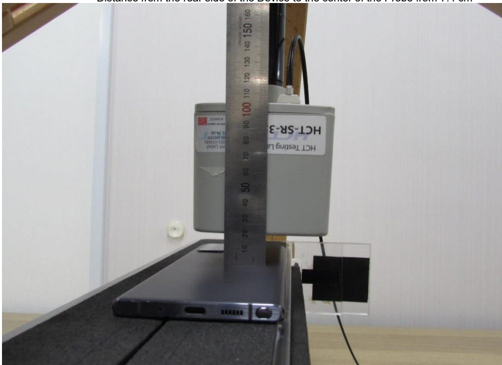
Distance from the rear side of the Device to the center of the Probe from 7.4 cm
