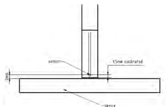
Figure 2-1 EUmWV3 Probe
