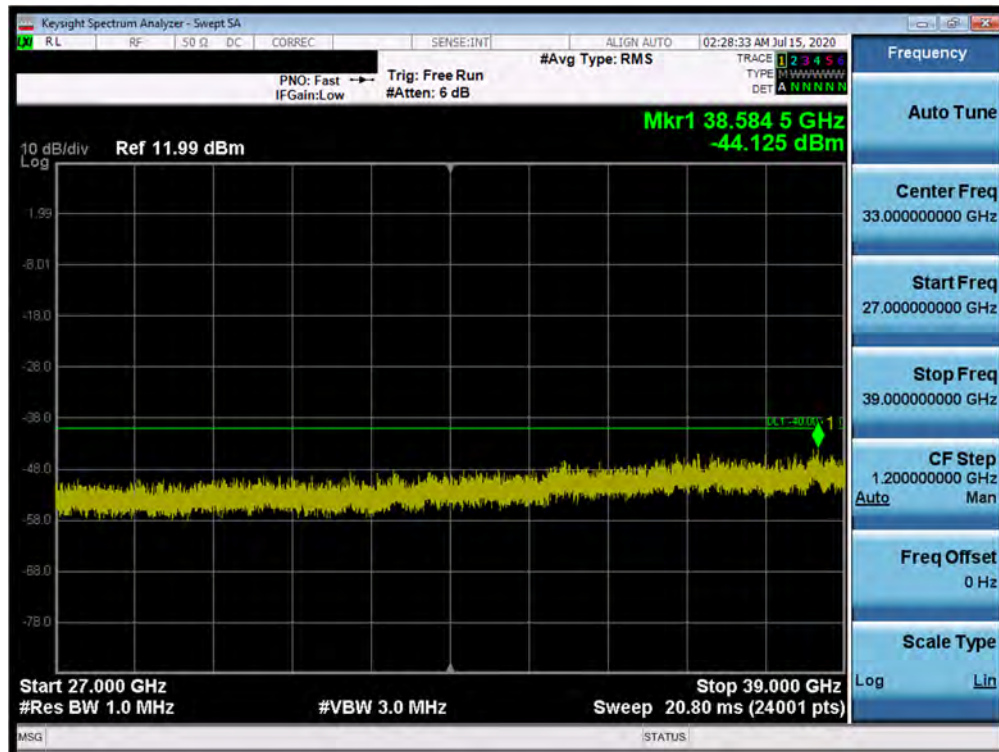
Plot 7-61. Conducted Spurious Plot (Band 48 – 20.0MHz QPSK – PCC 1/99 SCC 1/0 – Low Channel)
