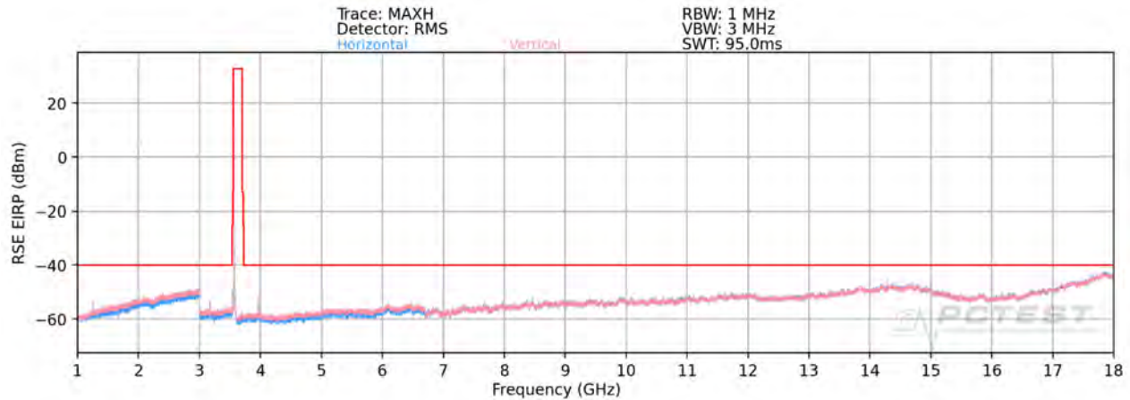
Plot 7-78. Radiated Spurious Plot 1GHz - 18GHz (ULCA Band 48) Low Channel – PCC/SCC: 1RB)
