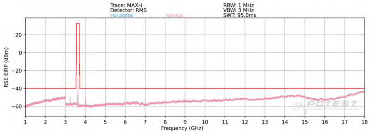
Plot 7-79. Radiated Spurious Plot 1GHz - 18GHz (ULCA Band 48) Mid Channel – PCC/SCC: 1RB)
