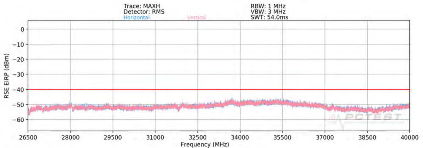
Plot 7-77. Radiated Spurious Plot (26.5 – 40GHz) – Band 48
