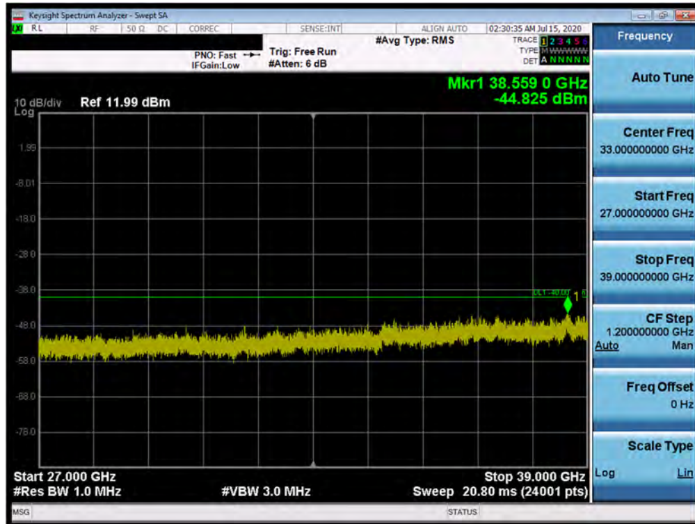
Plot 7-66. Conducted Spurious Plot (Band 48 – 20.0MHz QPSK – PCC 1/99 SCC 1/0 – Mid Channel)
