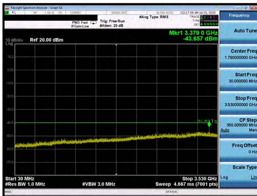
Plot 7-57. Conducted Spurious Plot (Band 48 – 20.0MHz QPSK – PCC 1/99 SCC 1/0 – Low Channel)
