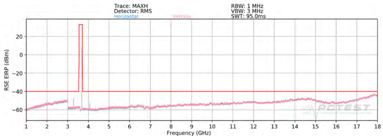
Plot 7-80. Radiated Spurious Plot 1GHz - 18GHz (ULCA Band 48) High Channel – PCC/SCC: 1RB)
