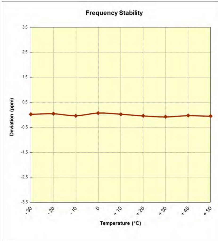
Figure 7-9. Frequency Stability Graph (LTE Band 48)
