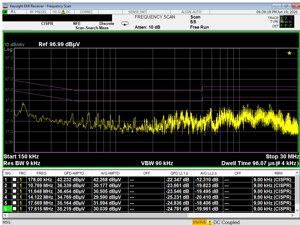
Plot 7-48. Line-Conducted Test Plot (N)
