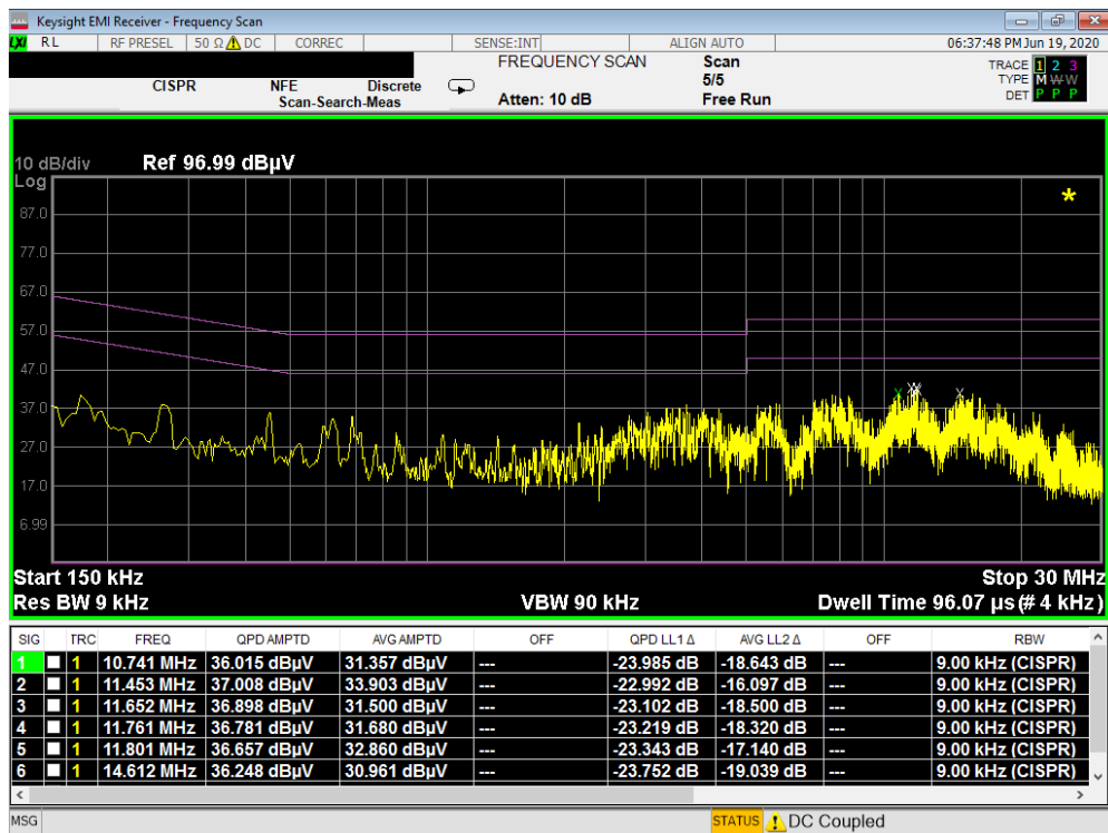
Plot 7-47. Line-Conducted Test Plot (L1)
