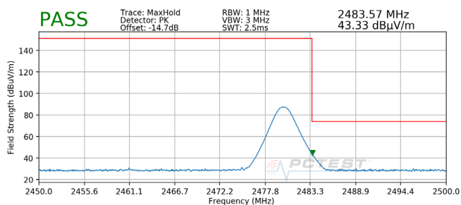
Plot 7-46. Radiated Restricted Upper Band Edge Measurement (Peak)
