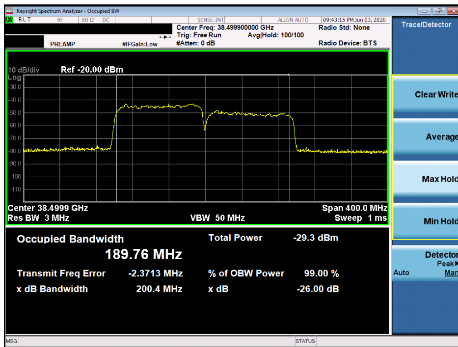
Plot 7-31. Ant 1 Occupied Bandwidth Plot (100MHz-2CC – 64QAM – Mid Channel)
