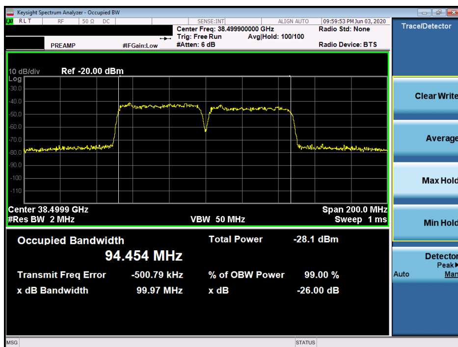
Plot 7-22. Ant 1 Occupied Bandwidth Plot (50MHz-2CC – 16QAM – Mid Channel)
