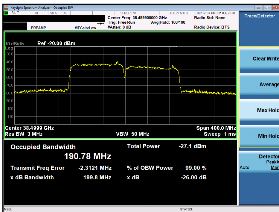
Plot 7-30. Ant 1 Occupied Bandwidth Plot (100MHz-2CC – 16QAM – Mid Channel)
