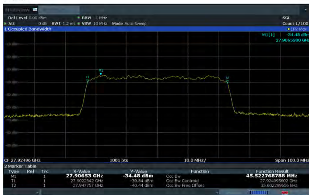
Plot 7-3. Ant 1 Occupied Bandwidth Plot (50MHz-1CC – 64QAM – Mid Channel)
