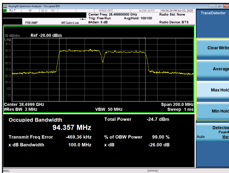
Plot 7-24. Ant 1 Occupied Bandwidth Plot (50MHz-2CC – pi/2-BPSK – Mid Channel)
