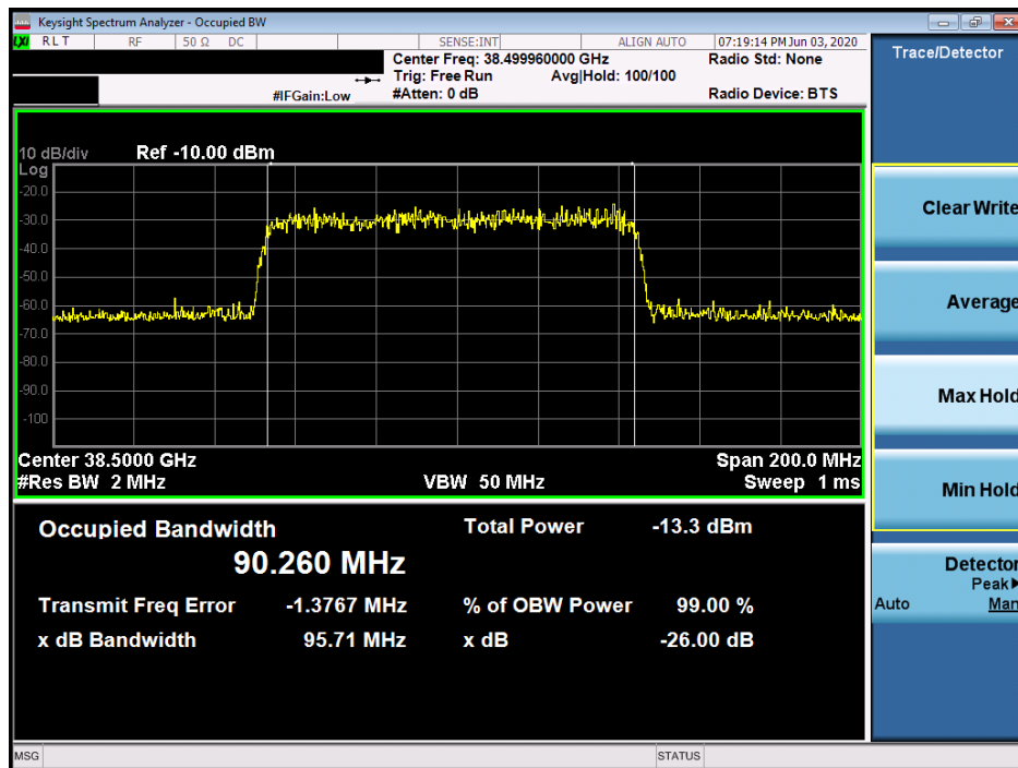
Plot 7-28. Ant 1 Occupied Bandwidth Plot (100MHz-1CC – pi/2-BPSK – Mid Channel)
