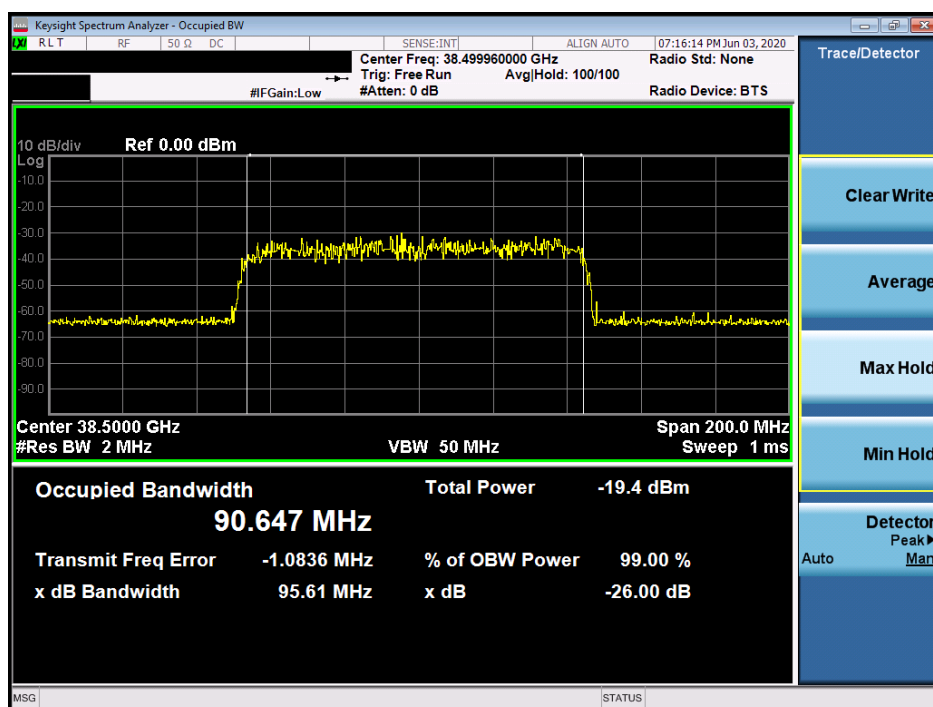
Plot 7-26. Ant 1 Occupied Bandwidth Plot (100MHz-1CC – 16QAM – Mid Channel)
