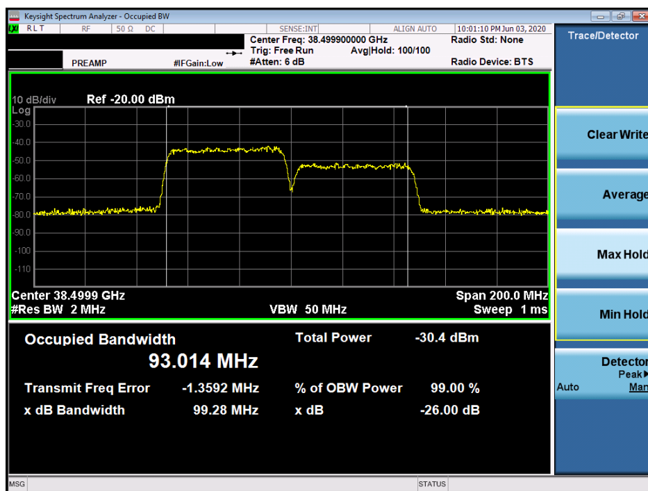
Plot 7-23. Ant 1 Occupied Bandwidth Plot (50MHz-2CC – 64QAM – Mid Channel)
