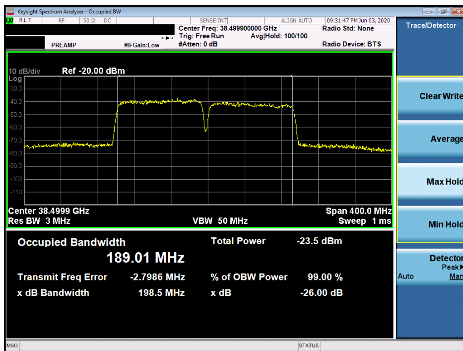
Plot 7-32. Ant 1 Occupied Bandwidth Plot (100MHz-2CC – pi/2-BPSK – Mid Channel)
