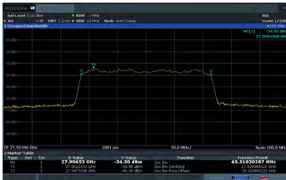
Plot 7-2. Ant 1 Occupied Bandwidth Plot (50MHz-1CC – 16QAM – Mid Channel)
