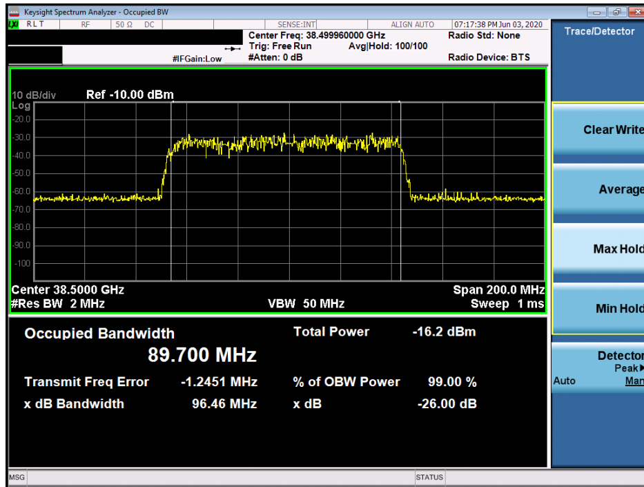
Plot 7-27. Ant 1 Occupied Bandwidth Plot (100MHz-1CC – 64QAM – Mid Channel)
