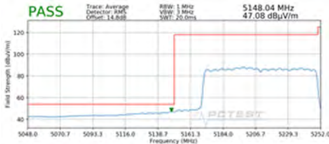
Plot 7-417. Radiated Lower Band Edge Plot MIMO (Average – UNII Band 1 – 996 Tones)
