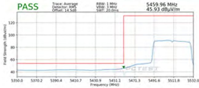
Plot 7-372. Radiated Lower Band Edge Plot SISO ANT1 (Average - UNII Band 2C - 484 Tones)
