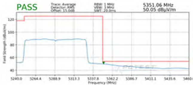
Plot 7-377. Radiated Upper Band Edge Plot SISO ANT1 (Average - UNII Band 2A - 996 Tones)
