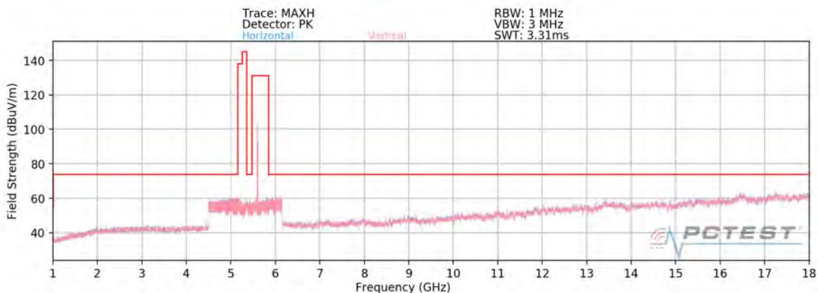
Plot 7-327. Radiated Spurious Plot above 1GHz SISO ANT1 (802.11ax – U2C Ch. 120 – 26 Tones)
