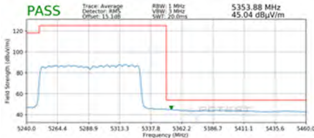
Plot 7-419. Radiated Upper Band Edge Plot MIMO (Average – UNII Band 2A – 996 Tones)
