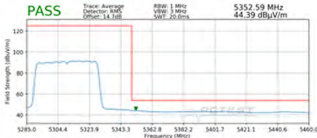
Plot 7-412. Radiated Upper Band Edge Plot MIMO (Average - UNII Band 2A - 484 Tones)
