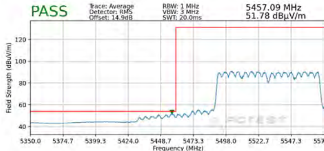
Plot 7-331. Radiated Lower Band Edge Plot MIMO (Average – UNII Band 2C)
