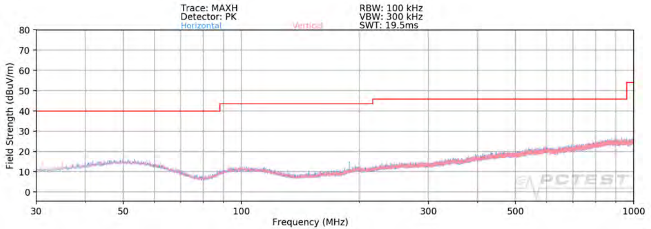
Plot 7-334. Radiated Spurious Plot below 1GHz CDD (802.11a – U3 Ch. 157)
