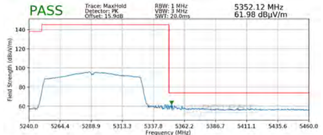
Plot 7-309. Radiated Upper Band Edge Plot SISO ANT2 (Peak – UNII Band 2A)
