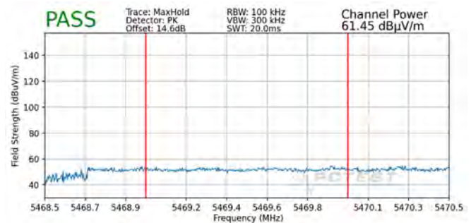
Plot 7-311. Radiated Lower Band Edge Plot SISO ANT2 (Peak – UNII Band 2C)
