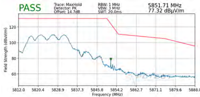
Plot 7-319. Radiated Upper Band Edge Plot MIMO (Peak - UNII Band 3)
