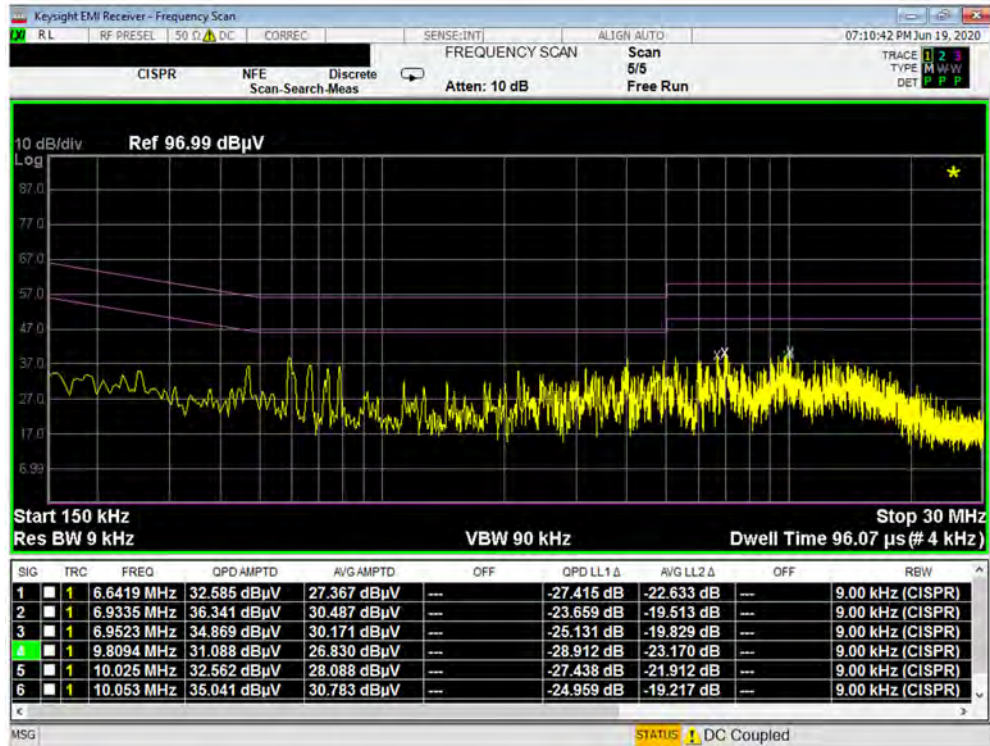
Plot 7-339. Line Conducted Plot with 802.11a UNII Band 2C (L1)
