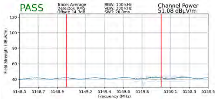
Plot 7-320. Radiated Lower Band Edge Plot MIMO (Average – UNII Band 1)
