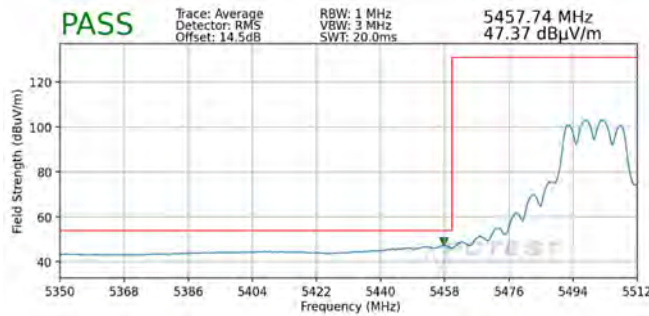
Plot 7-317. Radiated Lower Band Edge Plot MIMO (Average - UNII Band 2C)
