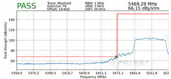
Plot 7-325. Radiated Lower Band Edge Plot MIMO (Peak – UNII Band 2C)
