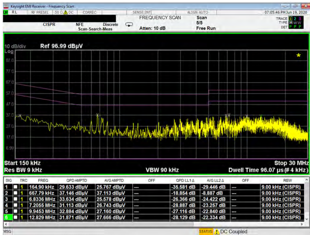
Plot 7-336. Line Conducted Plot with 802.11a UNII Band 1 (N)
