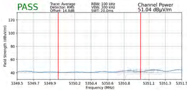
Plot 7-315. Radiated Upper Band Edge Plot MIMO (Average – UNII Band 2A)
