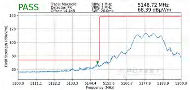
Plot 7-314. Radiated Lower Band Edge Plot MIMO (Peak – UNII Band 1)
