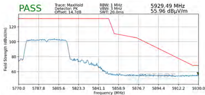
Plot 7-326. Radiated Upper Band Edge Plot MIMO (Peak – UNII Band 3)
