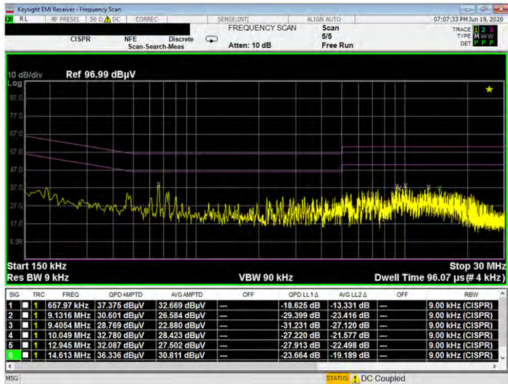
Plot 7-338. Line Conducted Plot with 802.11a UNII Band 2A (N)
