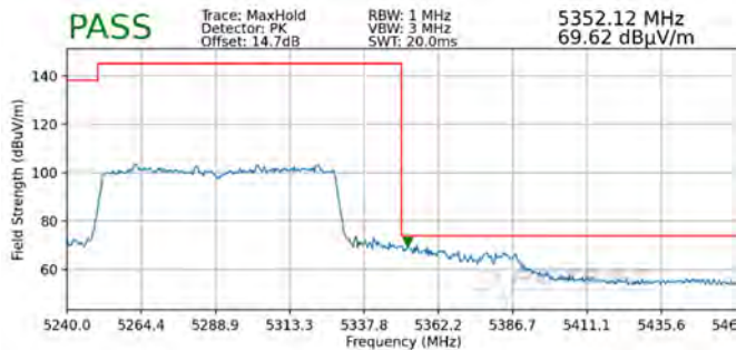
Plot 7-330. Radiated Upper Band Edge Plot MIMO (Peak – UNII Band 2A)
