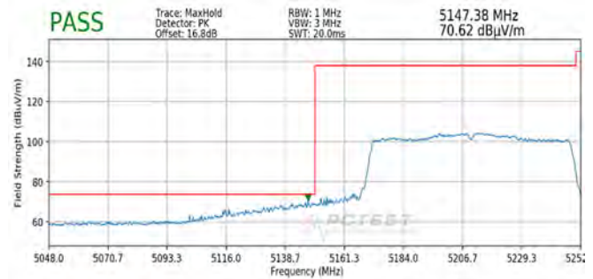
Plot 7-328. Radiated Lower Band Edge Plot MIMO (Peak – UNII Band 1)
