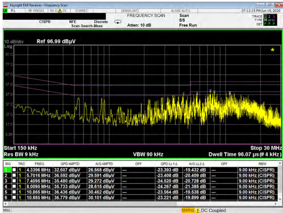
Plot 7-340. Line Conducted Plot with 802.11a UNII Band 2C (N)
