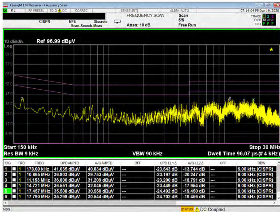
Plot 7-342. Line Conducted Plot with 802.11a UNII Band 3 (N)
