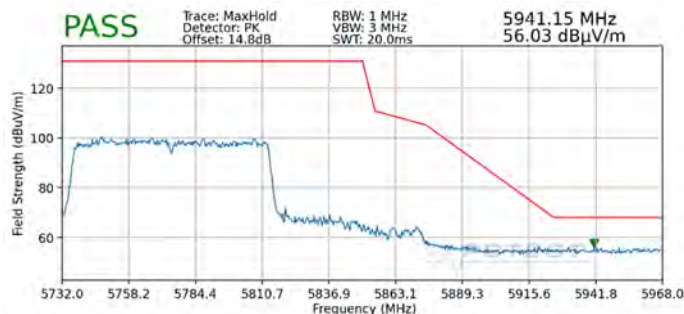
Plot 7-333. Radiated Upper Band Edge Plot MIMO (Peak – UNII Band 3)
