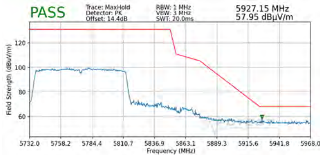
Plot 7-312. Radiated Upper Band Edge Plot SISO ANT2 (Peak – UNII Band 3)
