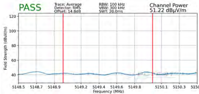
Plot 7-327. Radiated Lower Band Edge Plot MIMO (Average – UNII Band 1)
