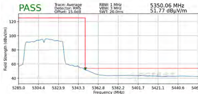
Plot 7-322. Radiated Upper Band Edge Plot MIMO (Average – UNII Band 2A)
