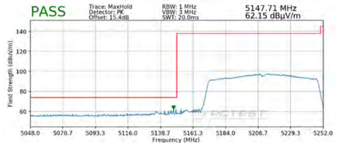
Plot 7-307. Radiated Lower Band Edge Plot SISO ANT2 (Peak – UNII Band 1)
