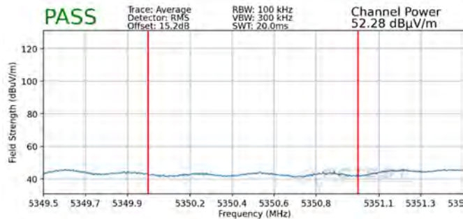
Plot 7-329. Radiated Upper Band Edge Plot MIMO (Average – UNII Band 2A)
