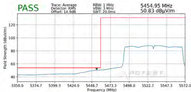
Plot 7-310. Radiated Lower Band Edge Plot SISO ANT2 (Average – UNII Band 2C)
