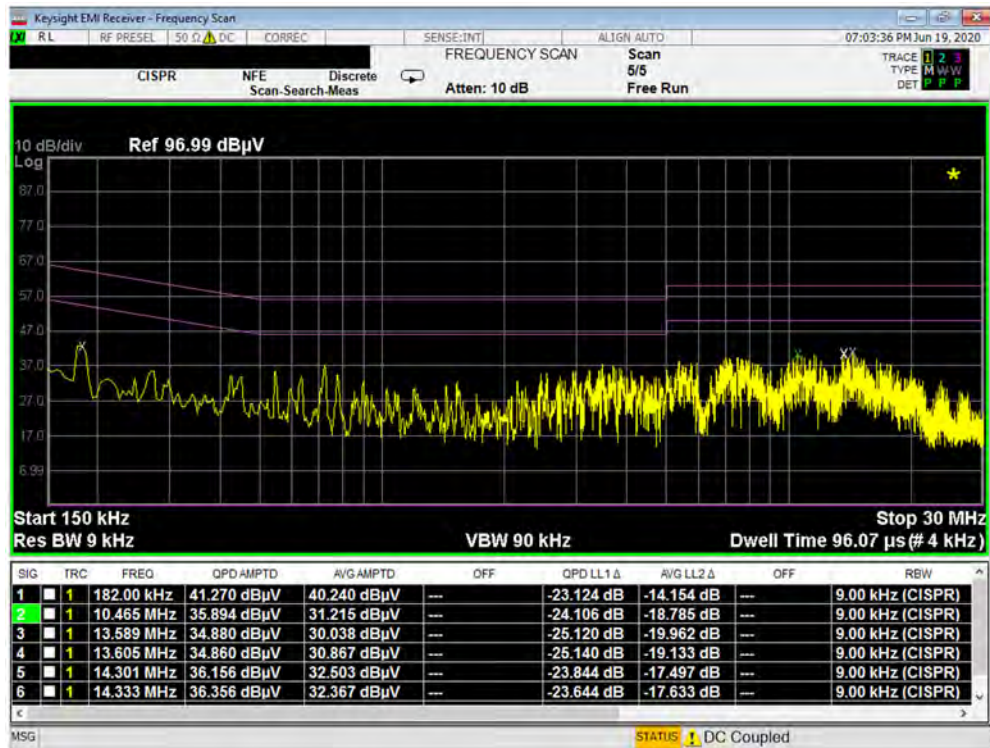
Plot 7-335. Line Conducted Plot with 802.11a UNII Band 1 (L1)
