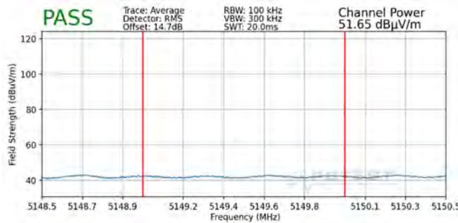
Plot 7-306. Radiated Lower Band Edge Plot SISO ANT2 (Average – UNII Band 1)
