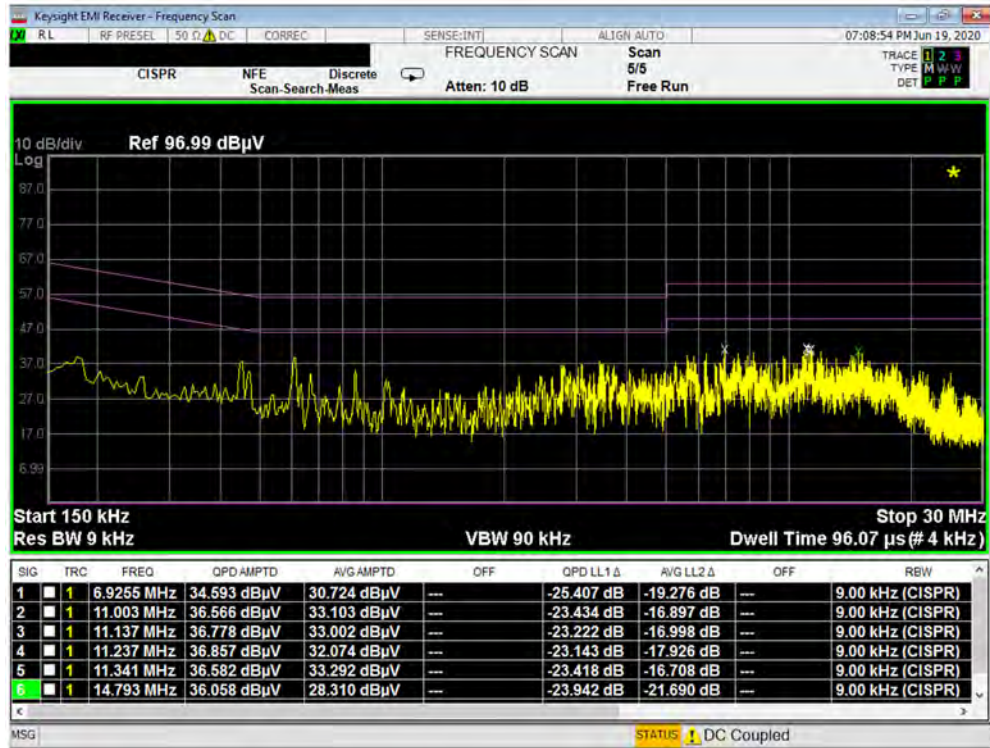
Plot 7-337. Line Conducted Plot with 802.11a UNII Band 2A (L1)
