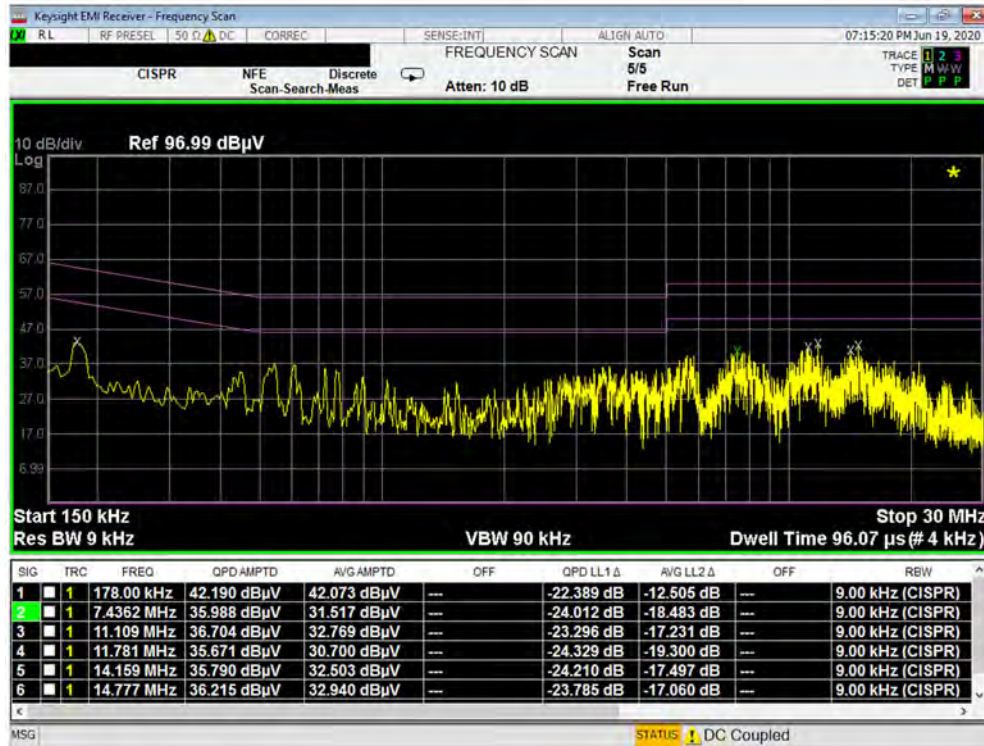
Plot 7-341. Line Conducted Plot with 802.11a UNII Band 3 (L1)
