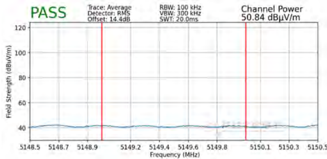
Plot 7-313. Radiated Lower Band Edge Plot MIMO (Average – UNII Band 1)
