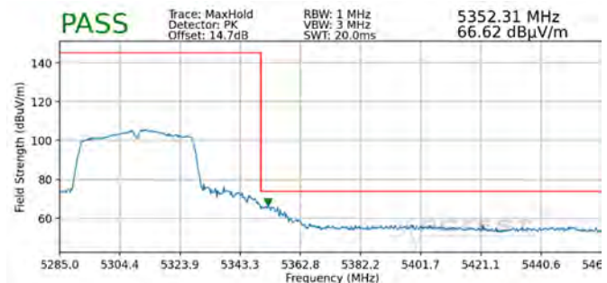
Plot 7-323. Radiated Upper Band Edge Plot MIMO (Peak – UNII Band 2A)
