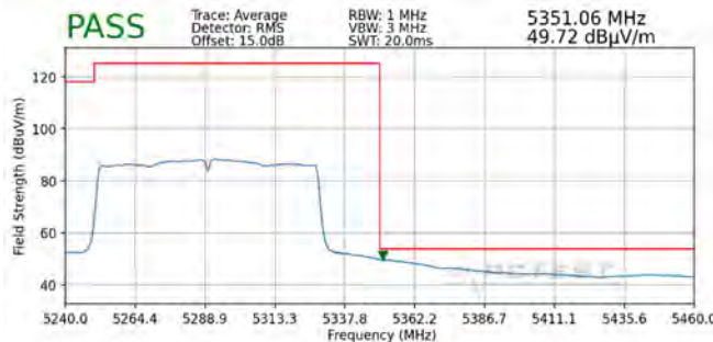
Plot 7-308. Radiated Upper Band Edge Plot SISO ANT2 (Average – UNII Band 2A)
