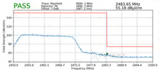
Plot 7-108. Radiated Restricted Upper Band Edge Measurement SISO ANT2 (Peak – 242 Tones)
