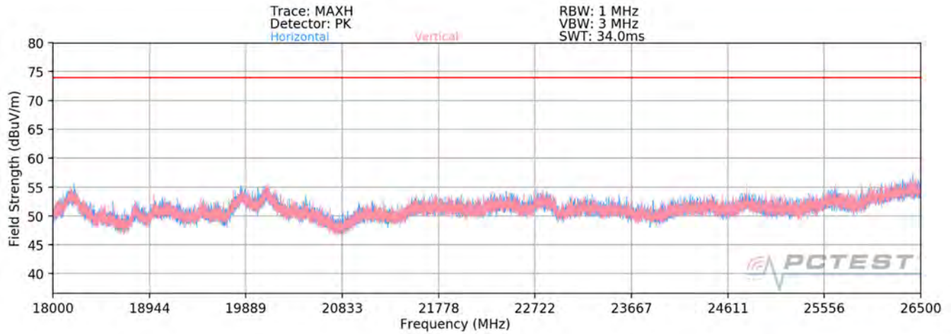
Plot 7-83. Radiated Spurious Plot above 18GHz SISO ANT2 (802.11ax OFDMA – 106 Tones)
