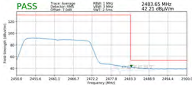
Plot 7-115. Radiated Restricted Upper Band Edge Measurement MIMO (Average - 242 Tones)
