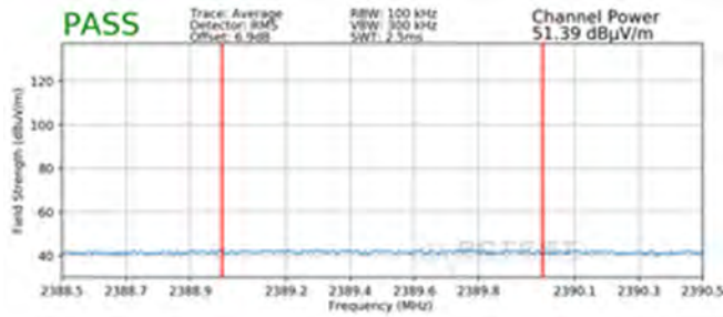
Plot 7-105. Radiated Restricted Lower Band Edge Measurement SISO ANT2 (Average – 242 Tones)
