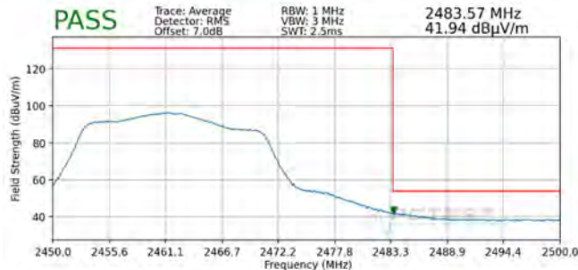
Plot 7-99. Radiated Restricted Upper Band Edge Measurement SISO ANT1 (Average - 242 Tones)
