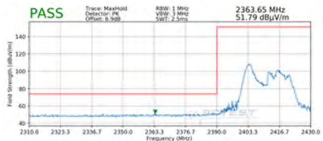
Plot 7-110. Radiated Restricted Lower Band Edge Measurement MIMO (Peak – 26 Tones)
