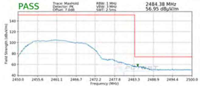
Plot 7-100. Radiated Restricted Upper Band Edge Measurement SISO ANT1 (Peak - 242 Tones)
