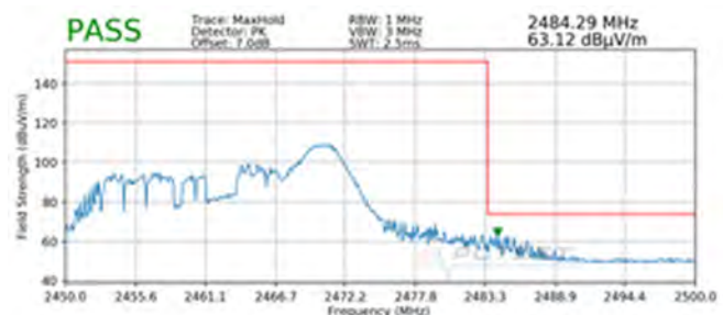
Plot 7-104. Radiated Restricted Upper Band Edge Measurement SISO ANT2 (Peak – 26 Tones)
