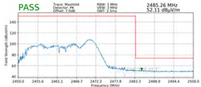
Plot 7-112. Radiated Restricted Upper Band Edge Measurement MIMO (Peak – 26 Tones)
