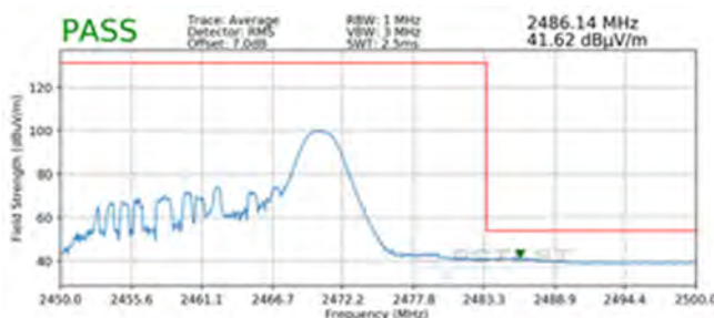
Plot 7-103. Radiated Restricted Upper Band Edge Measurement SISO ANT2 (Average – 26 Tones)
