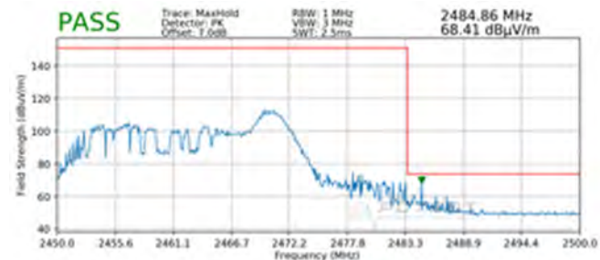
Plot 7-96. Radiated Restricted Upper Band Edge Measurement SISO ANT1 (Peak - 26 Tones)
