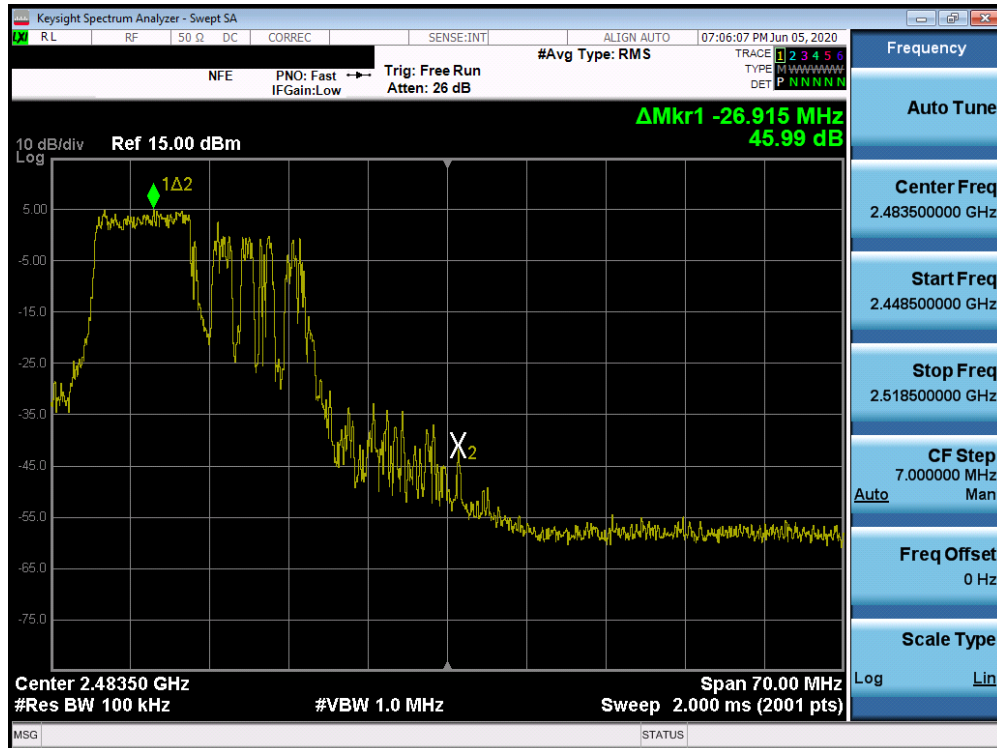
Plot 7-42. Band Edge Plot SISO ANT2 (802.11ax OFDMA – 106 Tones – Ch. 11)
