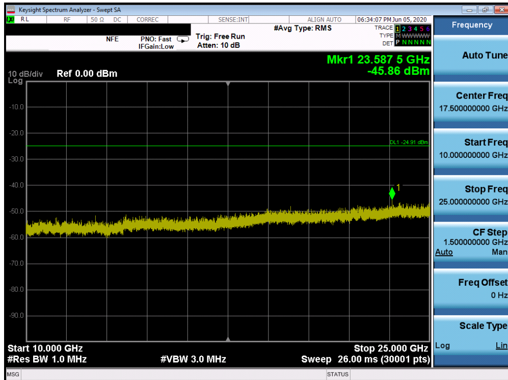
Plot 7-54. Conducted Spurious Plot SISO ANT1 (802.11ax OFDMA – 242 Tones – Ch. 6)
