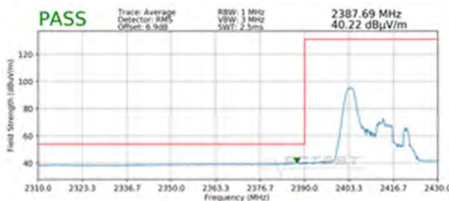
Plot 7-101. Radiated Restricted Lower Band Edge Measurement SISO ANT2 (Average – 26 Tones)
