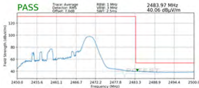
Plot 7-111. Radiated Restricted Upper Band Edge Measurement MIMO (Average – 26 Tones)
