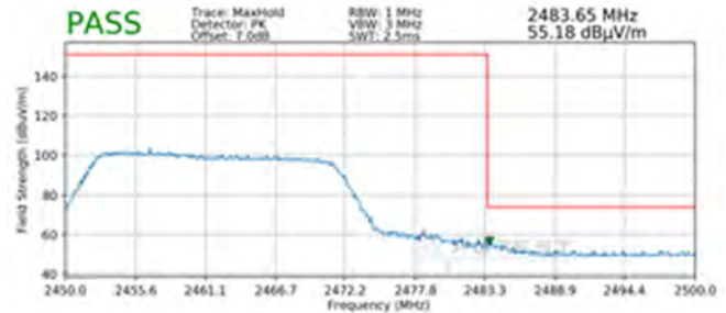
Plot 7-116. Radiated Restricted Upper Band Edge Measurement MIMO (Peak - 242 Tones)
