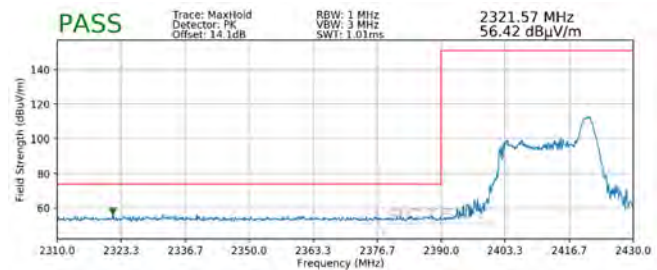
Plot 7-94. Radiated Restricted Lower Band Edge Measurement SISO ANT1 (Peak - 26 Tones)
