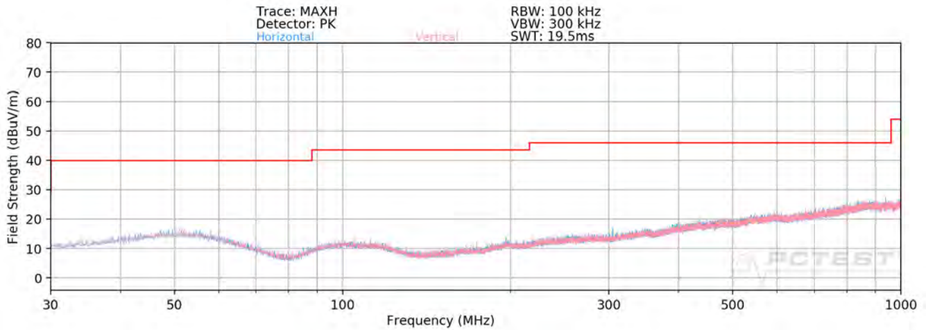
Plot 7-117. Radiated Spurious Plot below 1GHz MIMO (106 Tones)
