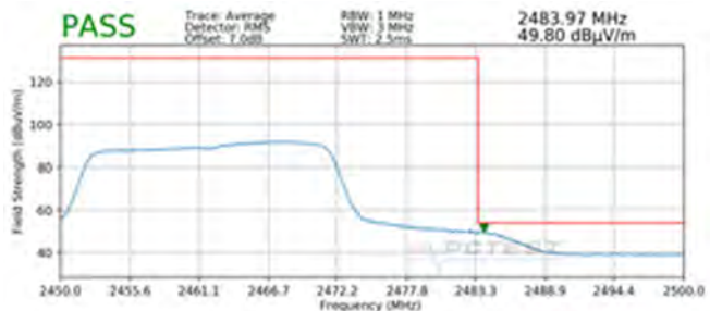
Plot 7-107. Radiated Restricted Upper Band Edge Measurement SISO ANT2 (Average – 242 Tones)
