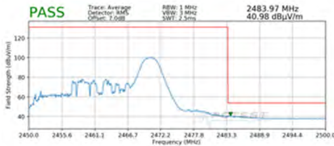
Plot 7-95. Radiated Restricted Upper Band Edge Measurement SISO ANT1 (Average - 26 Tones)
