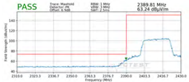
Plot 7-114. Radiated Restricted Lower Band Edge Measurement MIMO (Peak - 242 Tones)
