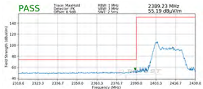
Plot 7-102. Radiated Restricted Lower Band Edge Measurement SISO ANT2 (Peak – 26 Tones)
