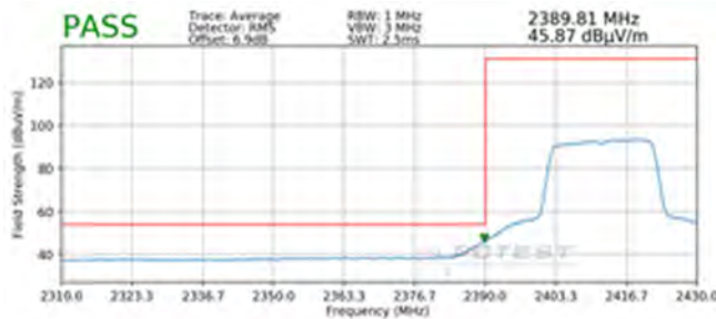
Plot 7-113. Radiated Restricted Lower Band Edge Measurement MIMO (Average - 242 Tones)
