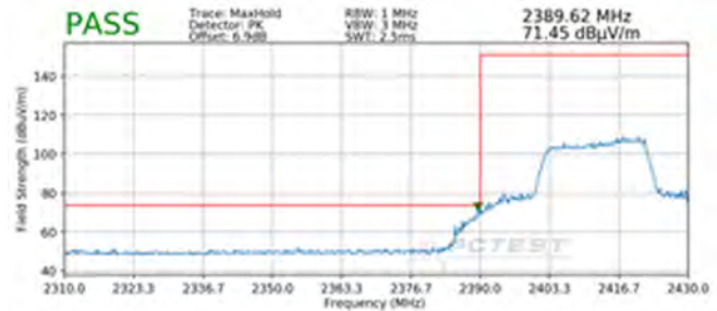
Plot 7-98. Radiated Restricted Lower Band Edge Measurement SISO ANT1 (Peak - 242 Tones)
