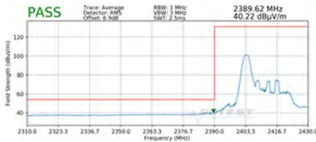
Plot 7-93. Radiated Restricted Lower Band Edge Measurement SISO ANT1 (Average - 26 Tones)
