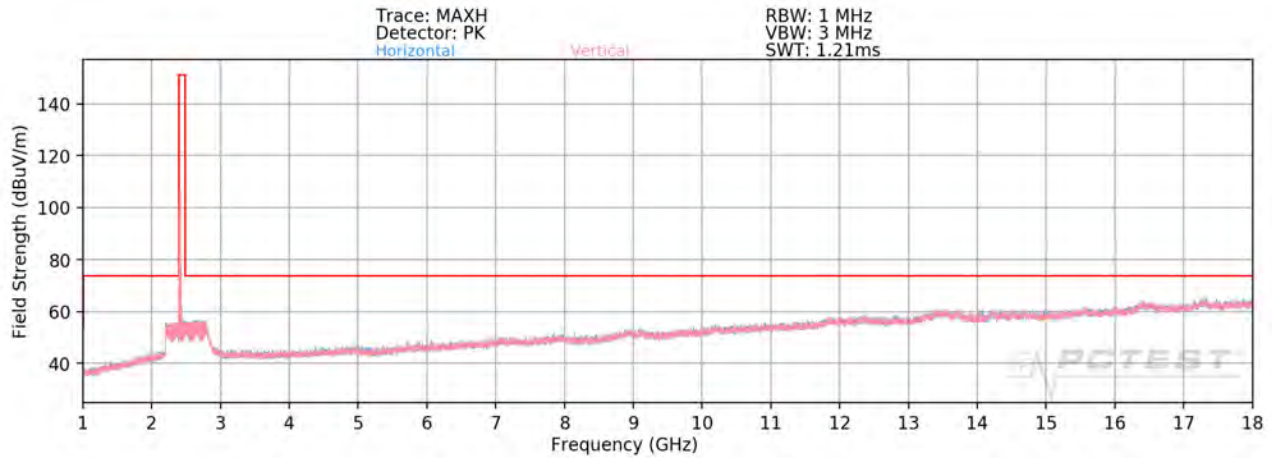
Plot 7-85. Radiated Spurious Plot above 1GHz MIMO/CDD (802.11g – Ch. 1)
