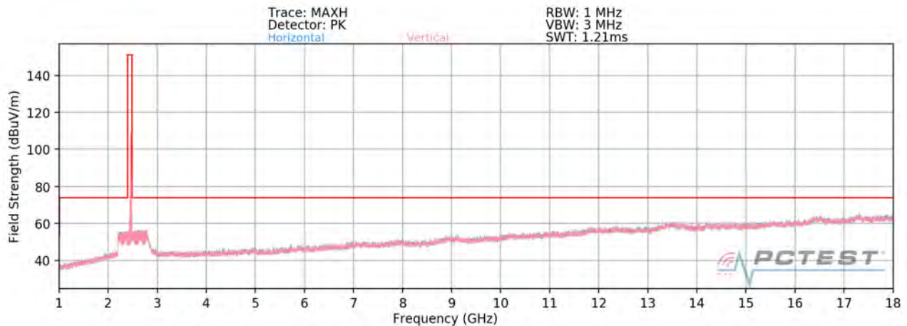
Plot 7-87. Radiated Spurious Plot above 1GHz MIMO/CDD (802.11g – Ch. 11)
