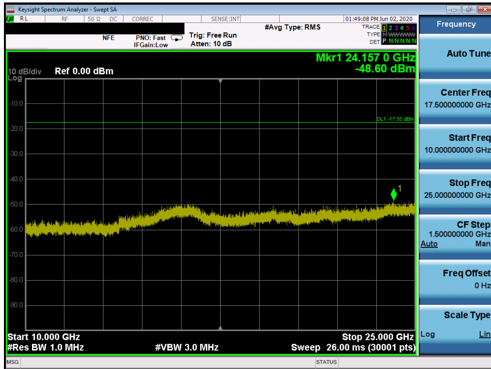
Plot 7-66. Conducted Spurious Plot SISO ANT1 (802.11b – Ch. 1)
