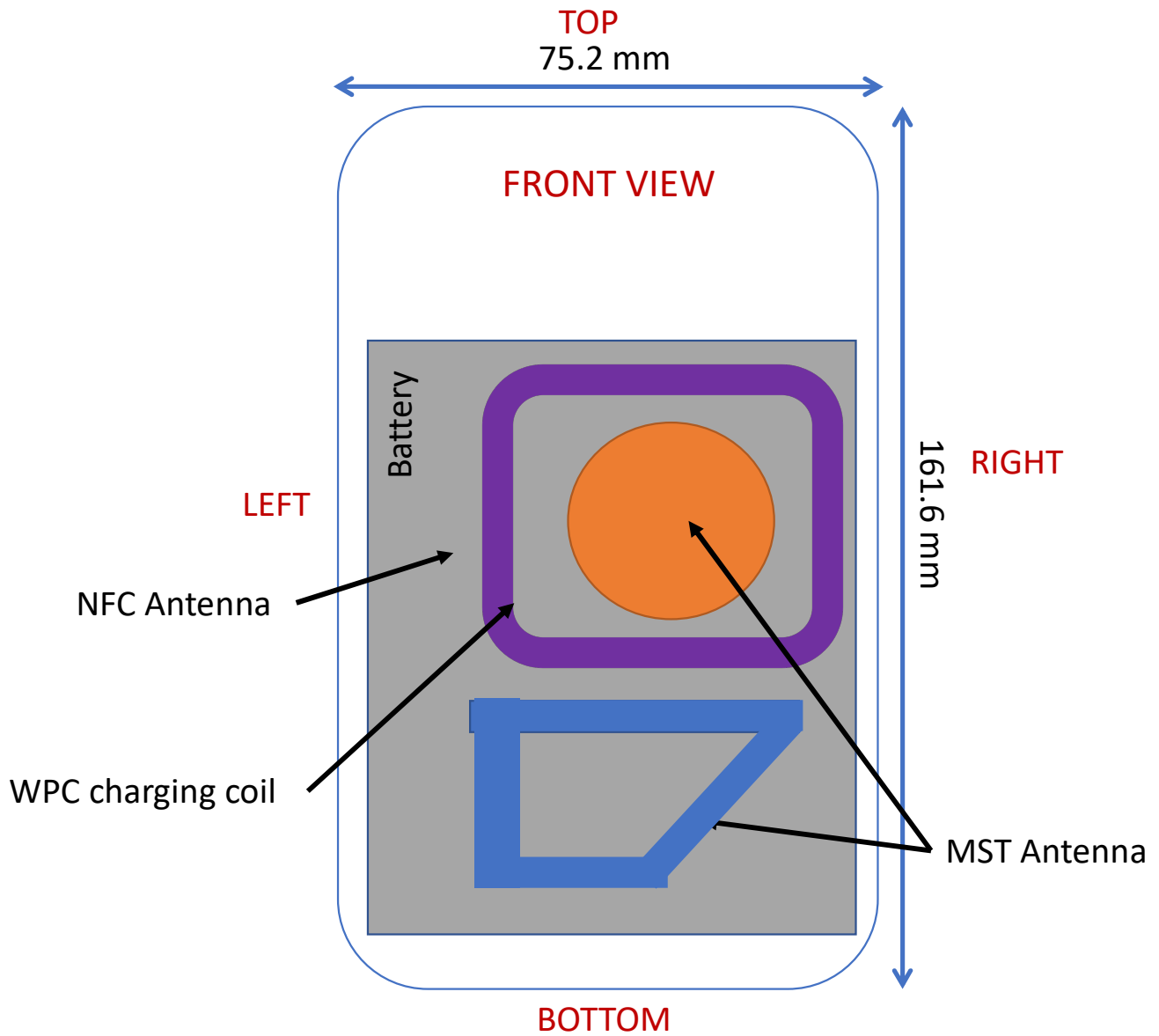
Figure E-2 WPC Charging Coil + MST/NFC Antenna Locations
