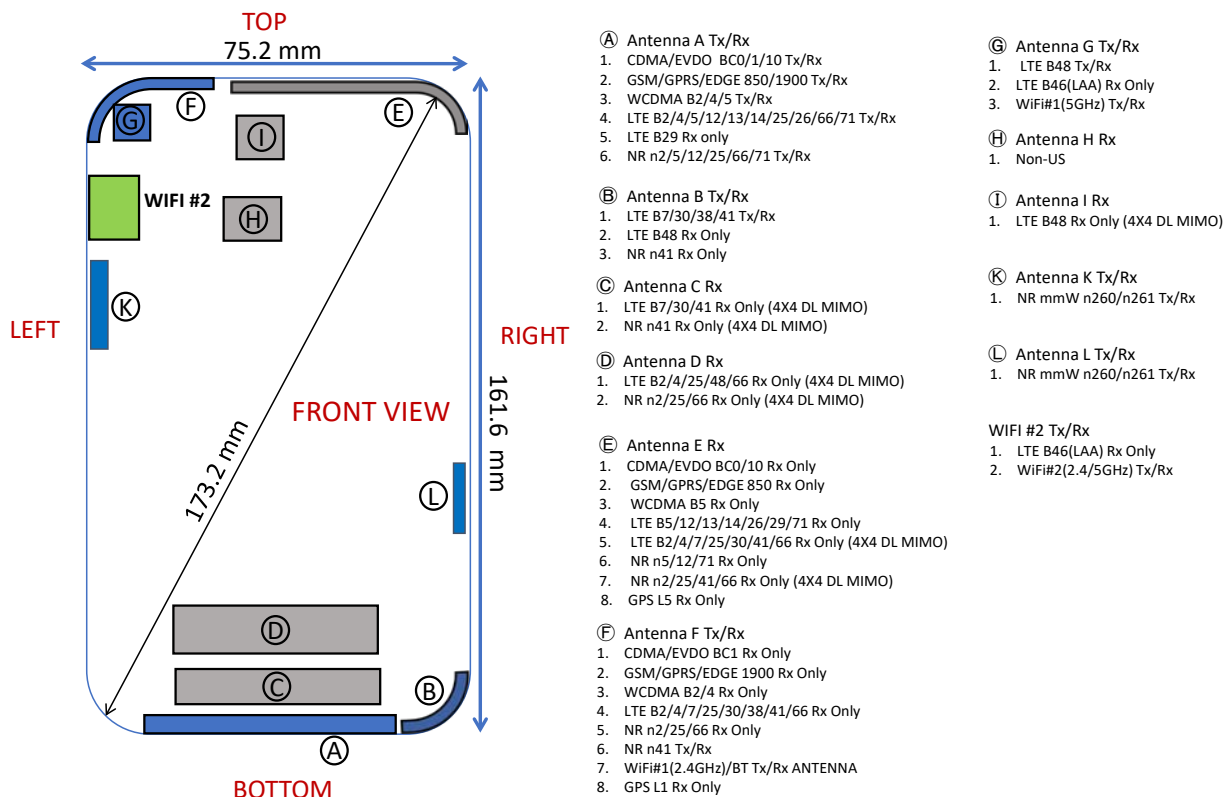
Figure E-1 DUT Antenna Locations
