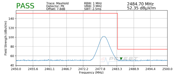
Plot 7-54. Radiated Restricted Upper Band Edge Measurement with WCP (Peak)
