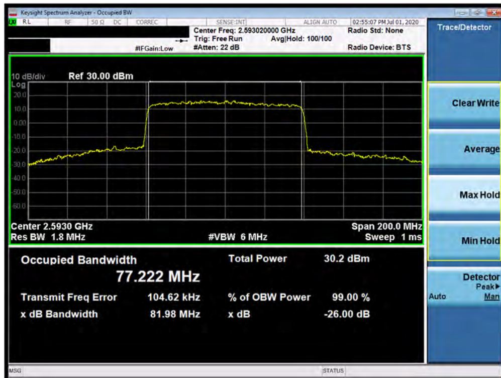
Plot 7-182. Occupied Bandwidth Plot (n41 80MHz QPSK-CP-OFDM - Full RB Configuration)
