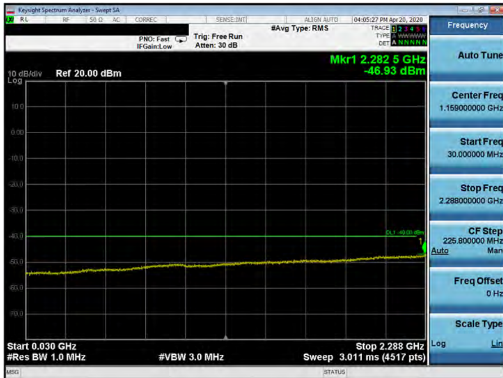
Plot 7-262. Conducted Spurious Plot (Band 30 - 10.0MHz QPSK - RB Size 1, RB Offset 0 - Mid Channel)
