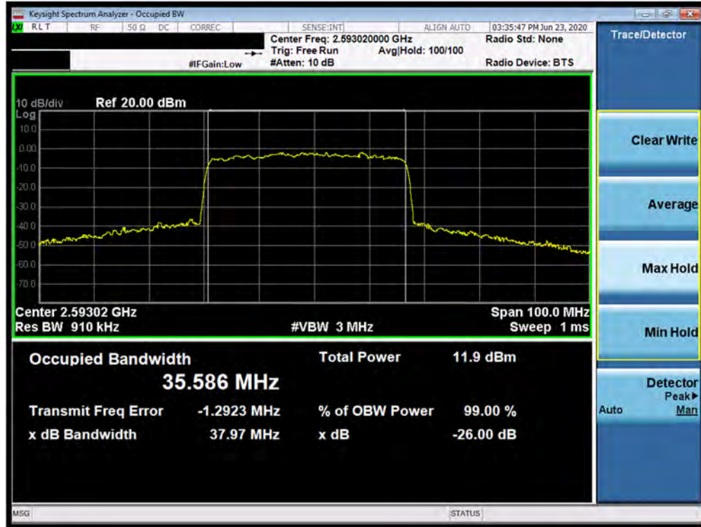
Plot 7-169. Occupied Bandwidth Plot (n41 40MHz 64QAM-CP-OFDM- Full RB Configuration)
