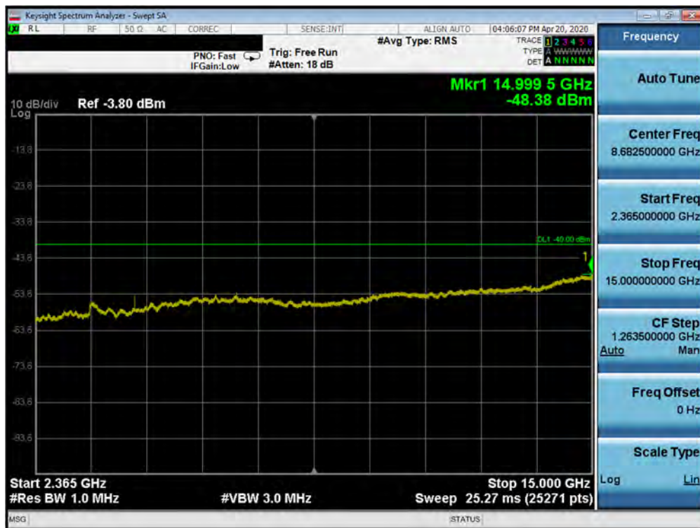
Plot 7-263. Conducted Spurious Plot (Band 30 - 10.0MHz QPSK - RB Size 1, RB Offset 0 - Mid Channel)
