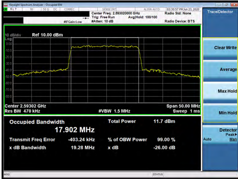
Plot 7-163. Occupied Bandwidth Plot (n41 20MHz 16QAM-CP-OFDM - Full RB Configuration)
