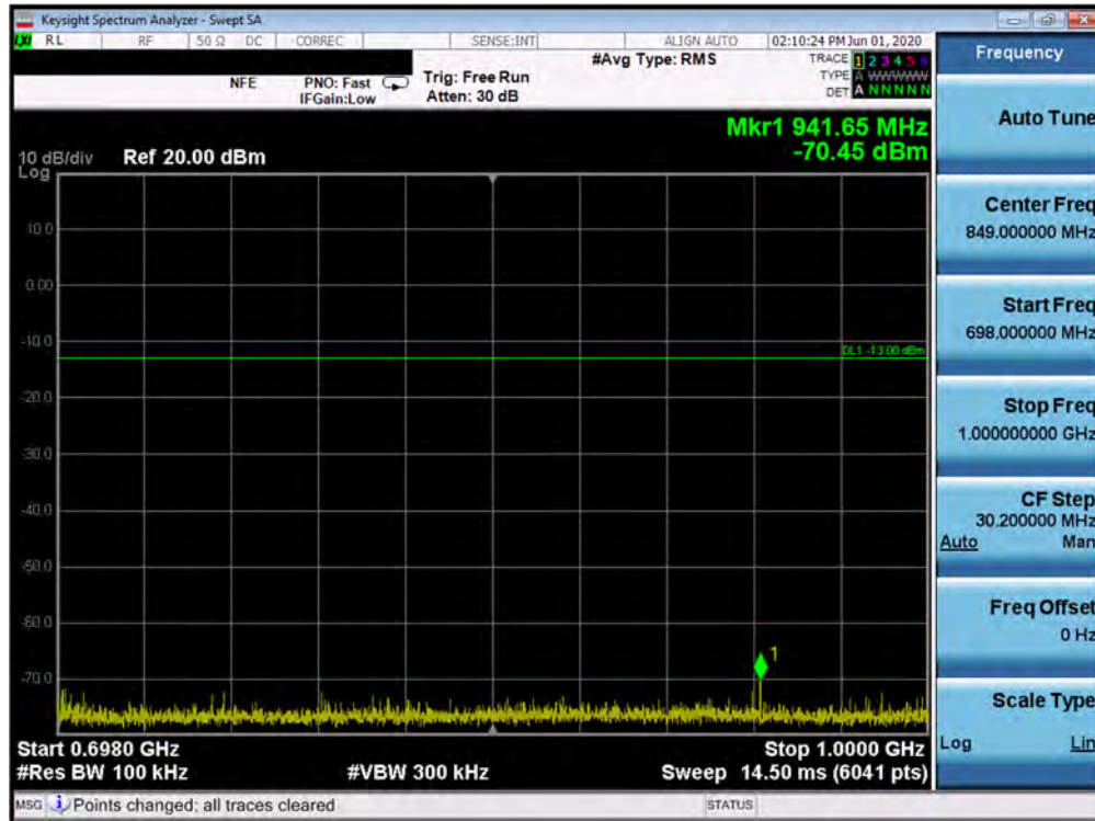
Plot 7-200. Conducted Spurious Plot (Band 71 - 20.0MHz QPSK - RB Size 1, RB Offset 0 - Mid Channel)
