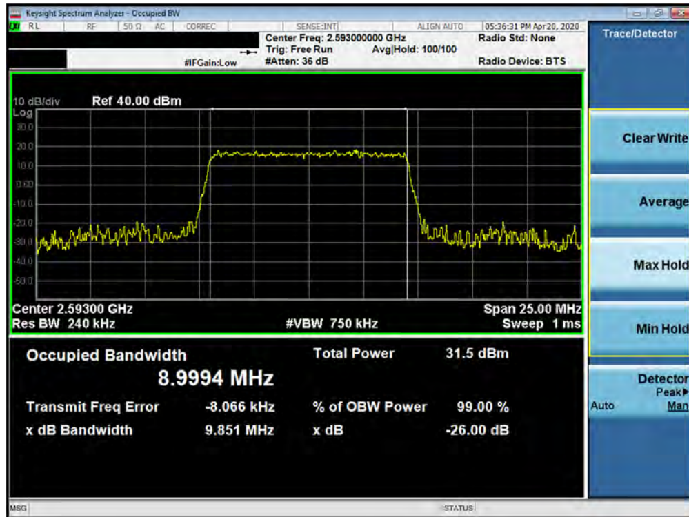
Plot 7-150. Occupied Bandwidth Plot (Band 41 - 10.0MHz 16-QAM - Full RB Configuration)
