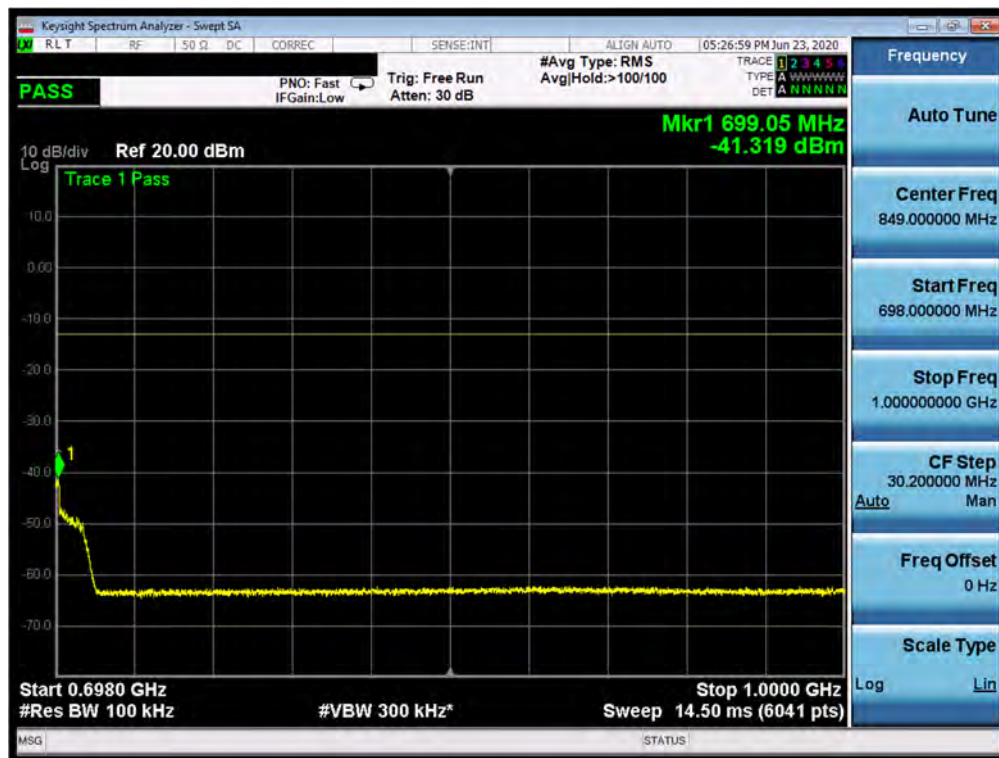
Plot 7-206. Conducted Spurious Plot (n71 - 20MHz DFT-s-OFDM-QPSK - RB Size 1, RB Offset 1 - Low Channel)
