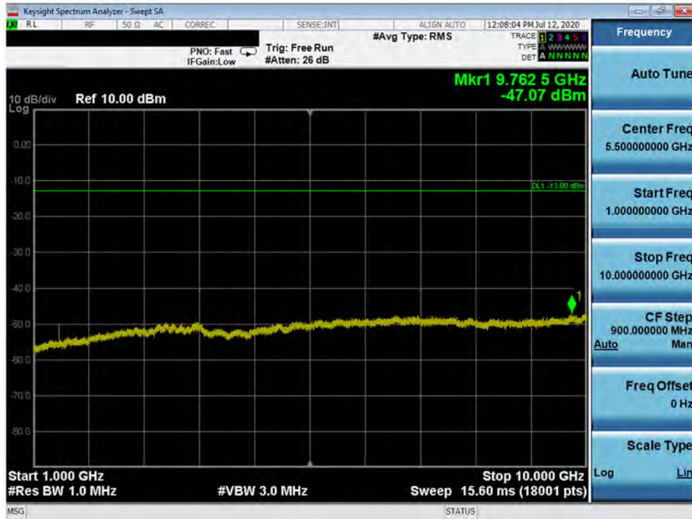
Plot 7-222. Conducted Spurious Plot (Band 12 - 10MHz QPSK - RB Size 1, RB Offset 0 - High Channel)
