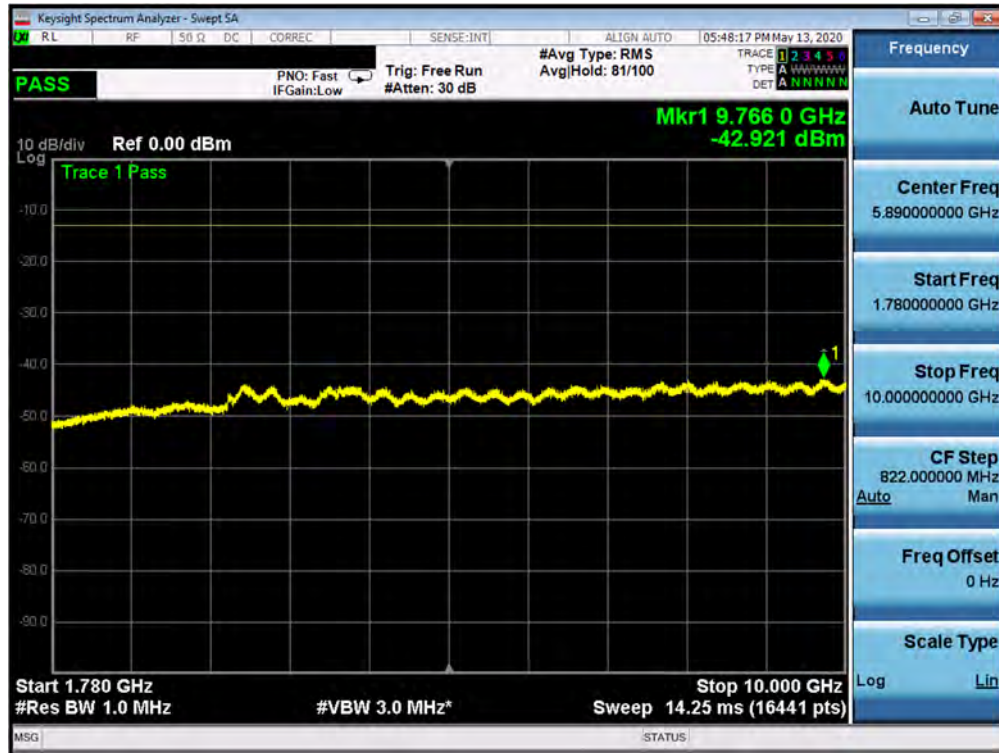
Plot 7-248. Conducted Spurious Plot (n66 - 20MHz DFT-s-OFDM-QPSK - RB Size 1, RB Offset 1 - Mid Channel)
