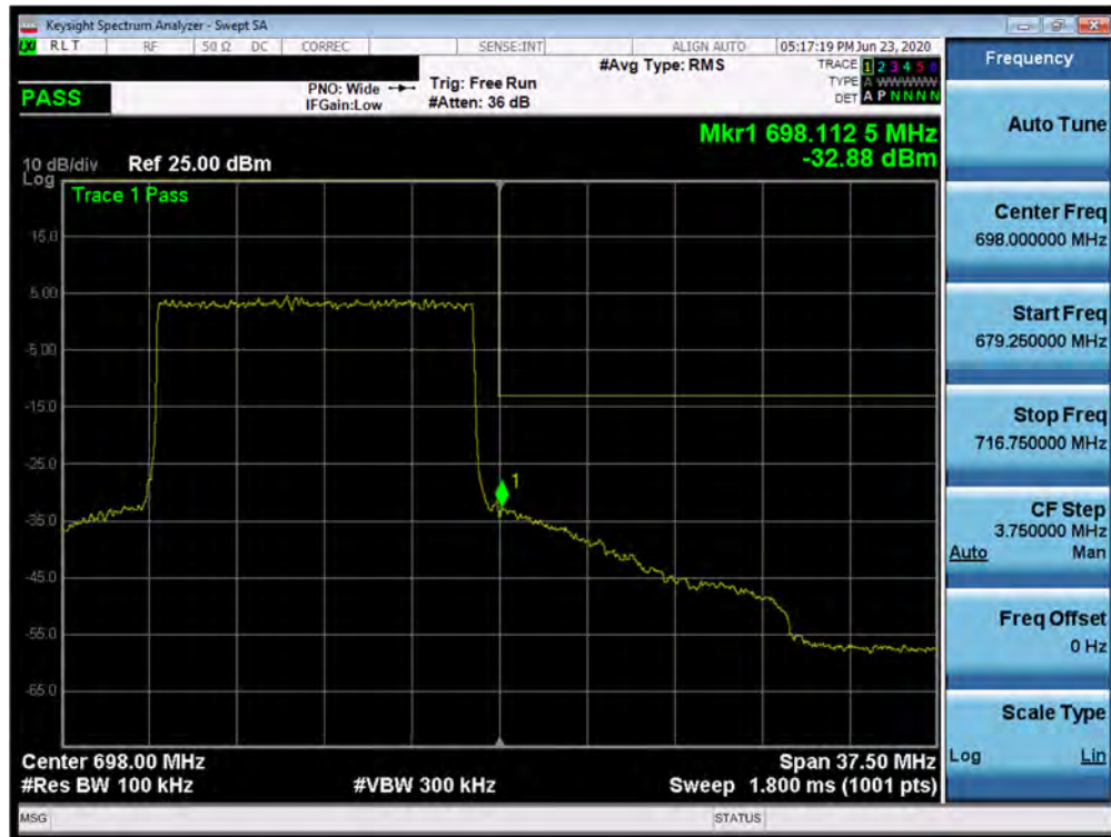
Plot 7-311. Upper Band Edge Plot (n71 - 15MHz DFT-s -OFDM-QPSK - Full RB Configuration)
