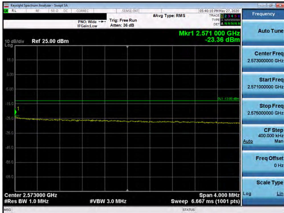
Plot 7-439. Upper Extended Band Edge Plot (Band 7 - 10.0MHz QPSK - Full RB Configuration)
