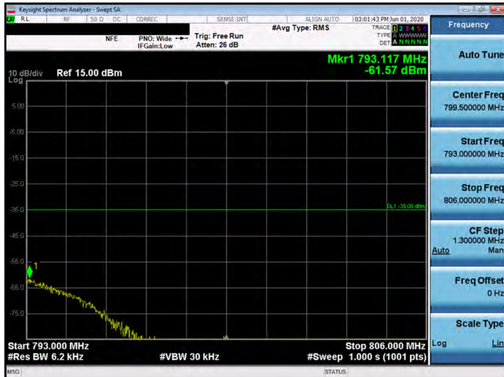
Plot 7-325. Upper Emission Mask Plot (Band 13 - 5.0MHz QPSK - Full RB Configuration)
