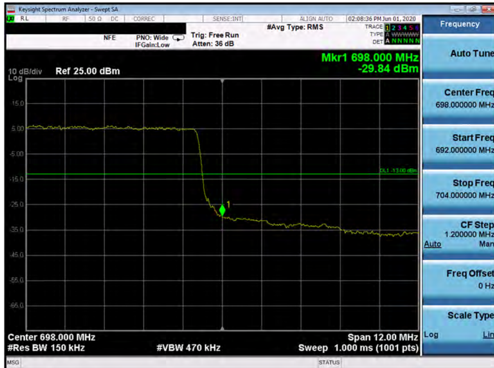
Plot 7-303. Upper Band Edge Plot (Band 71 - 15.0MHz QPSK - Full RB Configuration)
