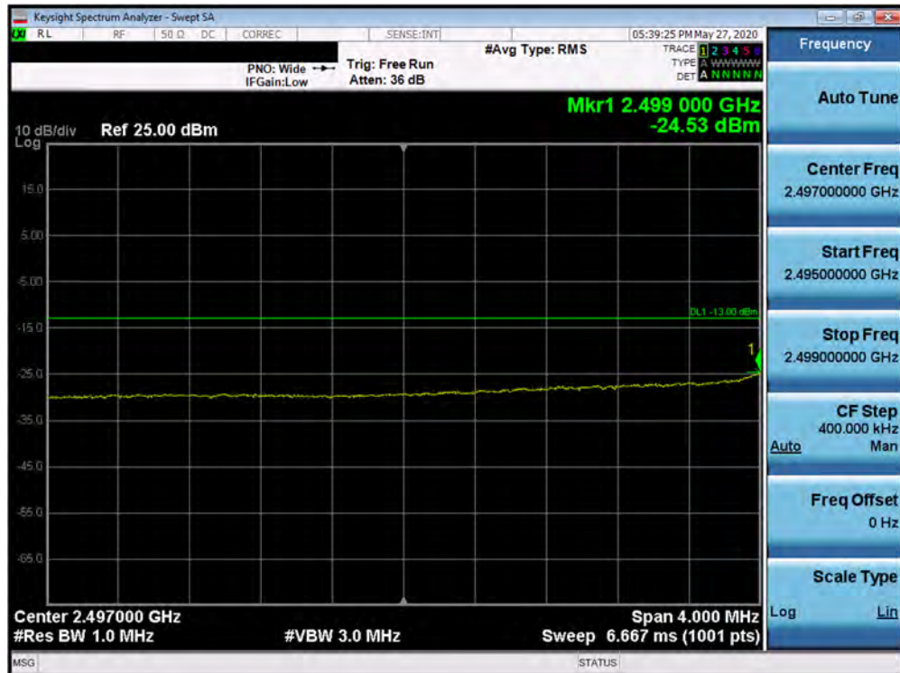
Plot 7-437. Lower Extended Band Edge Plot (Band 7 - 10.0MHz QPSK - Full RB Configuration)
