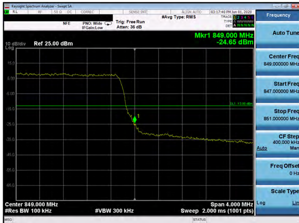
Plot 7-335. Upper Band Edge Plot (Band 5 - 5.0MHz QPSK - Full RB Configuration)
