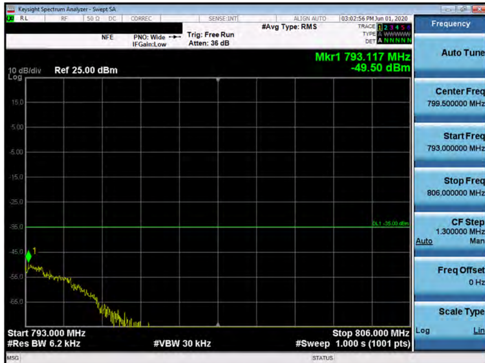
Plot 7-329. Upper Band Emission Mask Plot (Band 13 - 10.0MHz QPSK - Full RB Configuration)
