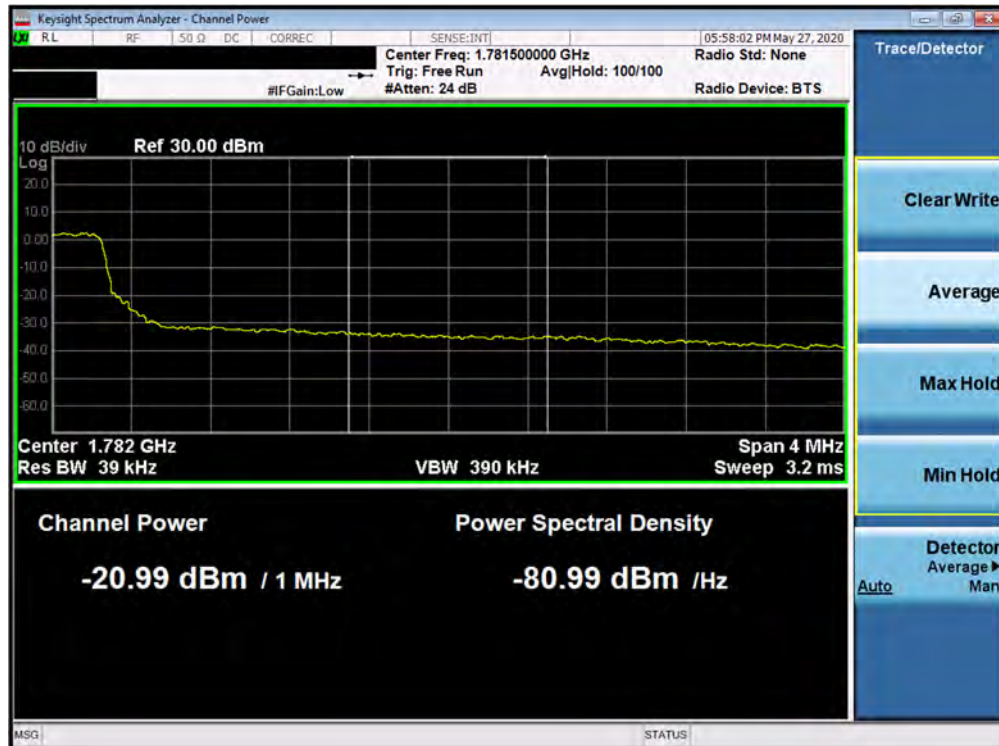
Plot 7-355. Upper Extended Band Edge Plot (Band 66 - 5.0MHz QPSK - Full RB Configuration)
