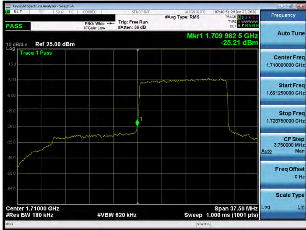
Plot 7-380. Lower Band Edge Plot (n66 - 15MHz DFT-s-OFDM-QPSK - Full RB Configuration)
