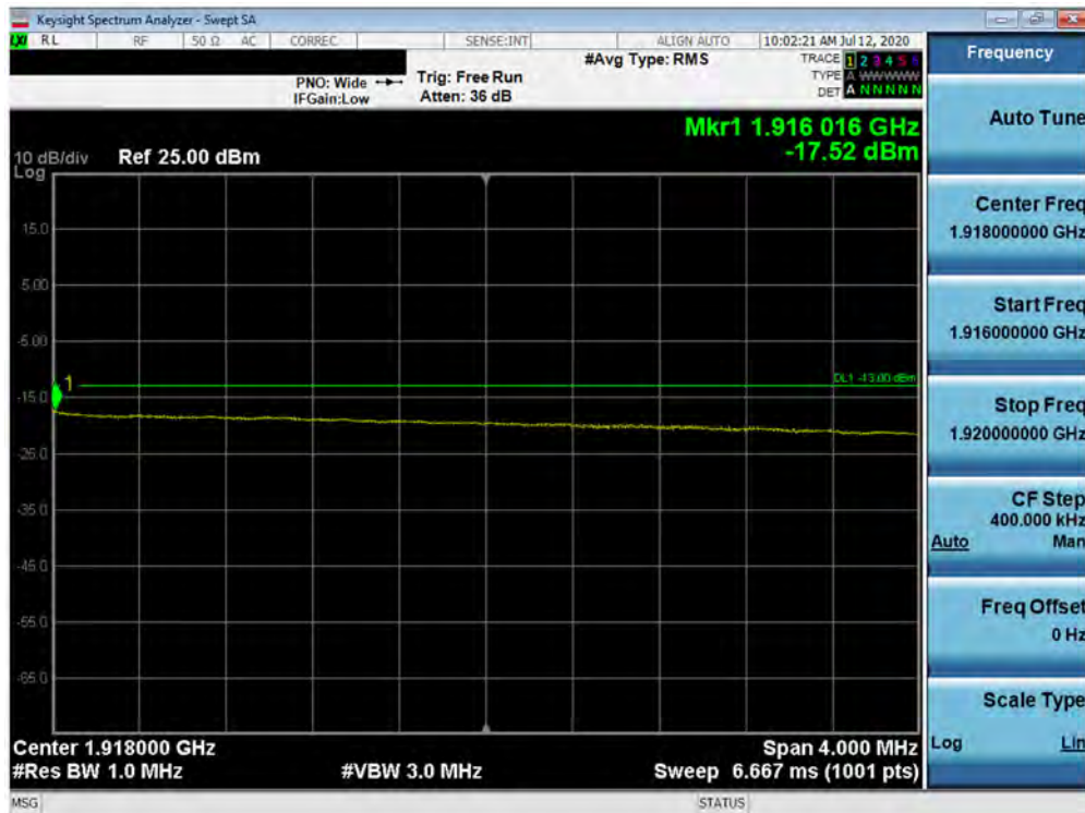
Plot 7-423. Upper Extended Band Edge Plot (Band 25 - 20.0MHz QPSK - Full RB Configuration)
