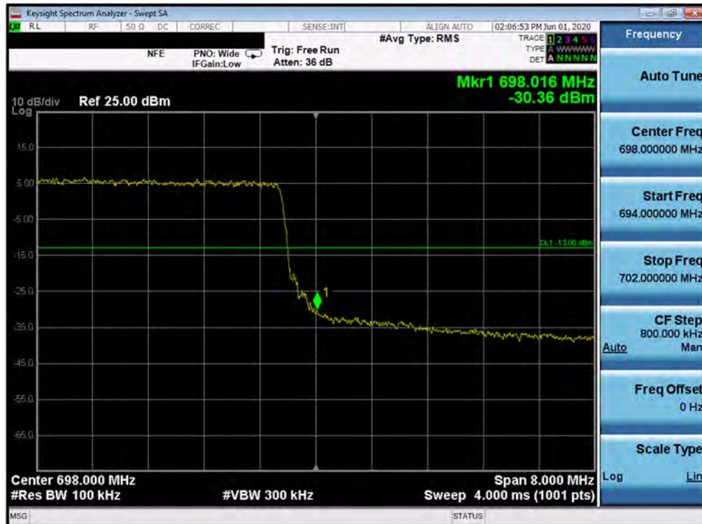
Plot 7-301. Upper Band Edge Plot (Band 71 - 10.0MHz QPSK - Full RB Configuration)
