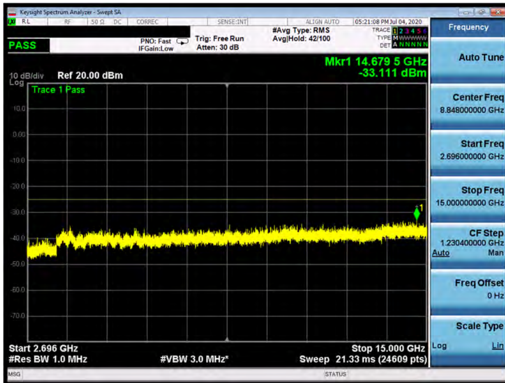
Plot 7-290. Conducted Spurious Plot (n41 - 100MHz DFT-s-OFDM-QPSK - RB Size 1, RB Offset 1 - Low Channel)
