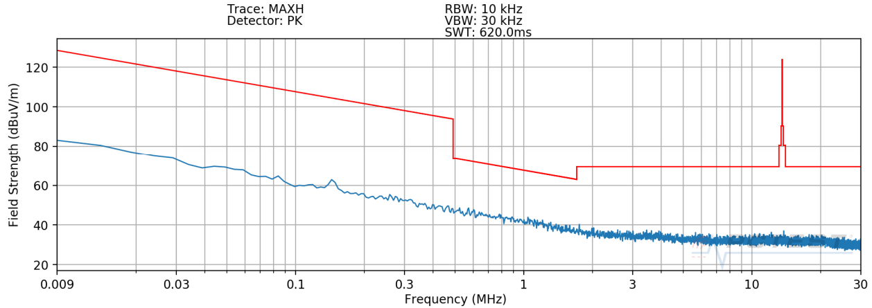
Plot 7-1. Radiated Spurious Plot 9kHz – 30MHz (Pol. X – Device to Device WPT)
