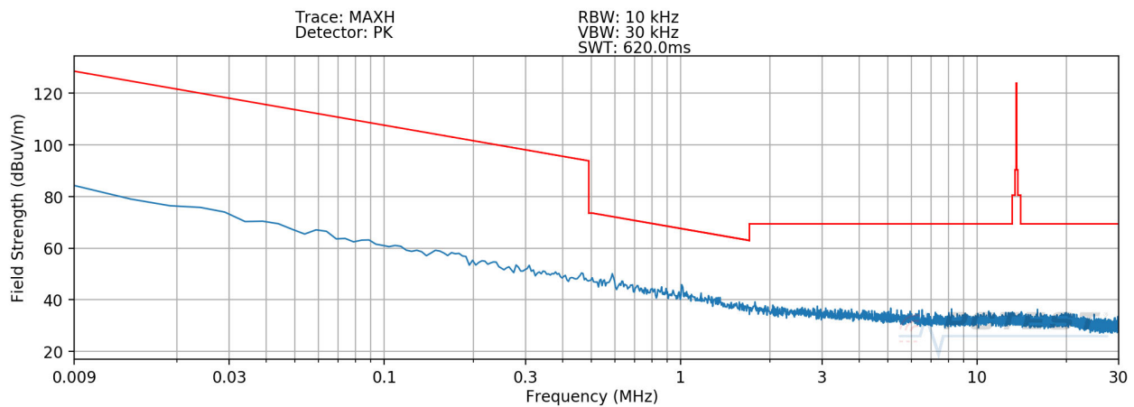
Plot 7-5. Radiated Spurious Plot 9kHz – 30MHz (Pol. Y – WPT - Device to S-Pen)
