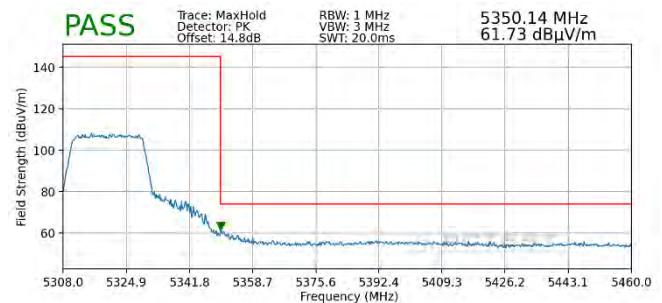
Plot 7-406. Radiated Upper Band Edge Plot MIMO (Peak – UNII Band 2A – 242 Tones)
