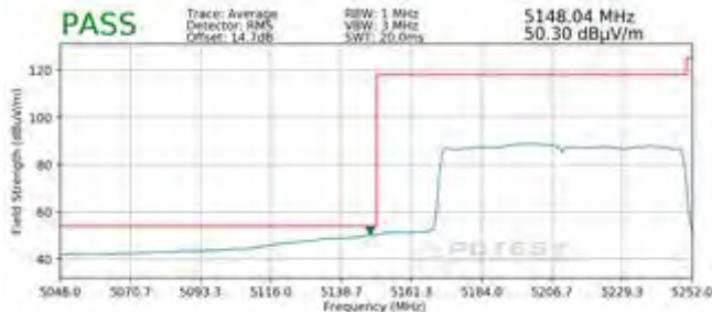
Plot 7-375. Radiated Lower Band Edge Plot SISO ANT1 (Average - UNII Band 1 - 996 Tones)
