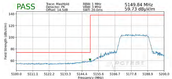
Plot 7-383. Radiated Lower Band Edge Plot SISO ANT2 (Peak - UNII Band 1 - 242 Tones)
