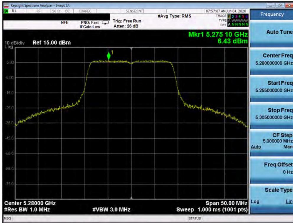
Plot 7-212. Power Spectral Density Plot SISO ANT2 (20MHz BW 802.11n (UNII Band 2A) – Ch. 56)
