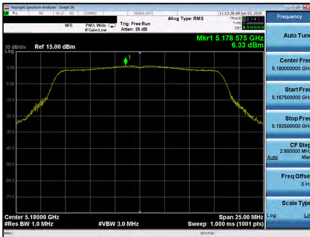
Plot 7-193. Power Spectral Density Plot SISO ANT2 (802.11a (UNII Band 1) – Ch. 36)
