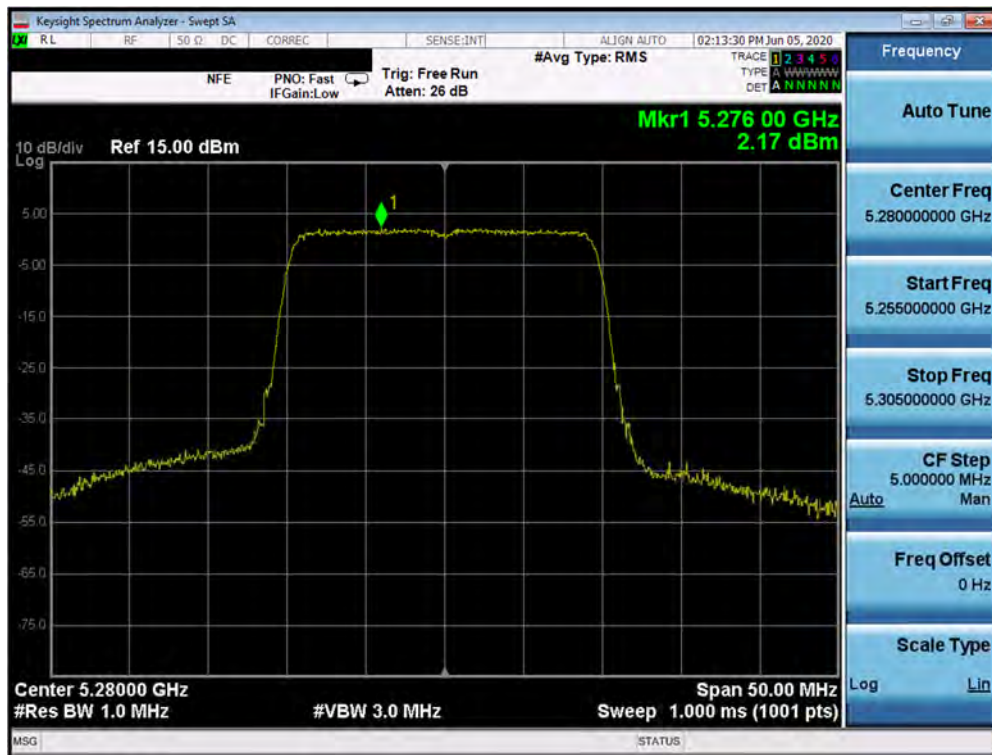
Plot 7-149. Power Spectral Density Plot SISO ANT1 (20MHz BW 802.11ax (UNII Band 2A) – Ch. 56)
