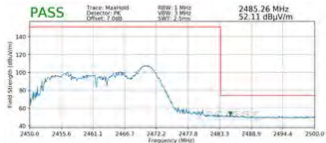
Plot 7-112. Radiated Restricted Upper Band Edge Measurement MIMO (Peak – 26 Tones)
