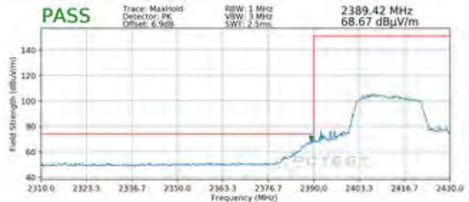
Plot 7-106. Radiated Restricted Lower Band Edge Measurement SISO ANT2 (Peak – 242 Tones)
