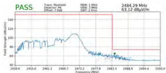
Plot 7-104. Radiated Restricted Upper Band Edge Measurement SISO ANT2 (Peak – 26 Tones)
