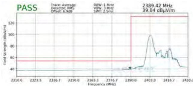
Plot 7-109. Radiated Restricted Lower Band Edge Measurement MIMO (Average – 26 Tones)
