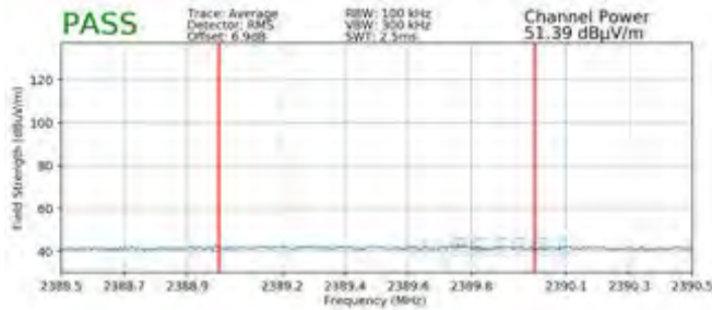
Plot 7-105. Radiated Restricted Lower Band Edge Measurement SISO ANT2 (Average – 242 Tones)
