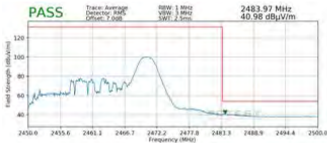
Plot 7-95. Radiated Restricted Upper Band Edge Measurement SISO ANT1 (Average - 26 Tones)
