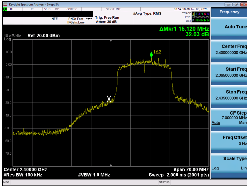
Plot 7-63. Band Edge Plot SISO ANT1 (802.11ax (2.4GHz) – Ch. 1)
