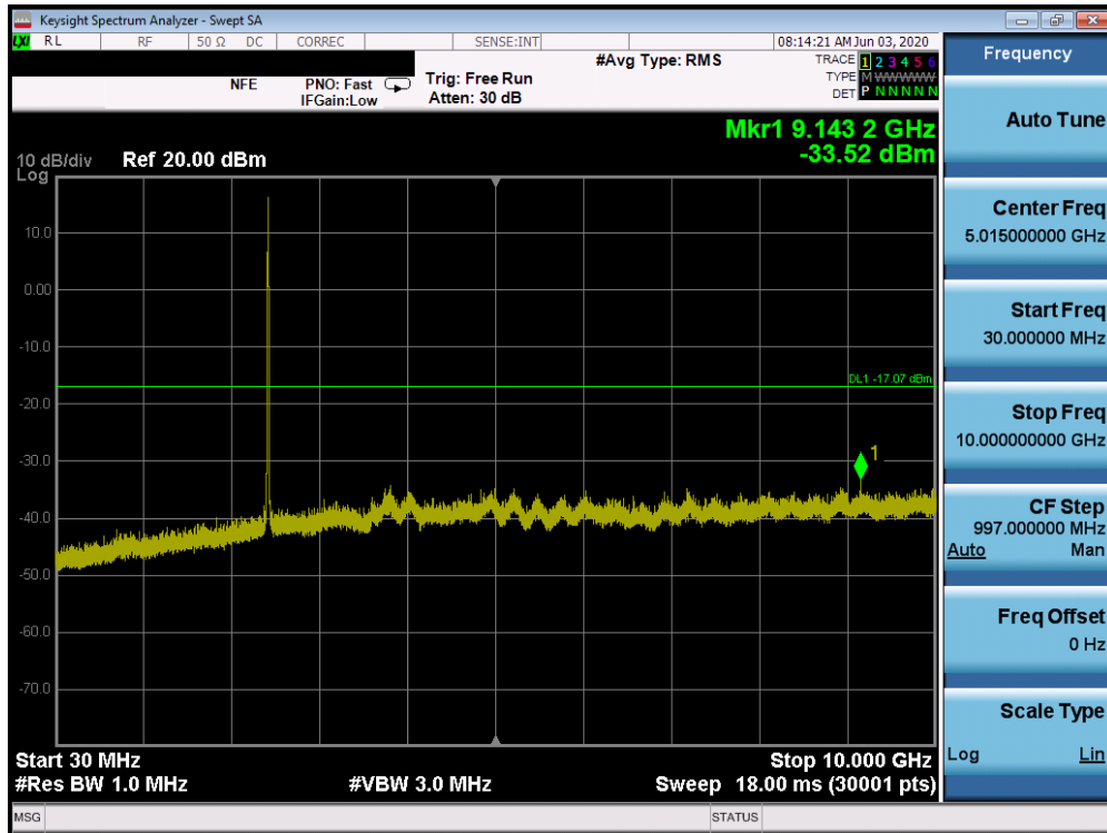
Plot 7-73. Conducted Spurious Plot SISO ANT2 (802.11b – Ch. 6)
