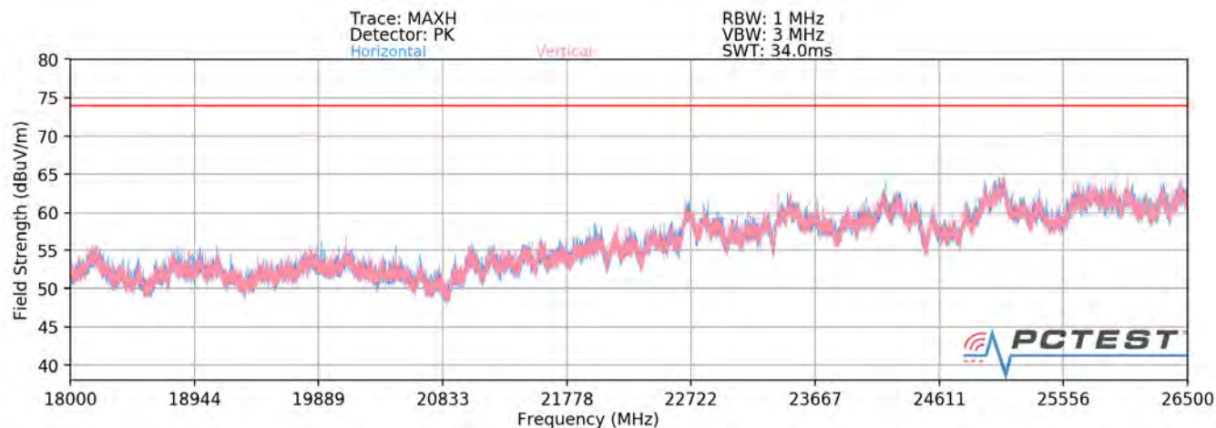
Plot 7-80. Radiated Spurious Plot above 18GHz SISO ANT1
