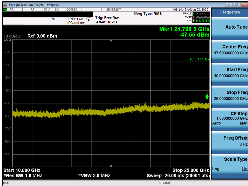
Plot 7-74. Conducted Spurious Plot SISO ANT2 (802.11b – Ch. 6)
