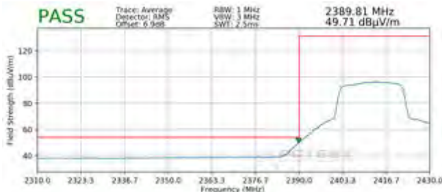
Plot 7-88. Radiated Restricted Lower Band Edge Measurement SISO ANT1 (Average)
