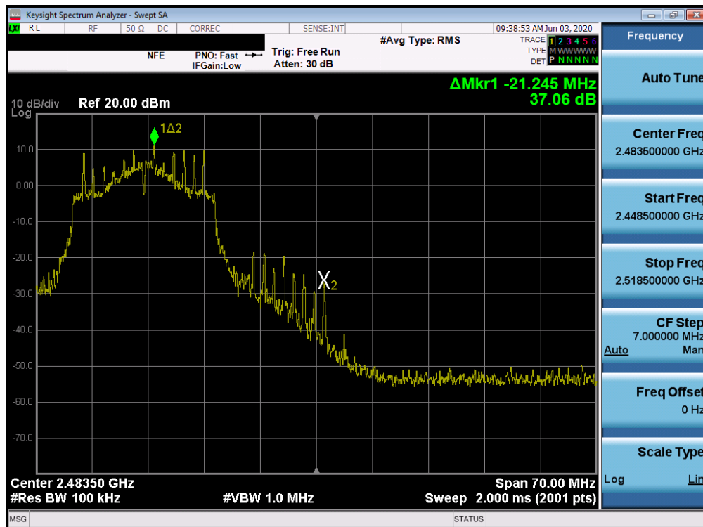
Plot 7-62. Band Edge Plot SISO ANT2 (802.11n (2.4GHz) – Ch. 11)
