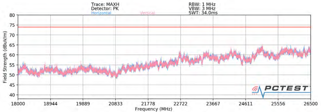
Plot 7-84. Radiated Spurious Plot above 18GHz SISO ANT2
