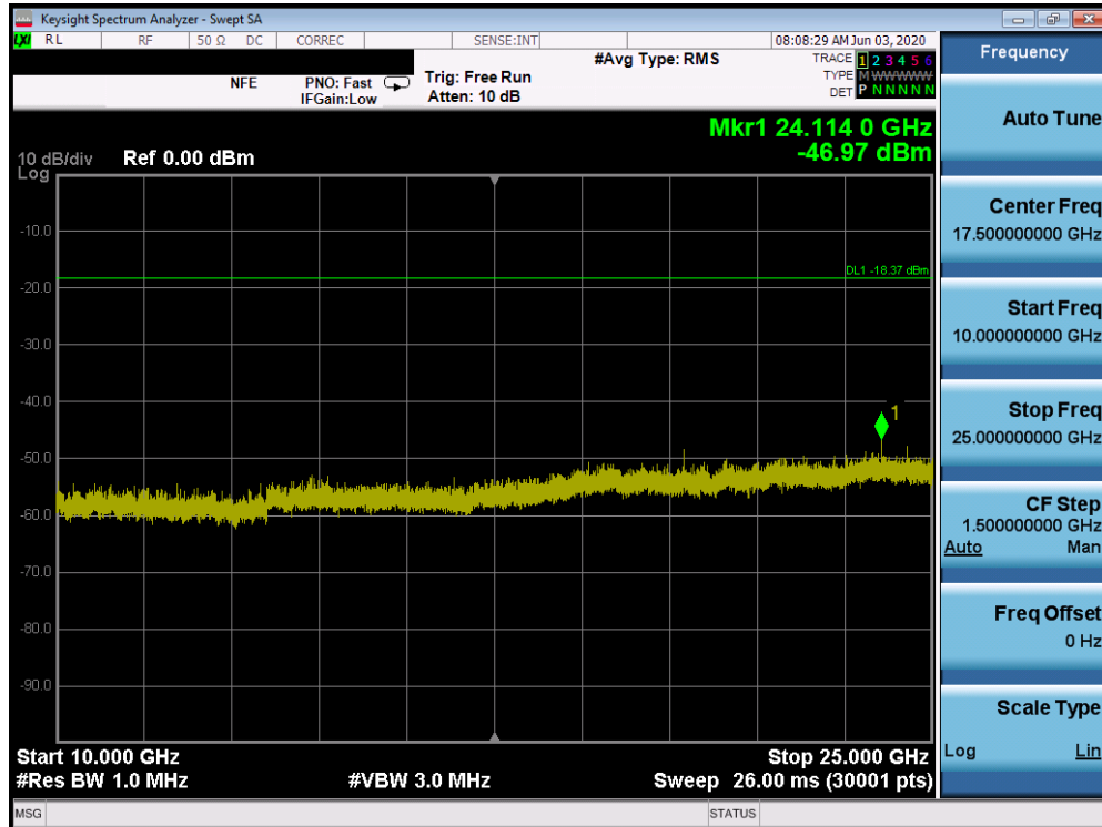
Plot 7-72. Conducted Spurious Plot SISO ANT2 (802.11b – Ch. 1)
