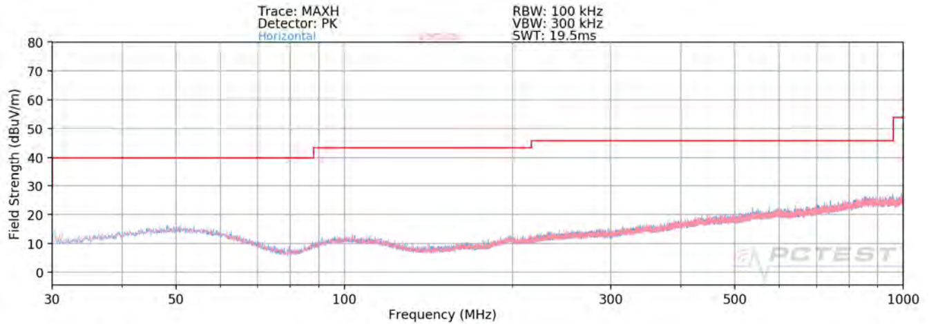
Plot 7-102. Radiated Spurious Plot below 1GHz MIMO
