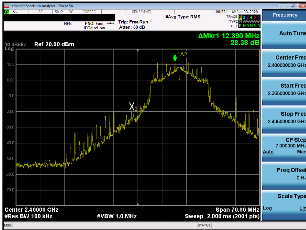
Plot 7-59. Band Edge Plot SISO ANT2 (802.11g- Ch. 1)
