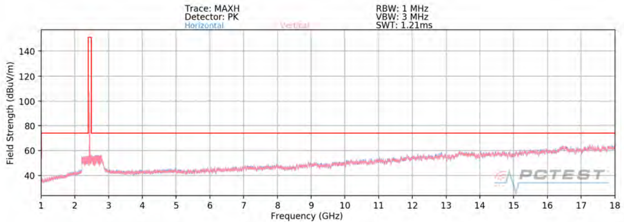
Plot 7-82. Radiated Spurious Plot above 1GHz SISO ANT2 (802.11b – Ch. 6)
