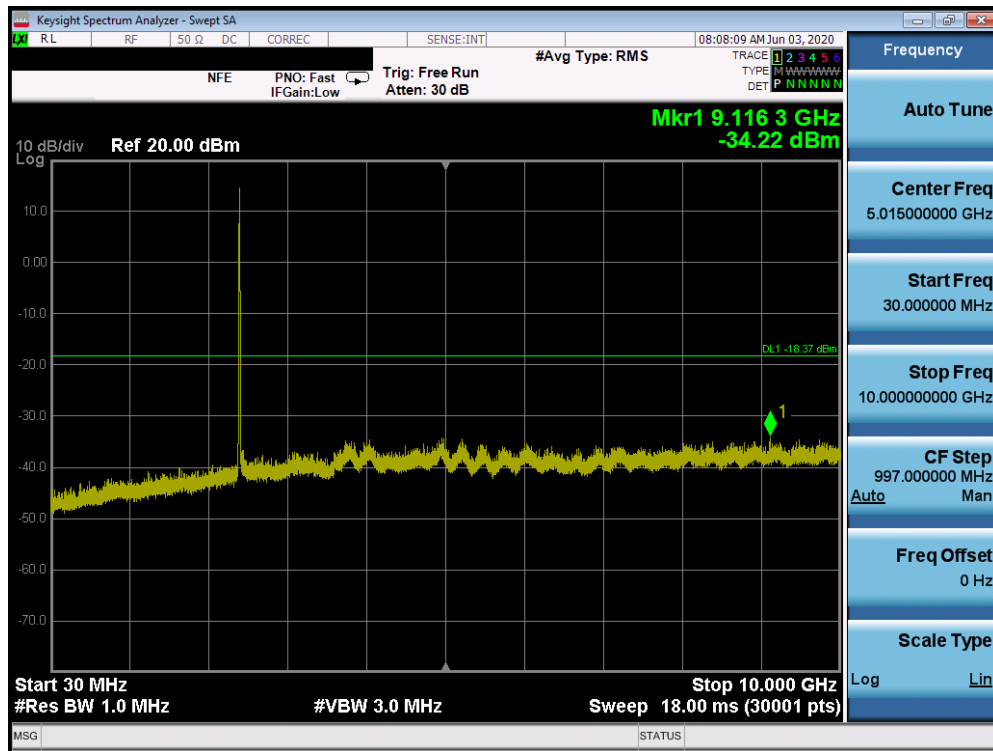
Plot 7-71. Conducted Spurious Plot SISO ANT2 (802.11b – Ch. 1)
