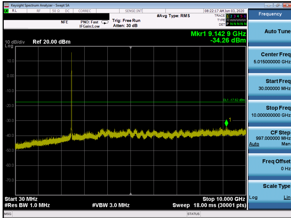
Plot 7-75. Conducted Spurious Plot SISO ANT2 (802.11b – Ch. 11)
