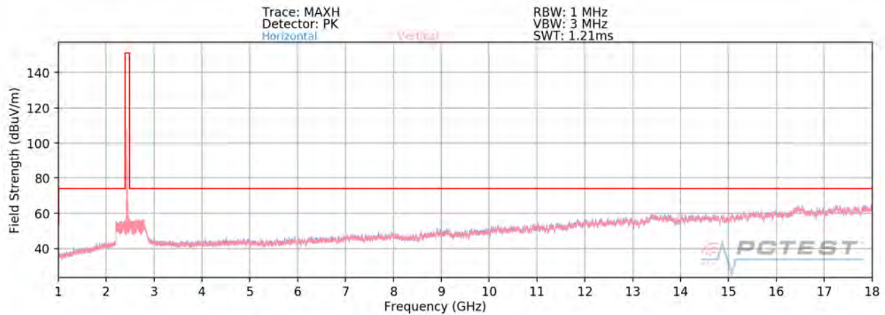
Plot 7-78. Radiated Spurious Plot above 1GHz SISO ANT1 (802.11b – Ch. 6)
