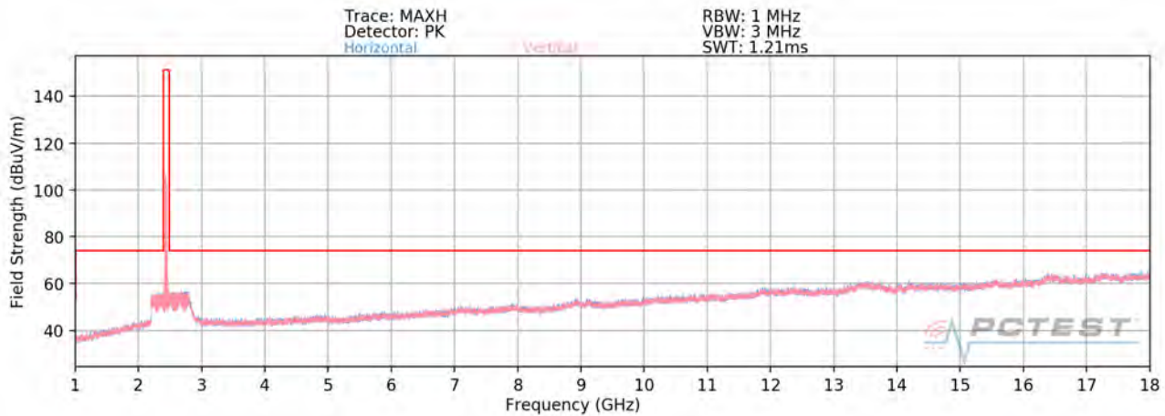
Plot 7-86. Radiated Spurious Plot above 1GHz MIMO/CDD (802.11g – Ch. 6)
