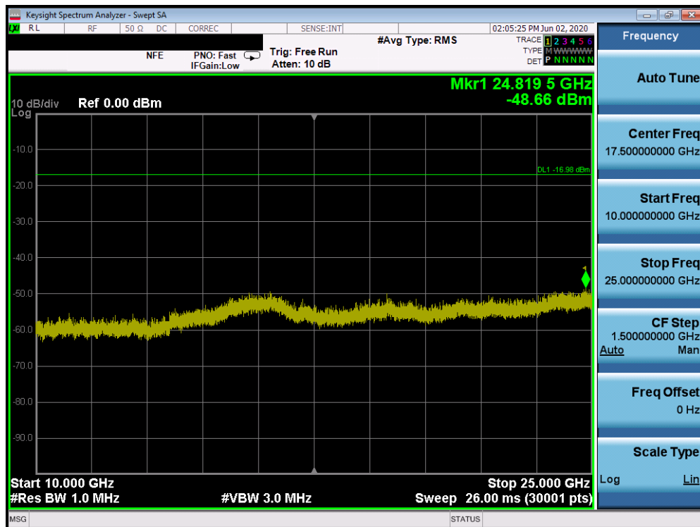
Plot 7-70. Conducted Spurious Plot SISO ANT1 (802.11b – Ch. 11)
