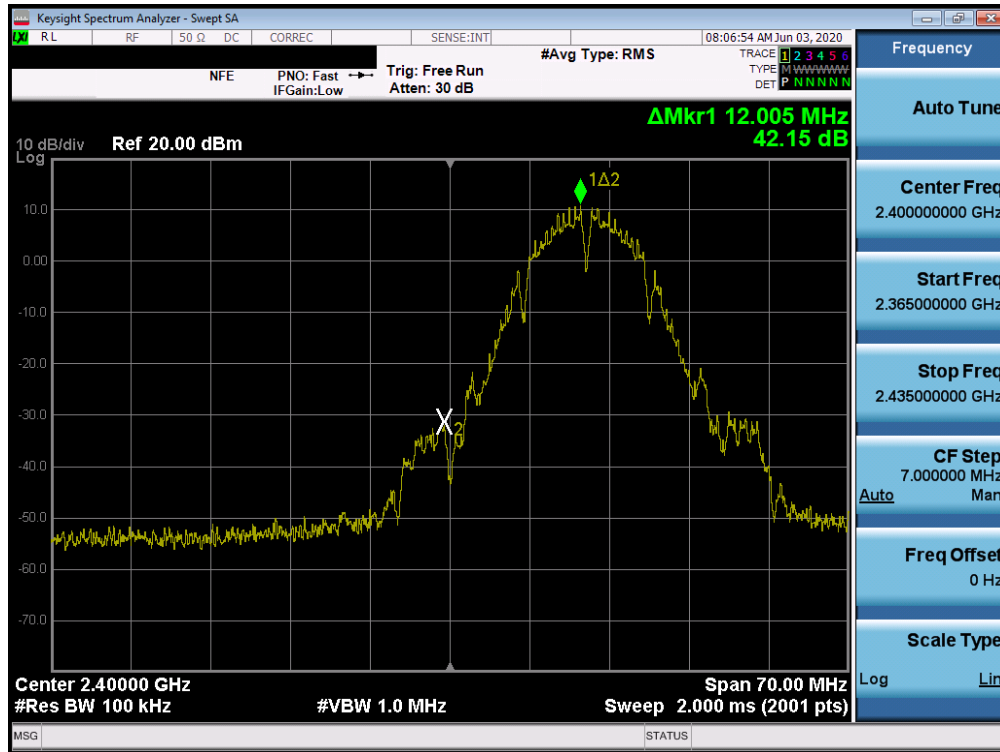
Plot 7-57. Band Edge Plot SISO ANT2 (802.11b - Ch. 1)
