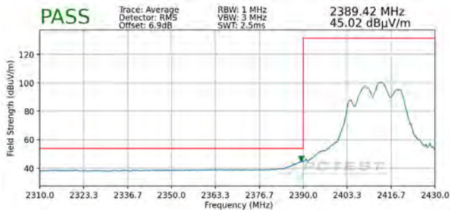
Plot 7-96. Radiated Restricted Lower Band Edge Measurement CDD (Average)
