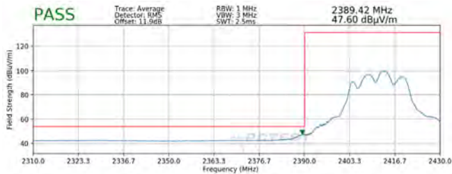
Plot 7-100. Radiated Restricted Band Edge Measurement MIMO with WCP (Average)
