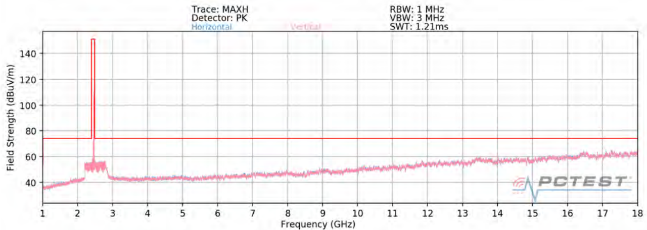
Plot 7-79. Radiated Spurious Plot above 1GHz SISO ANT1 (802.11b – Ch. 11)
