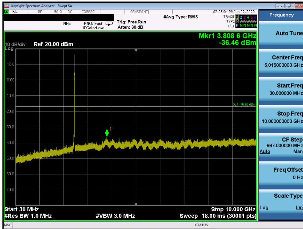
Plot 7-69. Conducted Spurious Plot SISO ANT1 (802.11b – Ch. 11)
