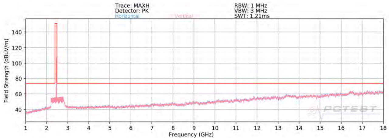
Plot 7-83. Radiated Spurious Plot above 1GHz SISO ANT2 (802.11b – Ch. 11)
