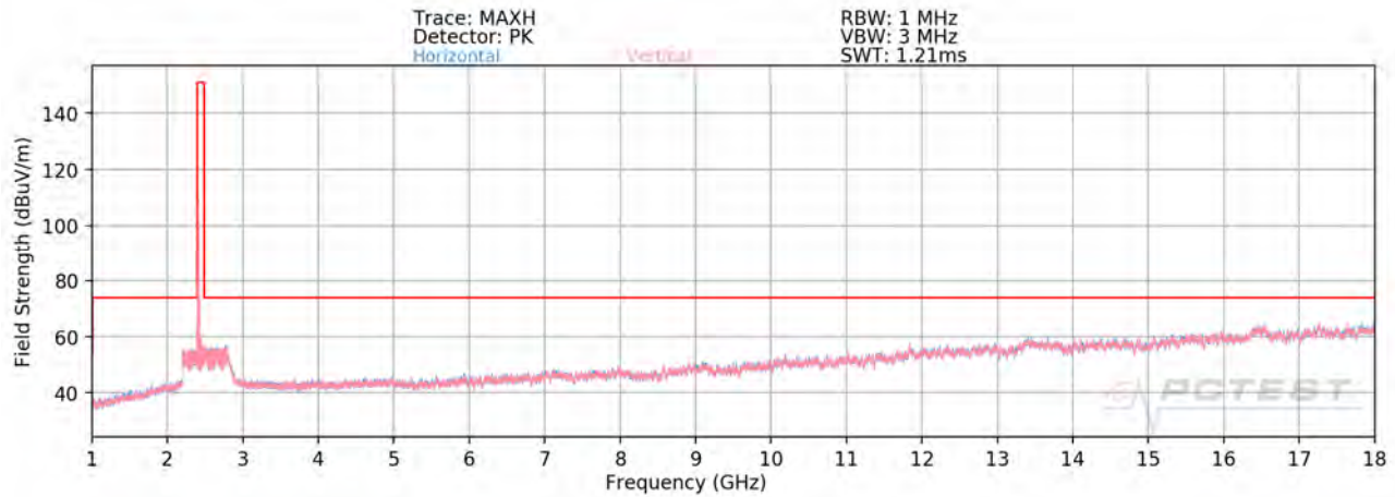
Plot 7-77. Radiated Spurious Plot above 1GHz SISO ANT1 (802.11b – Ch. 1)
