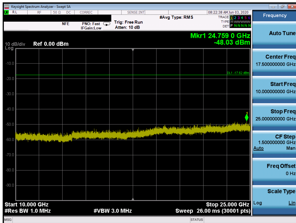
Plot 7-76. Conducted Spurious Plot SISO ANT2 (802.11b – Ch. 11)
