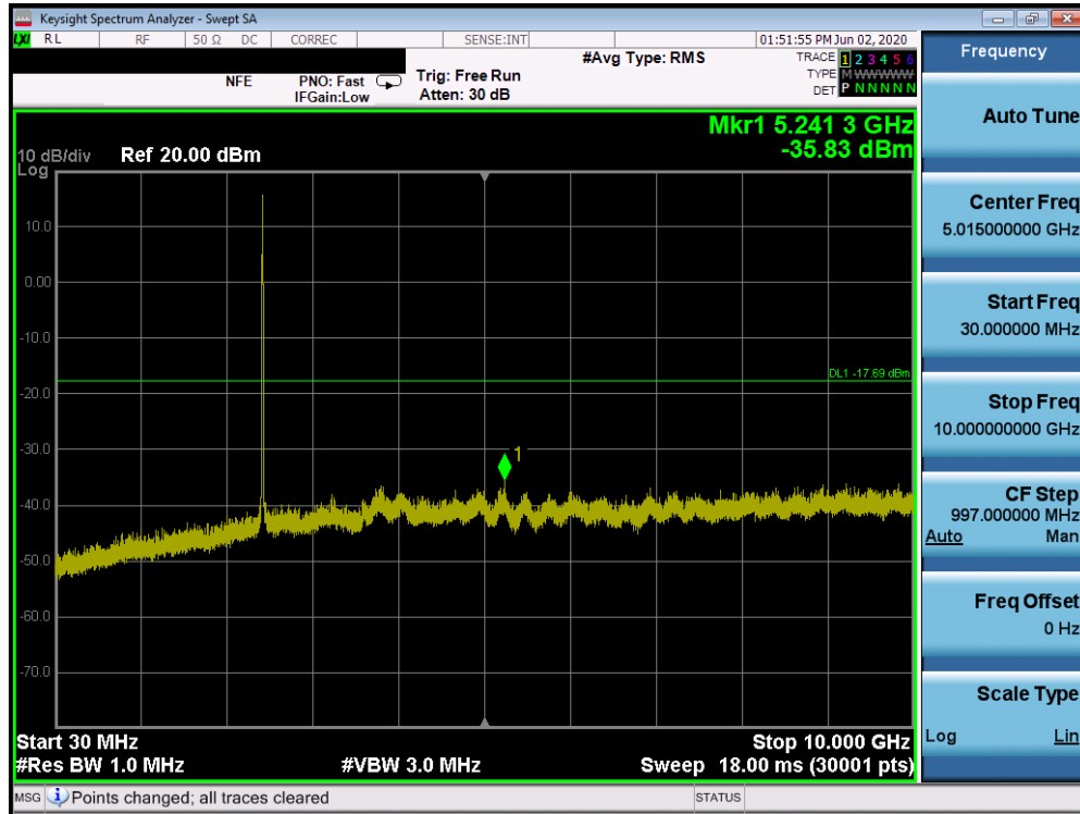
Plot 7-67. Conducted Spurious Plot SISO ANT1 (802.11b – Ch. 6)
