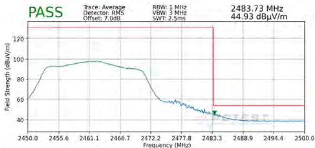
Plot 7-98. Radiated Restricted Upper Band Edge Measurement MIMO (Average)
