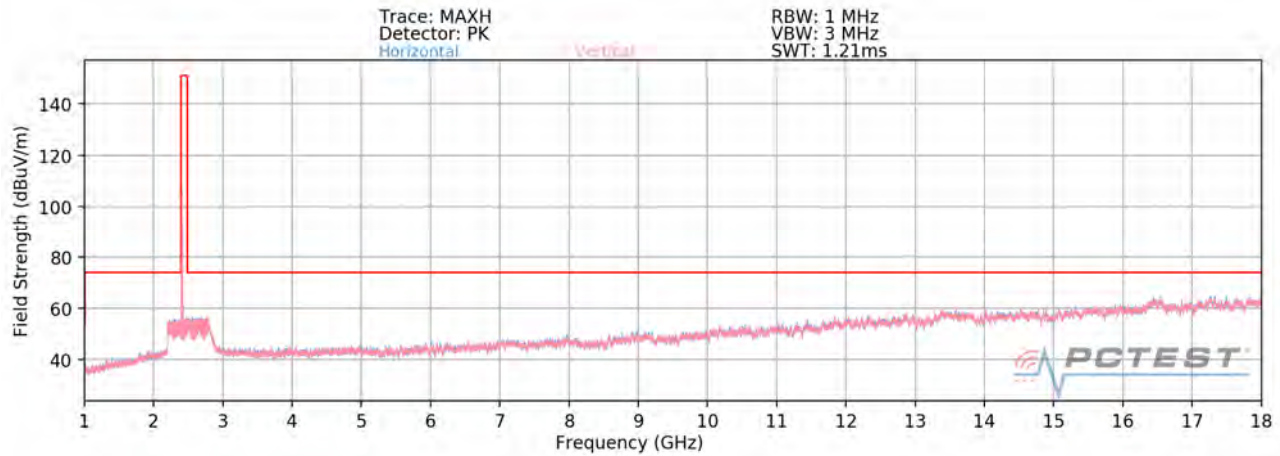
Plot 7-81. Radiated Spurious Plot above 1GHz SISO ANT2 (802.11b – Ch. 1)
