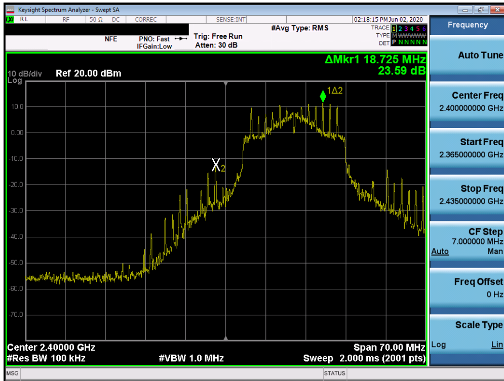
Plot 7-53. Band Edge Plot SISO ANT1 (802.11n (2.4GHz) – Ch. 1)
