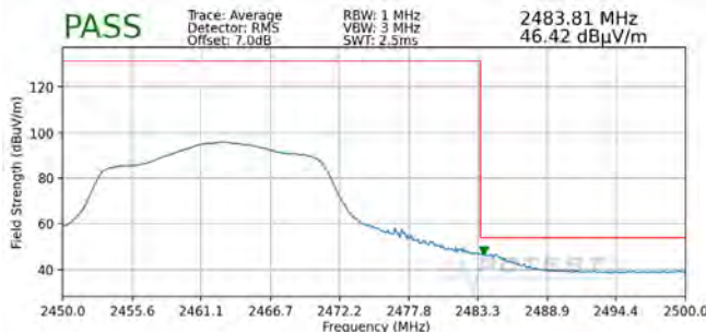
Plot 7-94. Radiated Restricted Upper Band Edge Measurement SISO ANT2 (Average)
