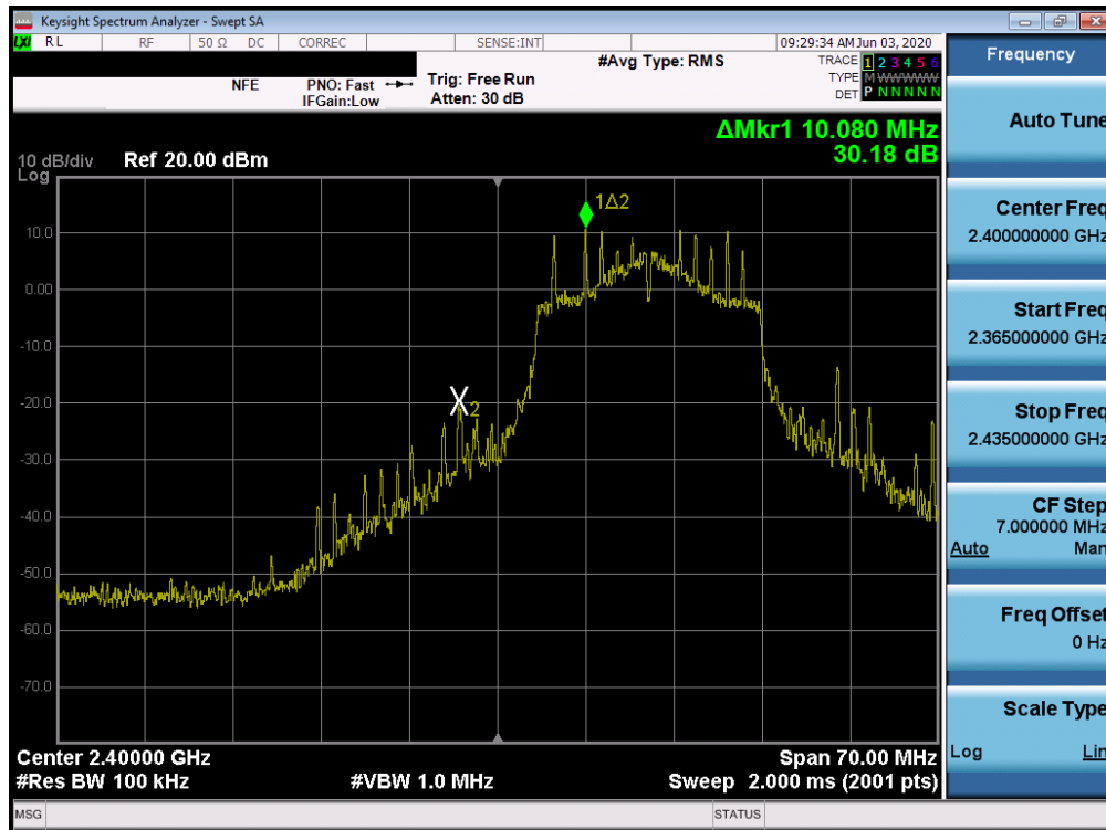
Plot 7-61. Band Edge Plot SISO ANT2 (802.11n (2.4GHz) – Ch. 1)
