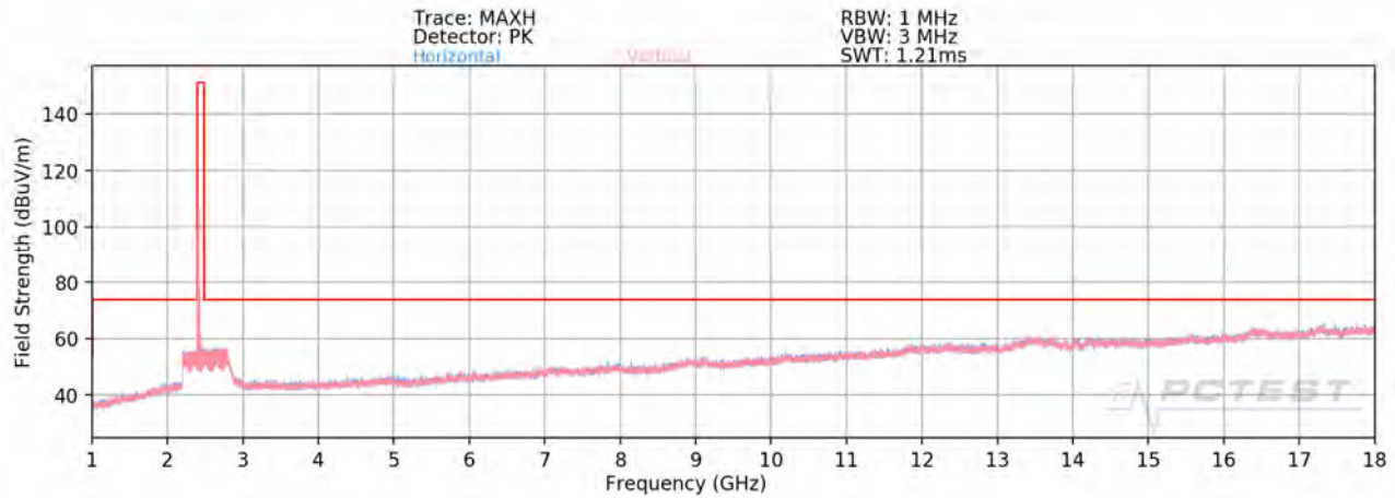
Plot 7-85. Radiated Spurious Plot above 1GHz MIMO/CDD (802.11g – Ch. 1)
