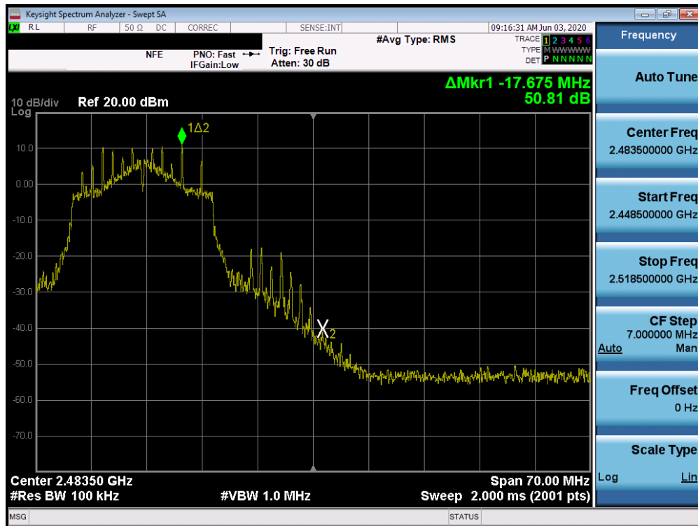
Plot 7-64. Band Edge Plot SISO ANT1 (802.11ax (2.4GHz) – Ch. 11)
