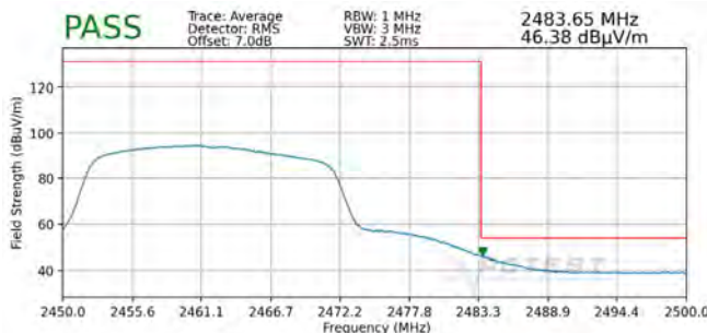
Plot 7-90. Radiated Restricted Upper Band Edge Measurement SISO ANT1 (Average)
