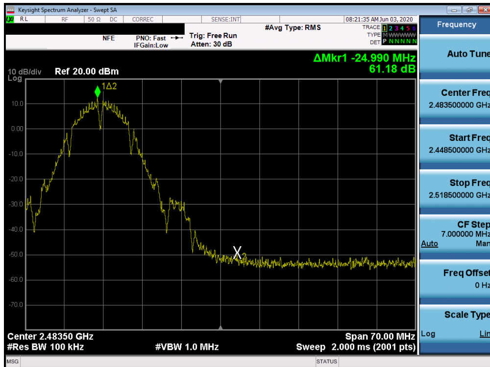
Plot 7-58. Band Edge Plot SISO ANT2 (802.11b - Ch. 11)
