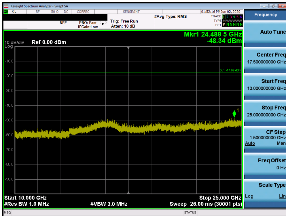
Plot 7-68. Conducted Spurious Plot SISO ANT1 (802.11b – Ch. 6)
