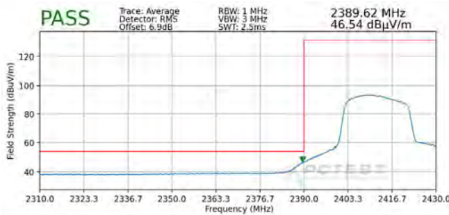
Plot 7-92. Radiated Restricted Lower Band Edge Measurement SISO ANT2 (Average)
