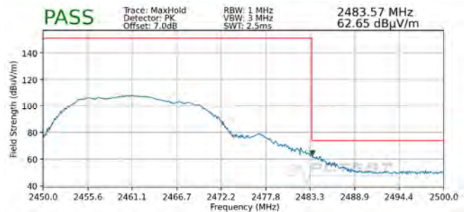
Plot 7-91. Radiated Restricted Upper Band Edge Measurement SISO ANT1 (Peak)
