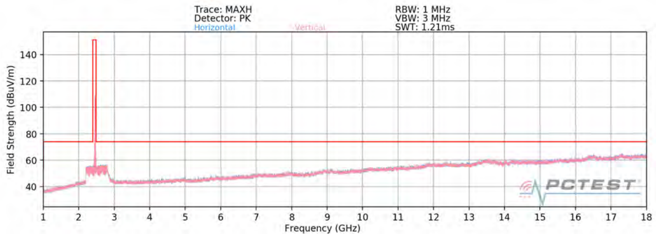
Plot 7-87. Radiated Spurious Plot above 1GHz MIMO/CDD (802.11g – Ch. 11)
