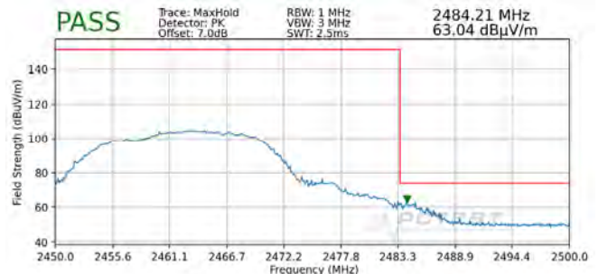
Plot 7-95. Radiated Restricted Upper Band Edge Measurement SISO ANT2 (Peak)
