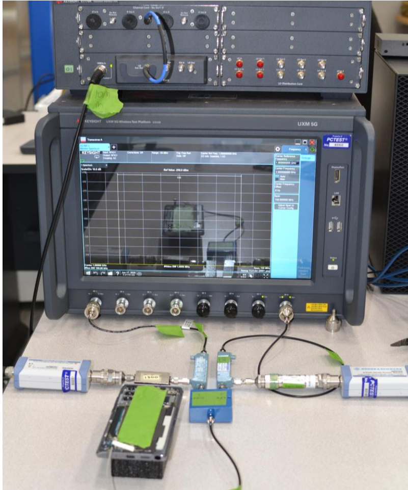
Test Setup Photo 3 – Conducted Test Setup (Figure 5-1c)
