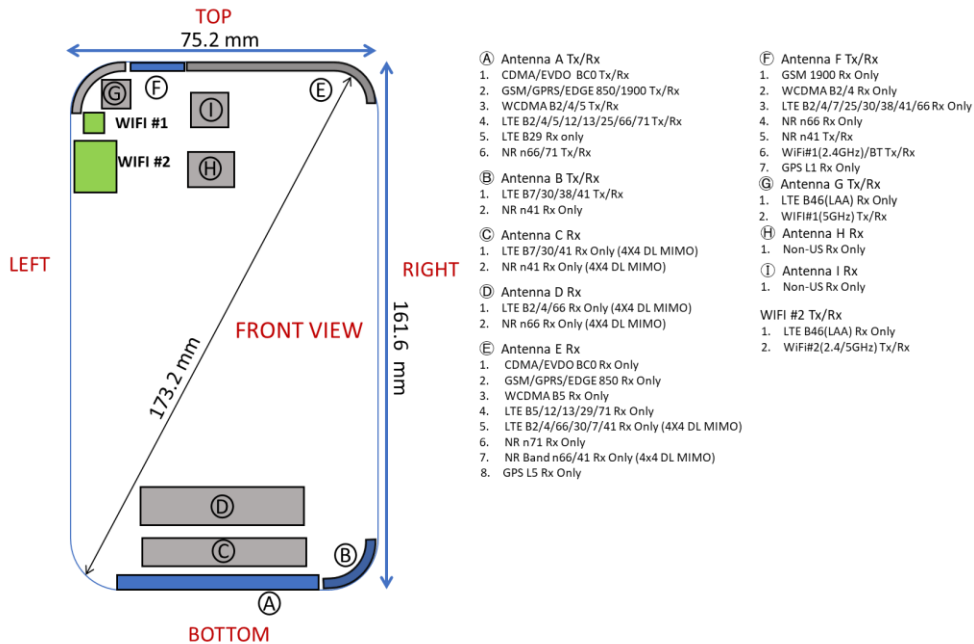
Figure E-1 DUT Antenna Locations
