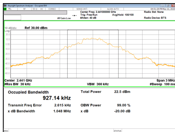
20 dB Bandwidth MID CHANNEL
