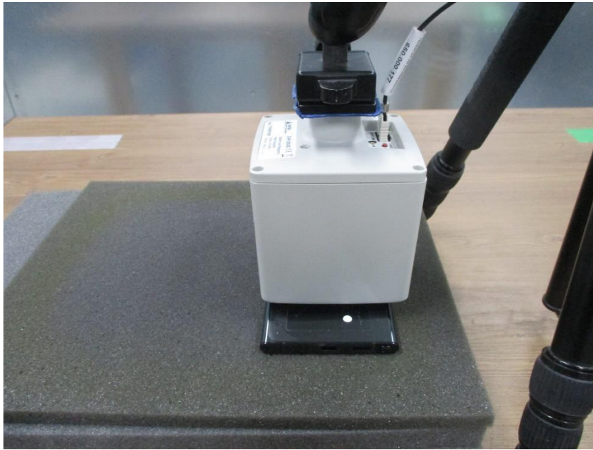
Rear
