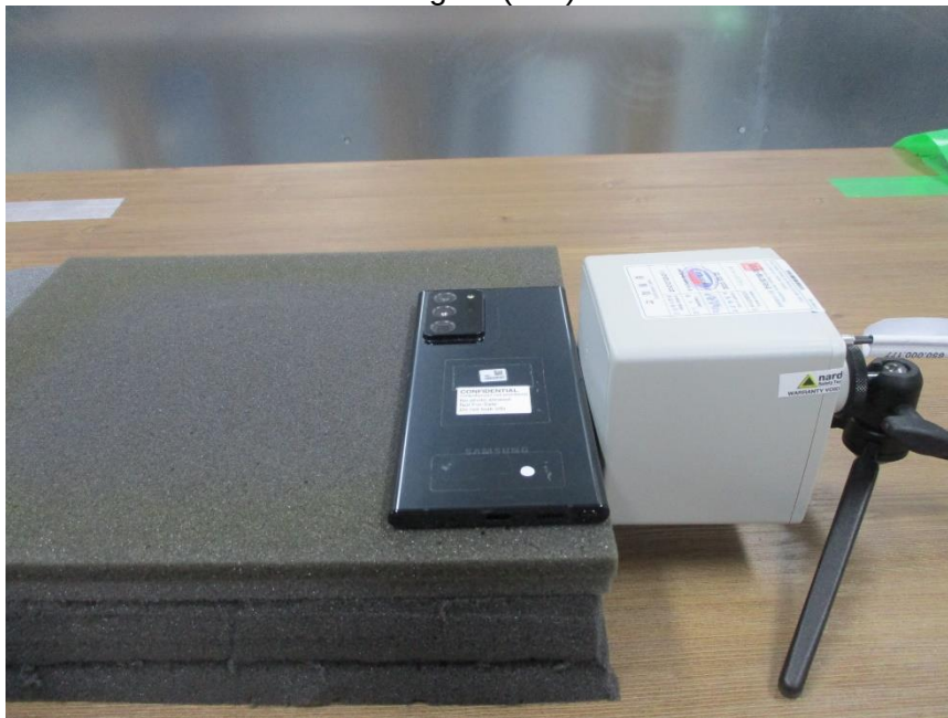
Edge 4 (Left)
