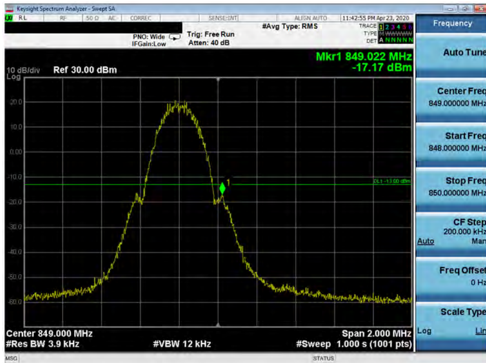
Plot 7-34. Band Edge Plot (CELL GPRS Mode - High Channel)
