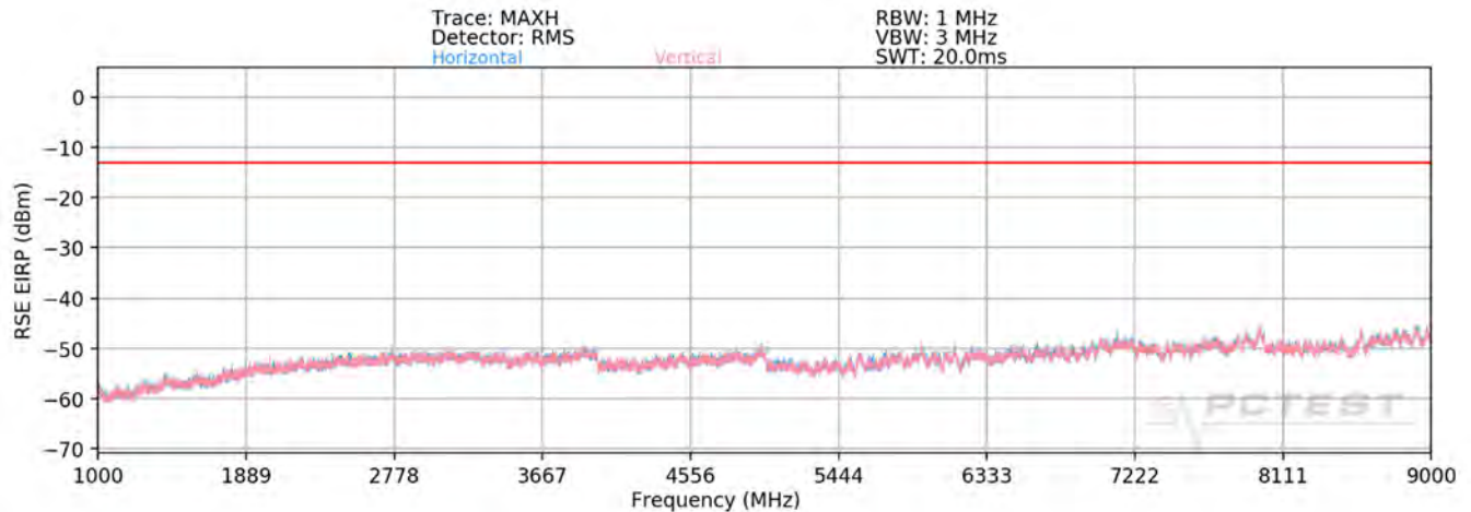
Plot 7-48. Radiated Spurious Plot above 1GHz (Cellular WCDMA Mode)
