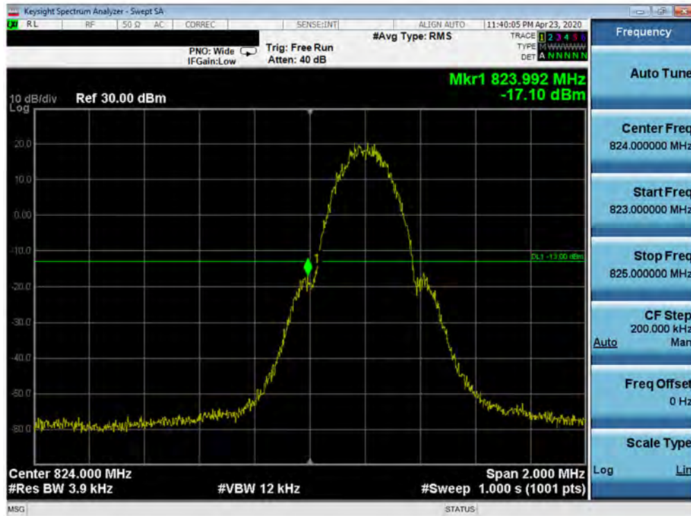
Plot 7-33. Band Edge Plot (CELL GPRS Mode - Low Channel)
