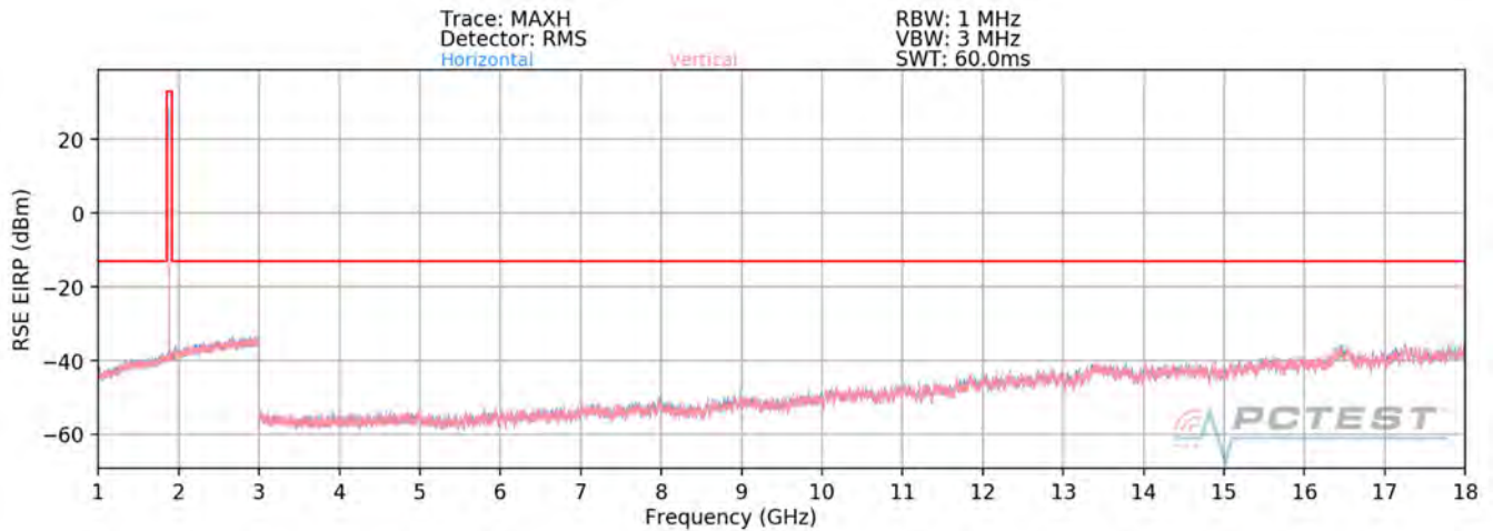
Plot 7-47. Radiated Spurious Plot above 1GHz (PCS GPRS Mode)
