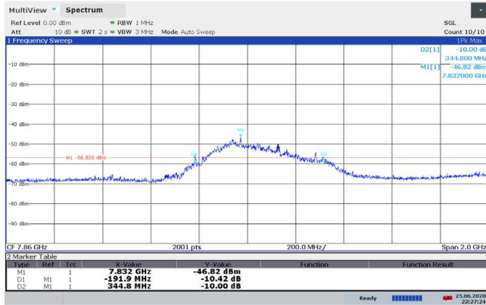
Plot 7-17. BANDWIDTH Plot - ANT1 - CH.9 – SP1 – Preamble 11
