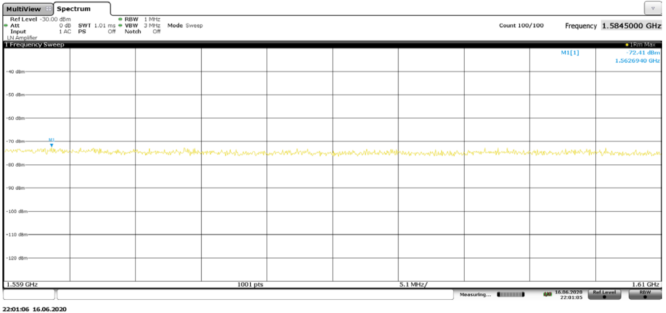
Plot 7-58. Radiated Spurious Pre-Scan 1559 - 1610 MHz - CH.9 - ANT 1
