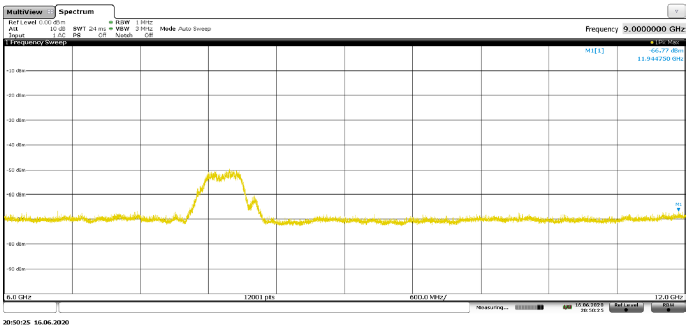
Plot 7-59. Radiated Spurious Pre-Scan 6000 - 12000 MHz - CH.9 - ANT 1
