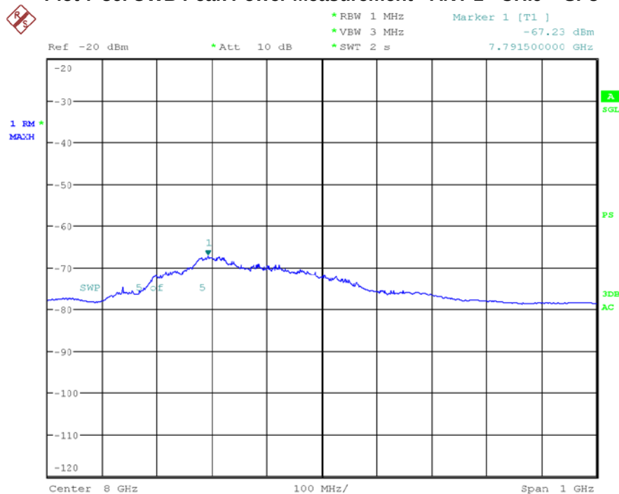
Plot 7-36. UWB Peak Power Measurement - ANT 1 - CH.9 – SP3 – BPRF
