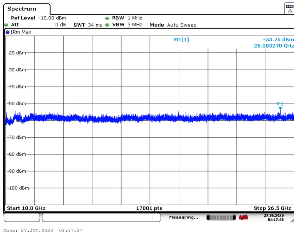
Plot 7-68. Radiated Spurious Pre-Scan 18 - 26.5 GHz - CH.9 - ANT 2
