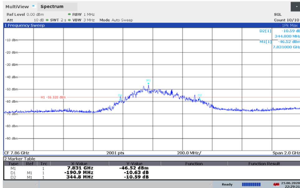
Plot 7-16. BANDWIDTH Plot – ANT2 - CH.9 - SP0 – Preamble 11
