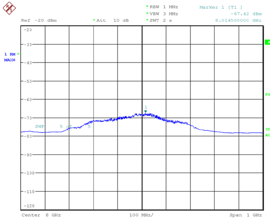
Plot 7-54. UWB Peak Power Measurement - ANT 2 - CH.9 – SP3 – HPRF
