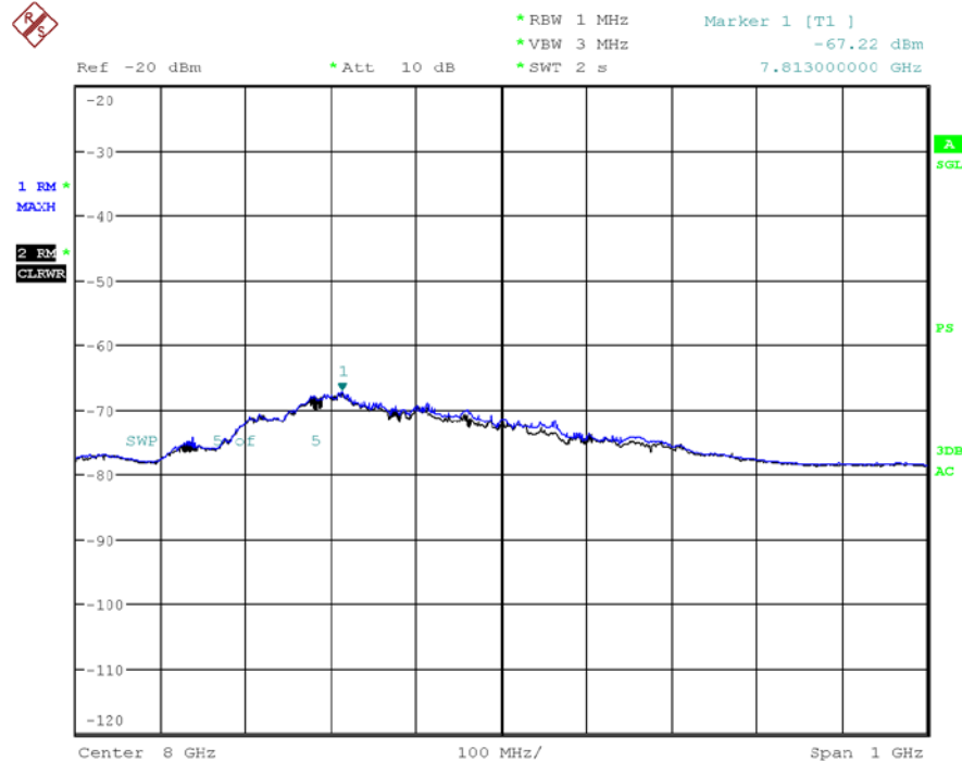
Plot 7-42. UWB Peak Power Measurement - ANT 2 - CH.9 – SP3 – BPRF
