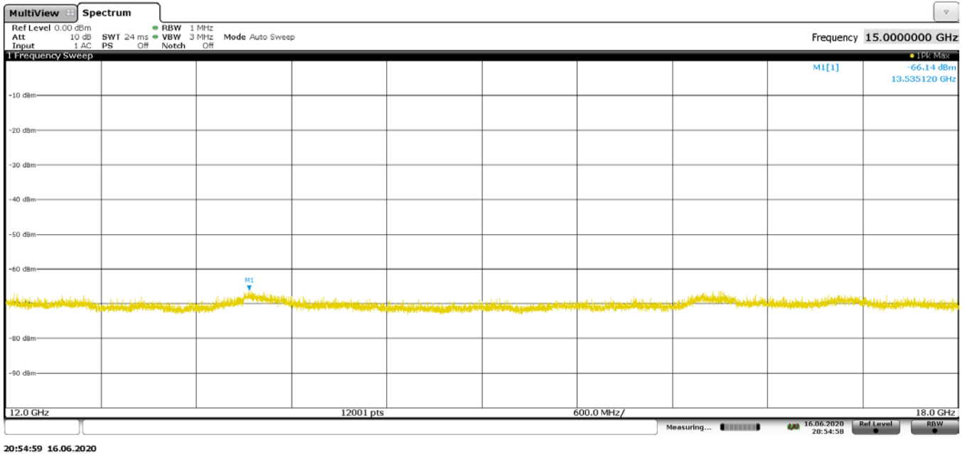
Plot 7-67. Radiated Spurious Pre-Scan 12000 - 18000 MHz - CH.9 - ANT 2
