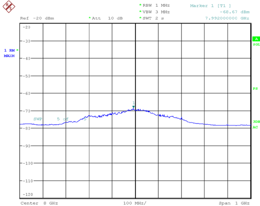
Plot 7-32. UWB Peak Power Measurement - ANT 1 - CH.9 - SP0 – BPRF
