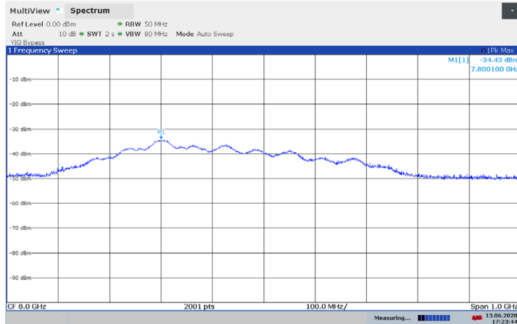
Plot 7-42. UWB Peak Power Measurement - ANT 2 - CH.9 – SP3 – BPRF
