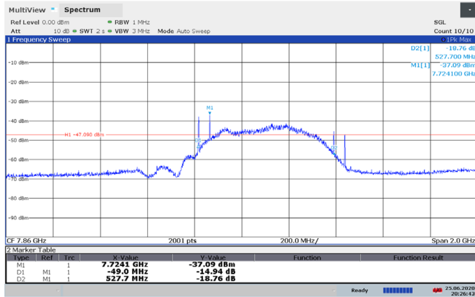
Plot 7-3. BANDWIDTH Plot - ANT1 - CH.9 – SP3 – Preamble 9
