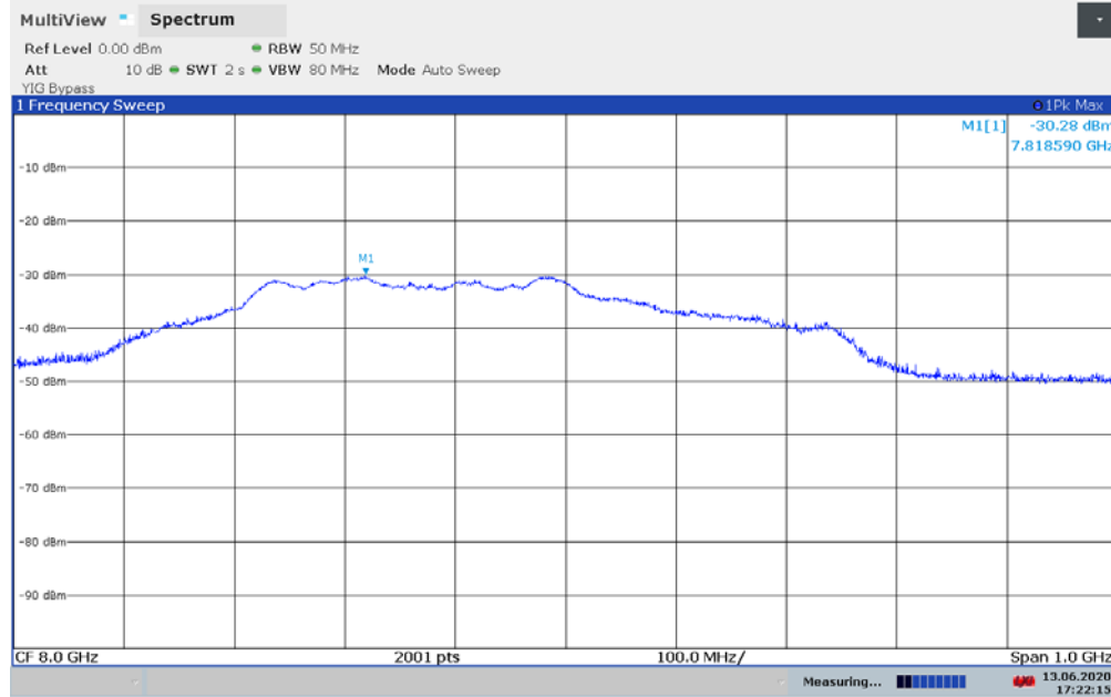
Plot 7-40. UWB Peak Power Measurement - ANT 2 - CH.9 – SP1 – BPRF
