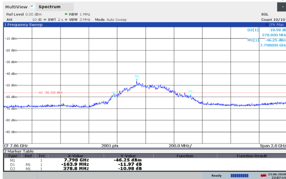
Plot 7-22. BANDWIDTH Plot 7-- ANT2 - CH.9 - SP0 – Preamble 12
