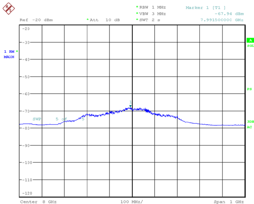
Plot 7-52. UWB Peak Power Measurement - ANT 2 - CH.9 – SP1 – HPRF
