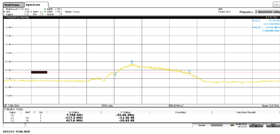
Plot 7-6. BANDWIDTH Plot – AN2 - CH.9 – SP3 – Preamble 9
