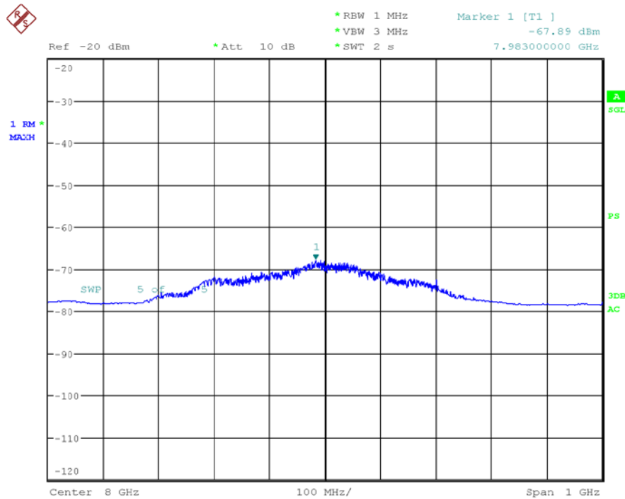
Plot 7-50. UWB Peak Power Measurement - ANT 2 - CH.9 - SP0 – HPRF
