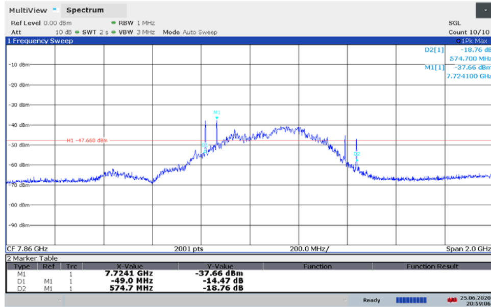
Plot 7-19. BANDWIDTH Plot 7-- ANT1 - CH.9 - SP0 – Preamble 12
