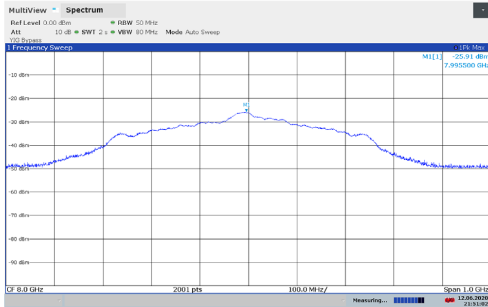
Plot 7-32. UWB Peak Power Measurement - ANT 1 - CH.9 - SP0 – BPRF
