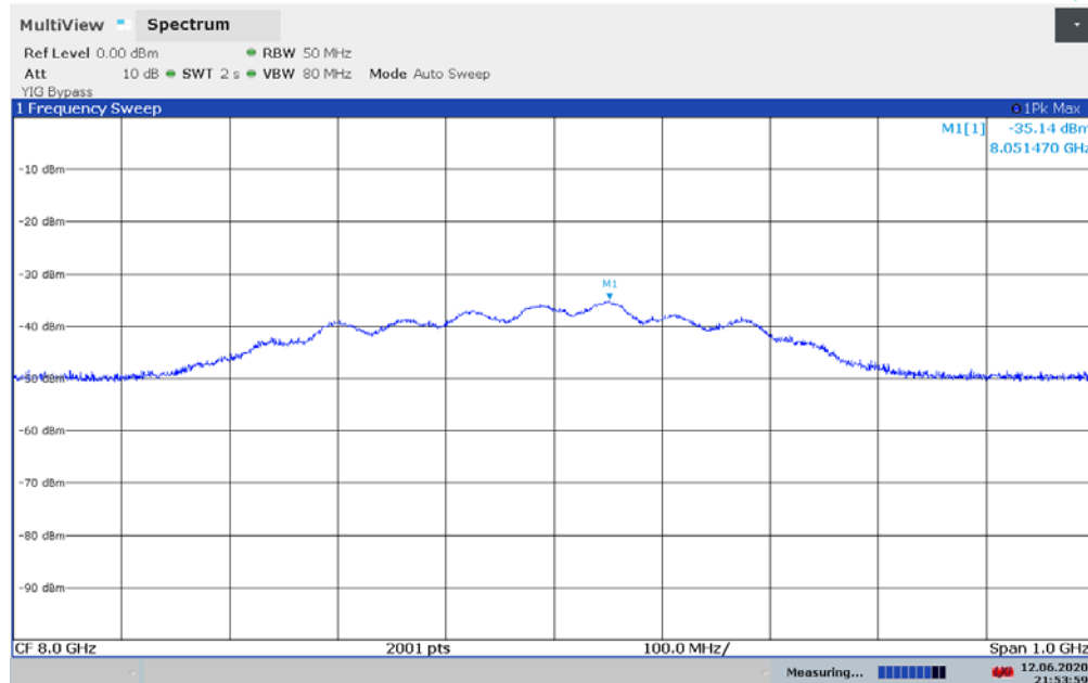
Plot 7-36. UWB Peak Power Measurement - ANT 1 - CH.9 – SP3 – BPRF
