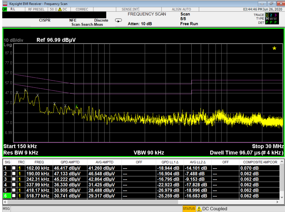
Plot 7-72. Line Conducted Plot (L1)
