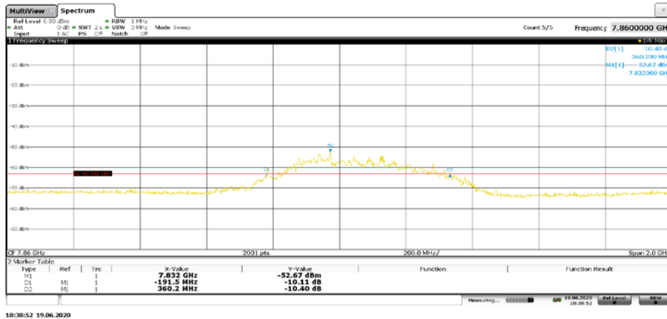
Plot 7-4. BANDWIDTH Plot – ANT2 - CH.9 - SP0 – Preamble 9
