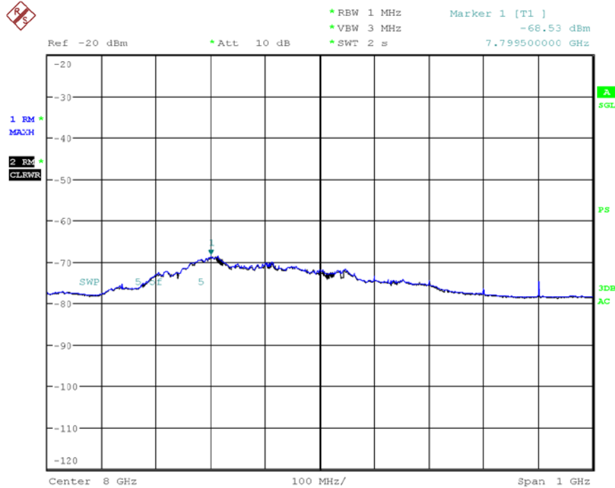
Plot 7-40. UWB Peak Power Measurement - ANT 2 - CH.9 – SP1 – BPRF
