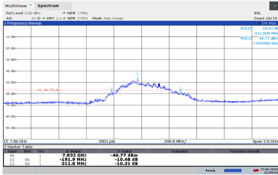
Plot 7-23. BANDWIDTH Plot – ANT2 - CH.9 – SP1 – Preamble 12
