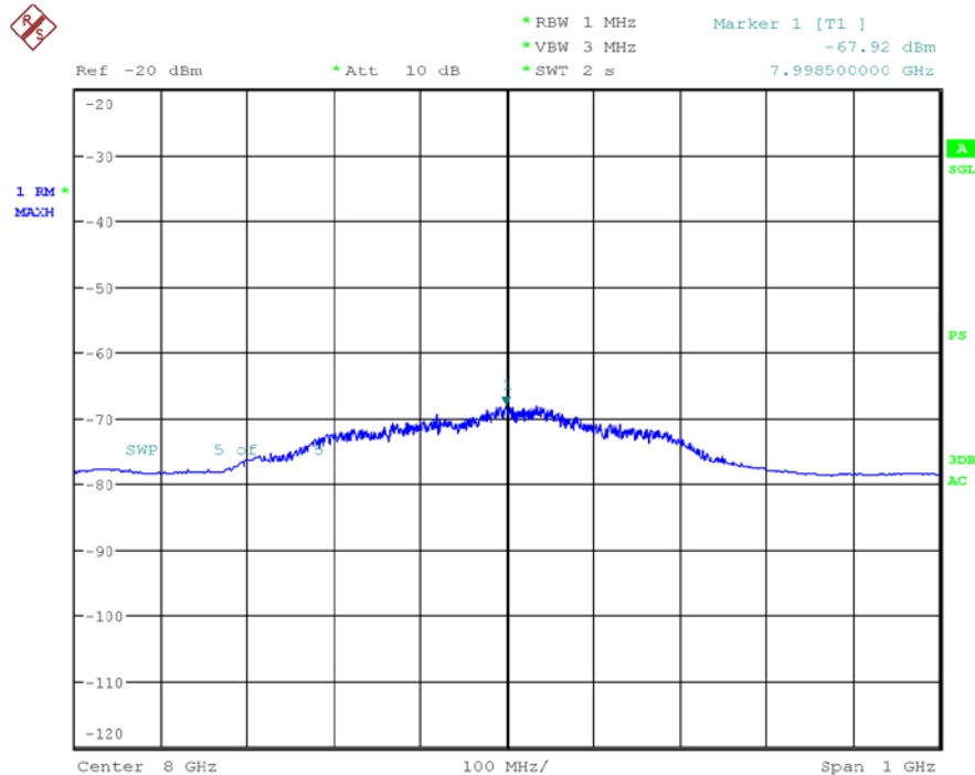
Plot 7-44. UWB Peak Power Measurement - ANT 1 - CH.9 - SP0 – HPRF
