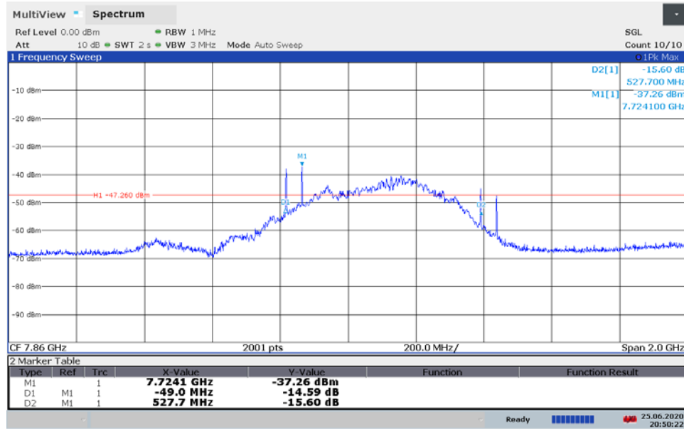
Plot 7-13. BANDWIDTH Plot - ANT1 - CH.9 - SP0 – Preamble 11
