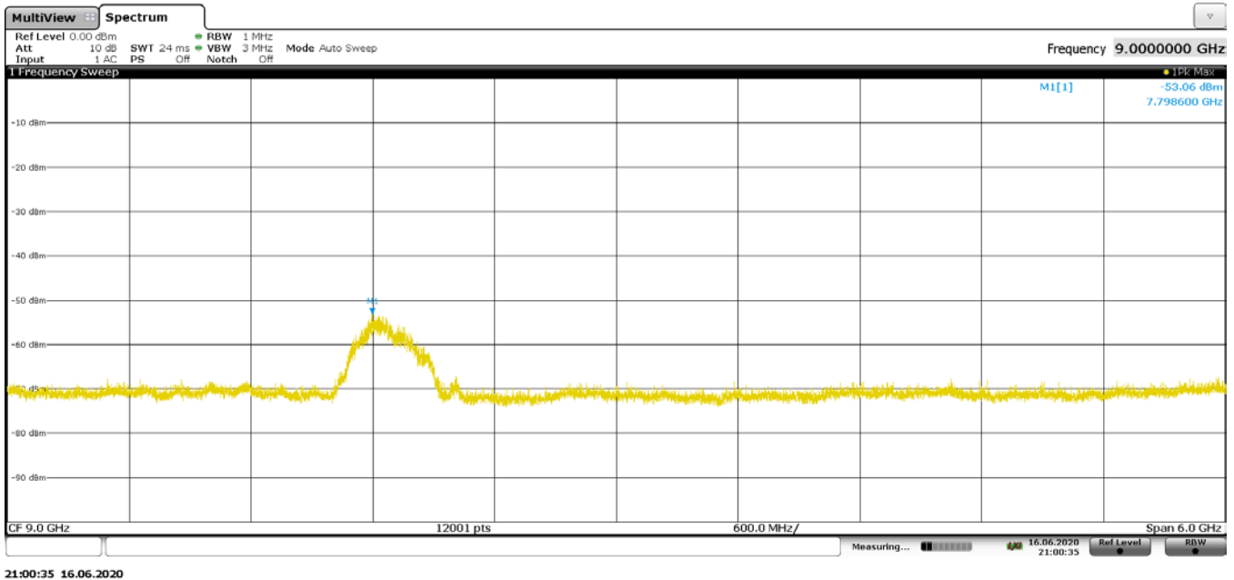
Plot 7-66. Radiated Spurious Pre-Scan 6000 - 12000 MHz - CH.9 - ANT 2
