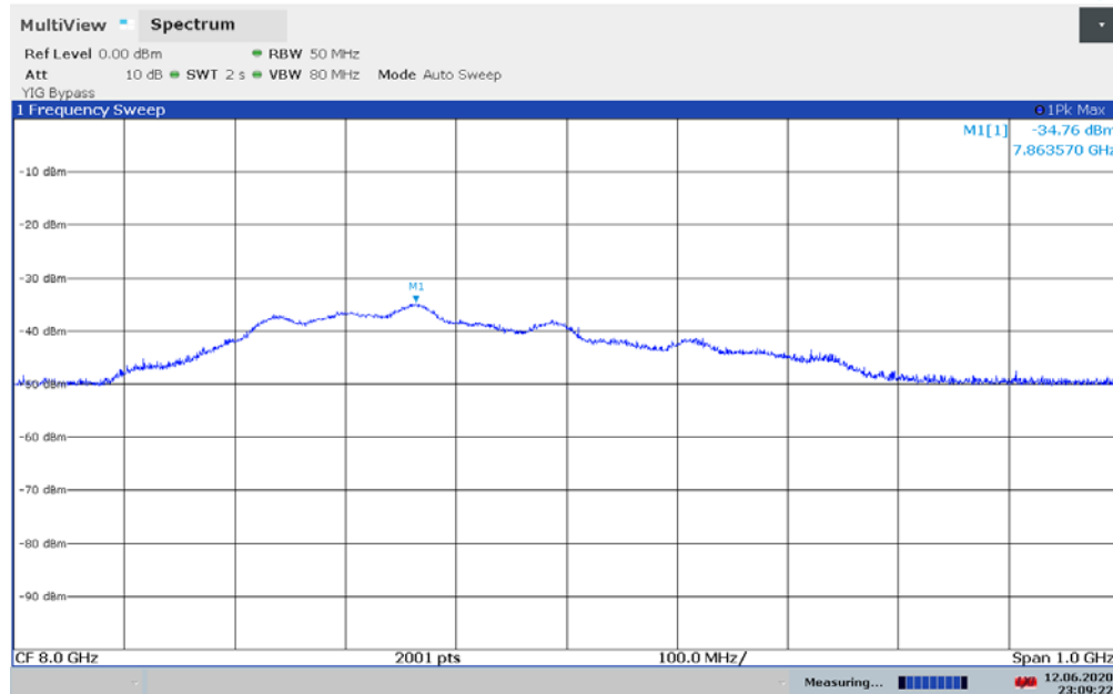
Plot 7-52. UWB Peak Power Measurement - ANT 2 - CH.9 – SP1 – HPRF
