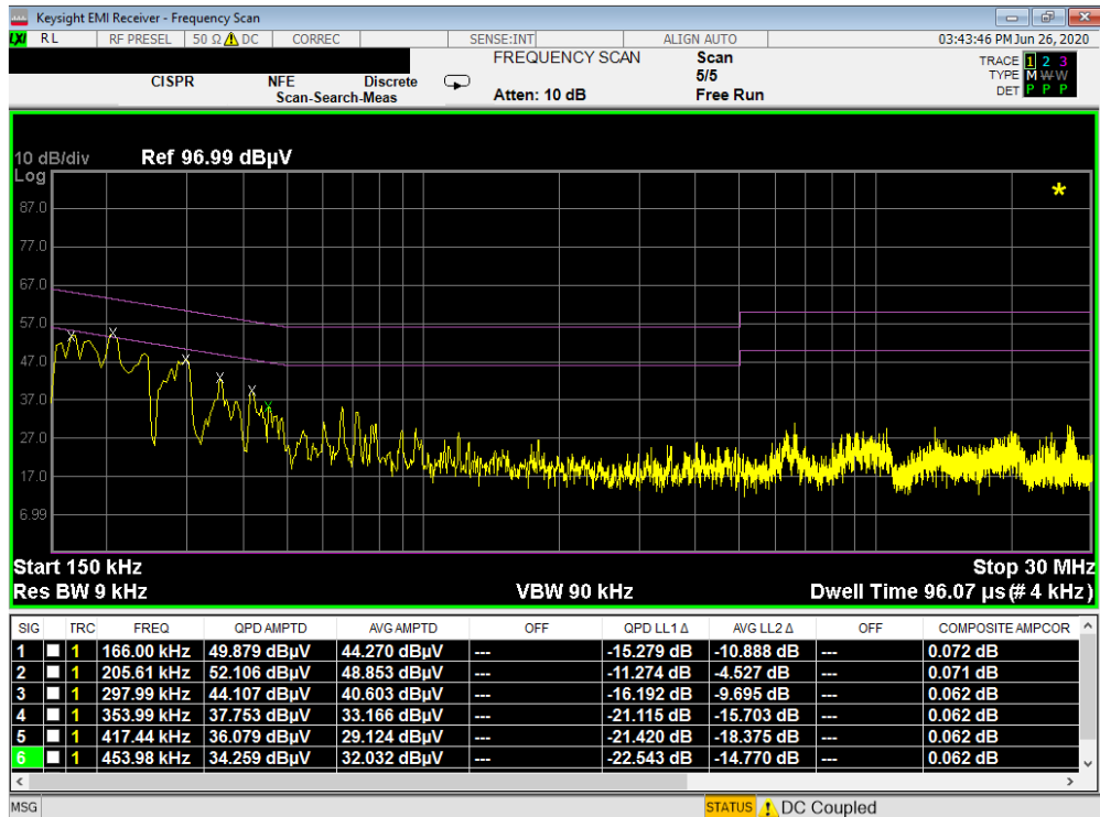
Plot 7-73. Line Conducted Plot (N)
