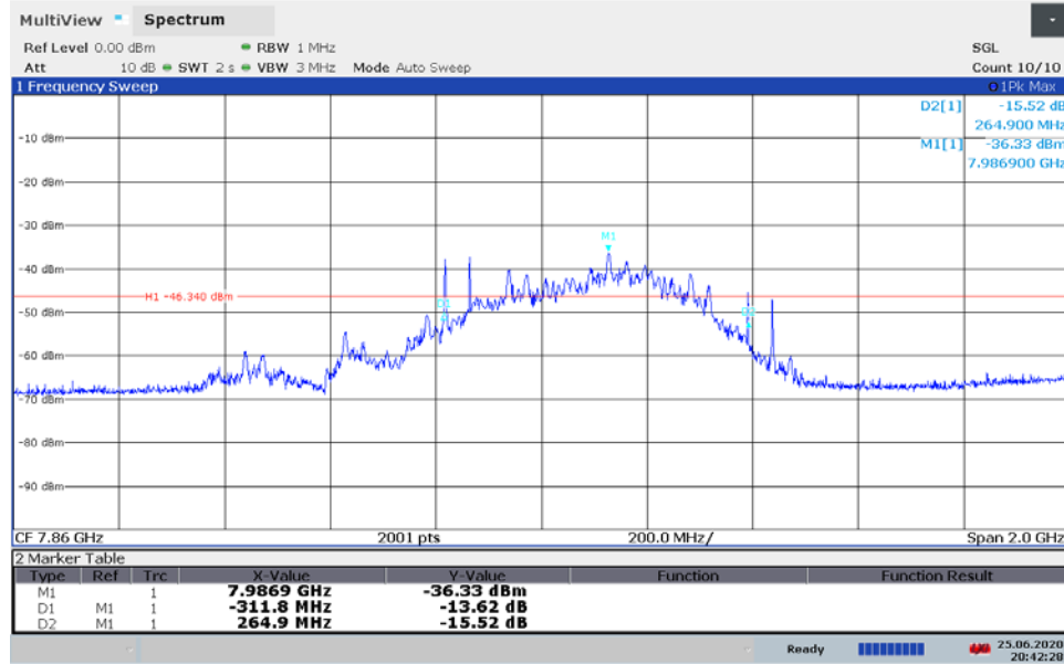
Plot 7-7. BANDWIDTH Plot - ANT1 - CH.9 - SP0 – Preamble 10
