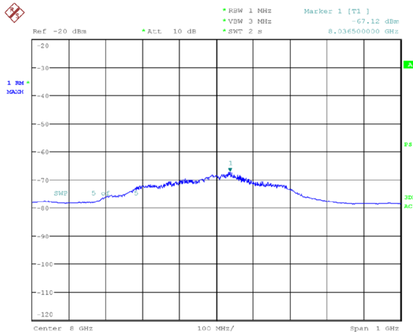
Plot 7-48. UWB Peak Power Measurement - ANT 1 - CH.9 – SP3 – HPRF
