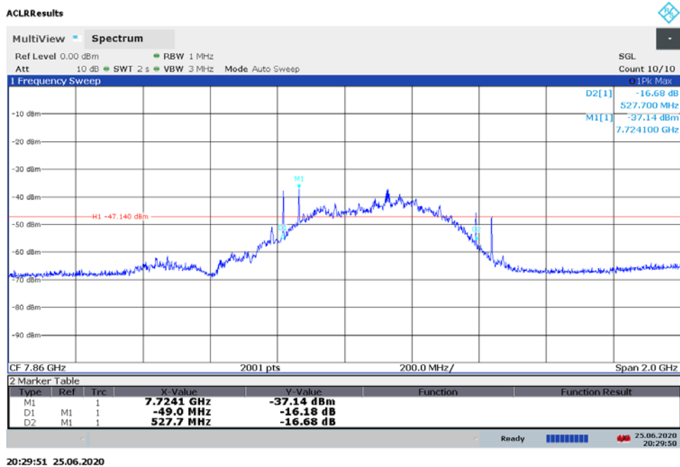
Plot 7-2. BANDWIDTH Plot - ANT1 - CH.9 - SP1 - Preamble 9
