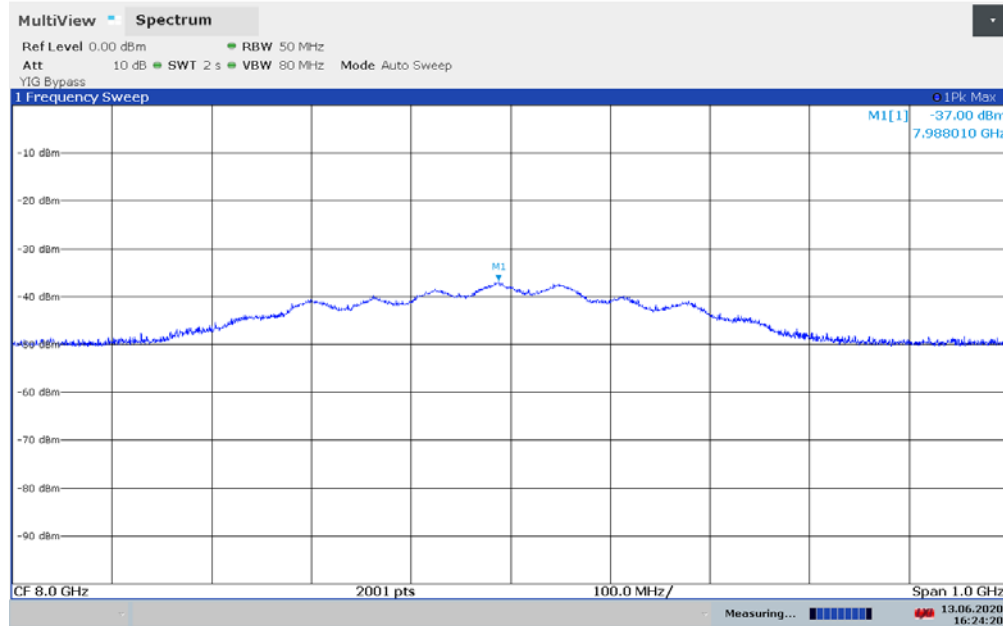
Plot 7-48. UWB Peak Power Measurement - ANT 1 - CH.9 – SP3 – HPRF
