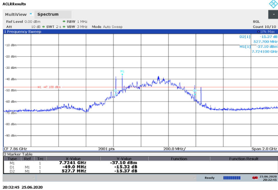
Plot 7-1. BANDWIDTH Plot - ANT1 - CH.9 - SP0 - Preamble 9
