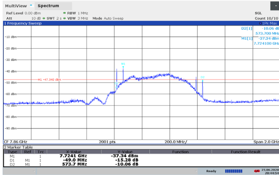
Plot 7-15. BANDWIDTH Plot - ANT1 - CH.9 – SP3 – Preamble 11
