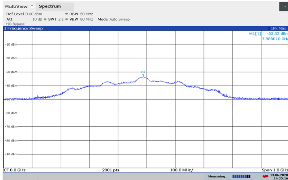
Plot 7-46. UWB Peak Power Measurement - ANT 1 - CH.9 – SP1 – HPRF
