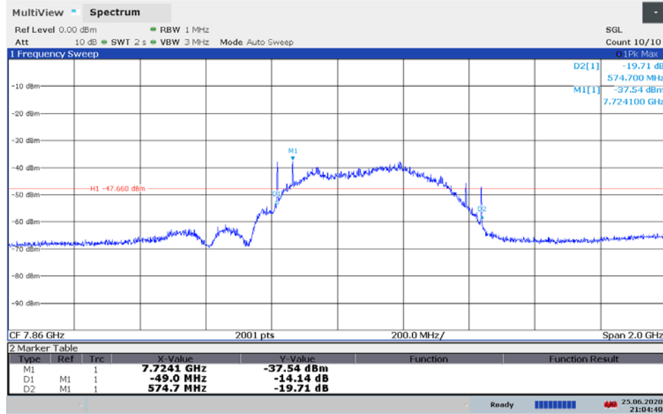
Plot 7-27. BANDWIDTH Plot – ANT1 - CH.9 – SP3 – Preamble 27
