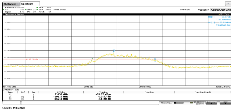
Plot 7-5. BANDWIDTH Plot – ANT2 - CH.9 – SP1 – Preamble 9
