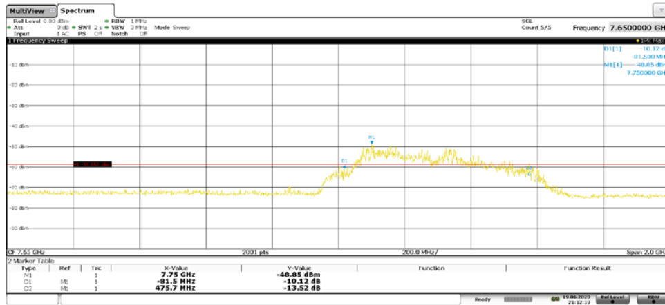
Plot 7-28. BANDWIDTH Plot – ANT2 - CH.9 - SP0 – Preamble 27
