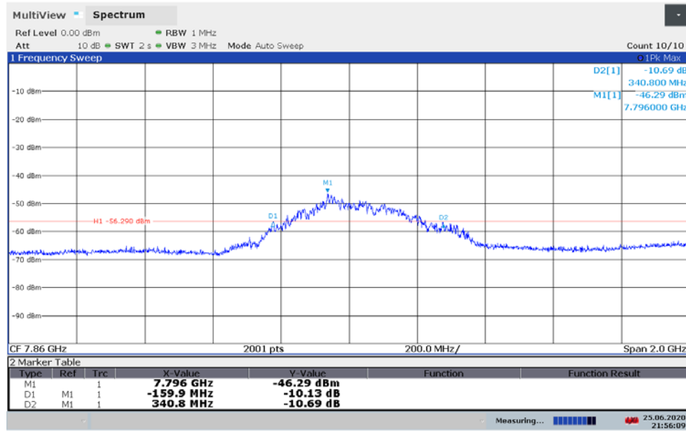
Plot 7-24. BANDWIDTH Plot – ANT2 - CH.9 – SP3 – Preamble 12
