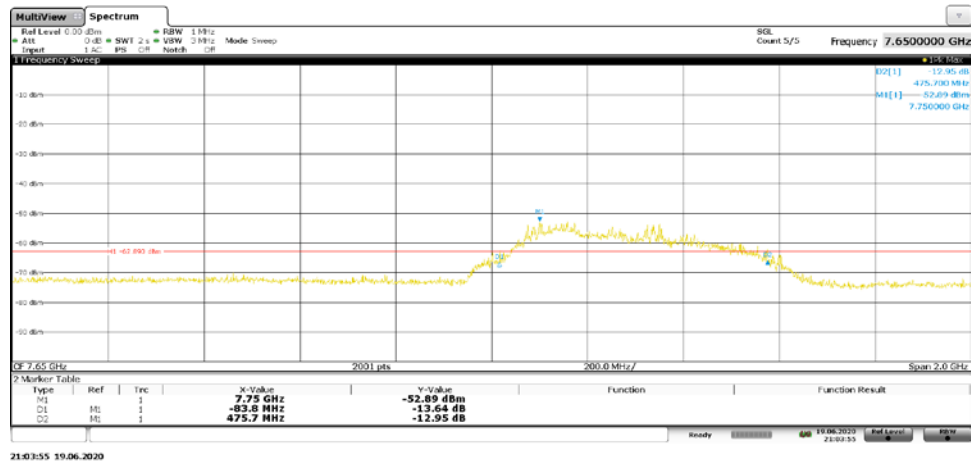
Plot 7-29. BANDWIDTH Plot – ANT2 - CH.9 – SP1 – Preamble 27
