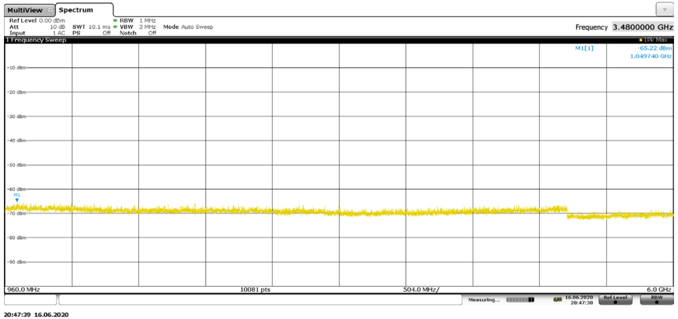
Plot 7-56. Radiated Spurious Pre-Scan 960 - 6000 MHz - CH.9 - ANT 1
