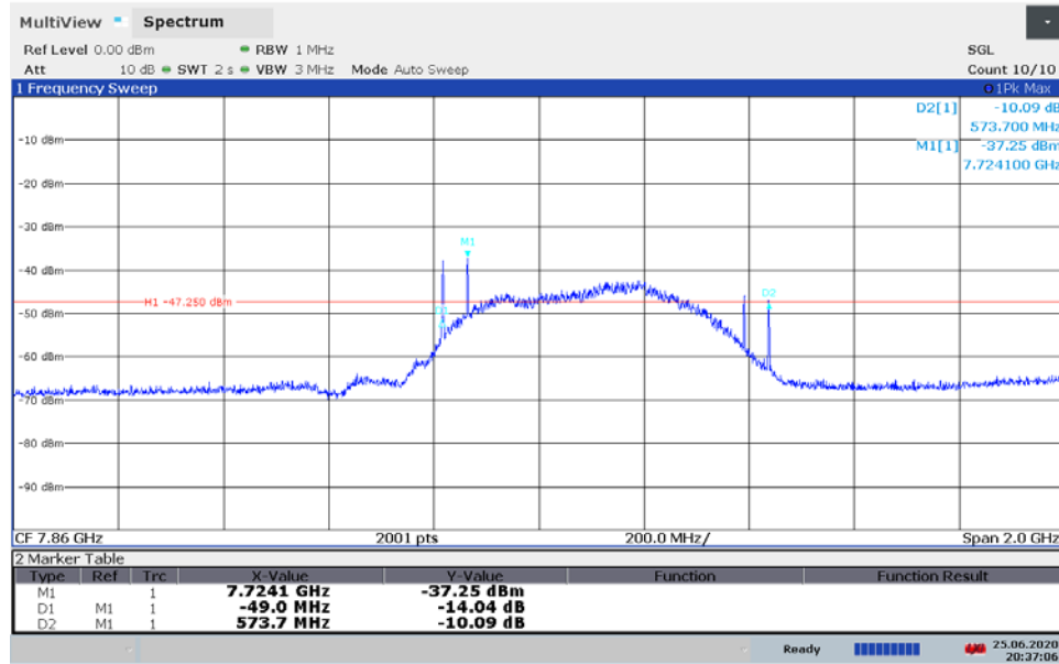
Plot 7-9. BANDWIDTH Plot - ANT1 - CH.9 – SP3 – Preamble 10
