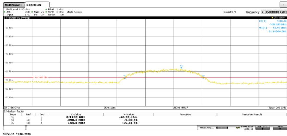
Plot 7-12. BANDWIDTH Plot – ANT2 - CH.9 – SP3 – Preamble 10
