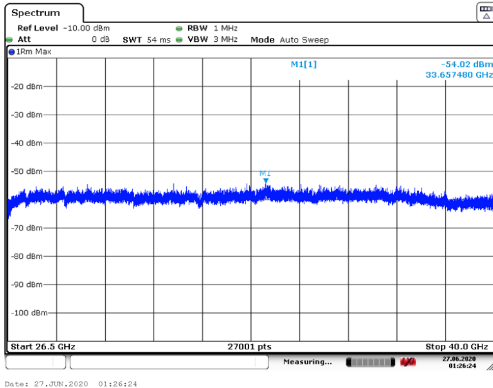
Plot 7-69. Radiated Spurious Pre-Scan 26.5 – 40.0 GHz - CH.9 - ANT 2
