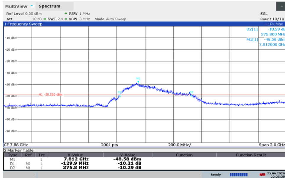
Plot 7-18. BANDWIDTH Plot - ANT1 - CH.9 – SP3 – Preamble 11
