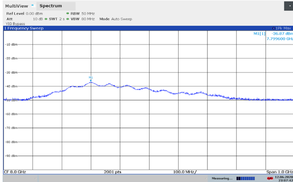
Plot 7-54. UWB Peak Power Measurement - ANT 2 - CH.9 – SP3 – HPRF
