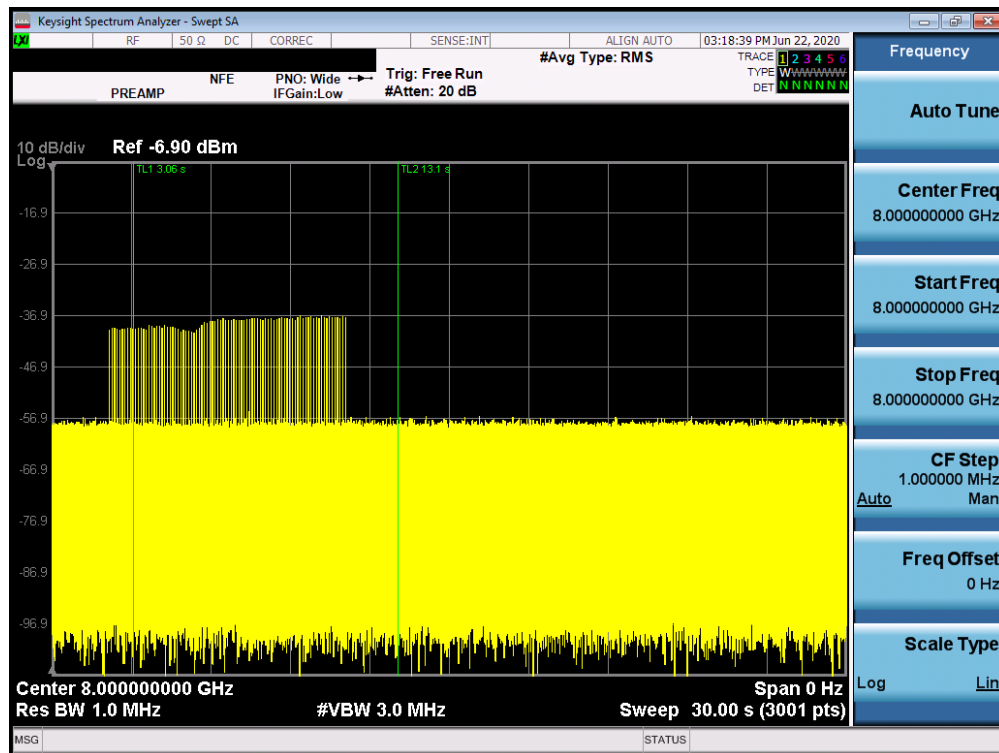
Plot 7-31. Cessation Time Plot
