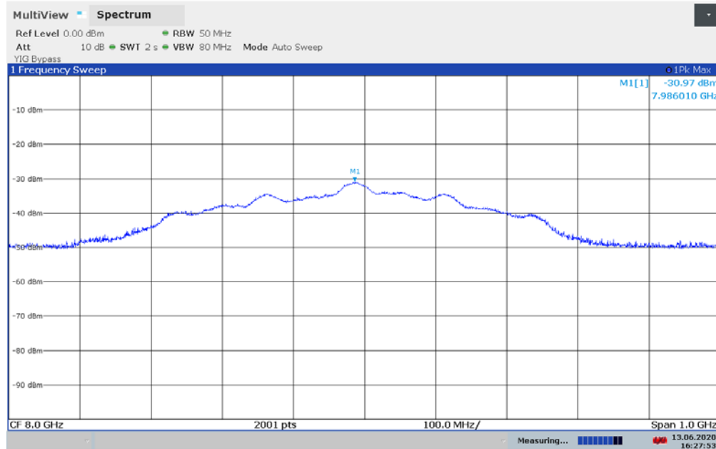
Plot 7-44. UWB Peak Power Measurement - ANT 1 - CH.9 - SP0 – HPRF
