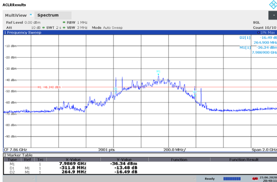
Plot 7-7. BANDWIDTH Plot - ANT1 - CH.9 - SP0 – Preamble 10
