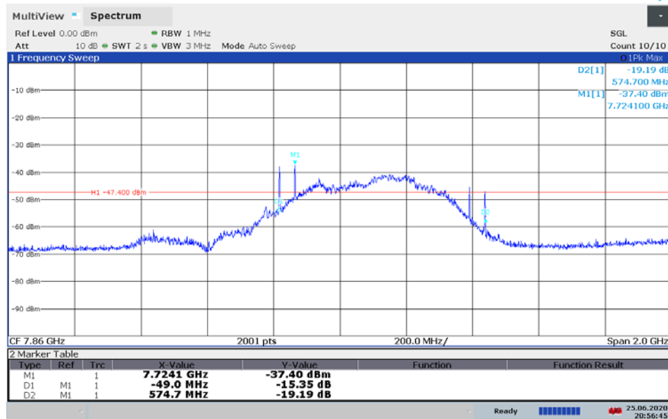
Plot 7-20. BANDWIDTH Plot 7-- ANT1 - CH.9 – SP1 – Preamble 12
