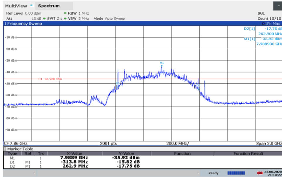
Plot 7-25. BANDWIDTH Plot – ANT1 - CH.9 - SP0 – Preamble 27
