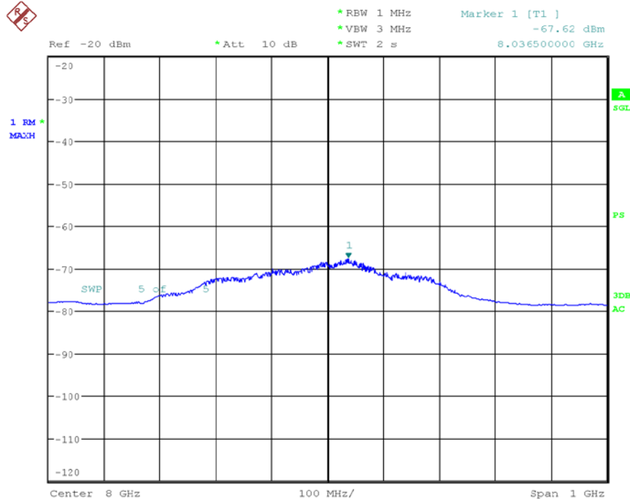
Plot 7-34. UWB Peak Power Measurement - ANT 1 - CH.9 – SP1 – BPRF
