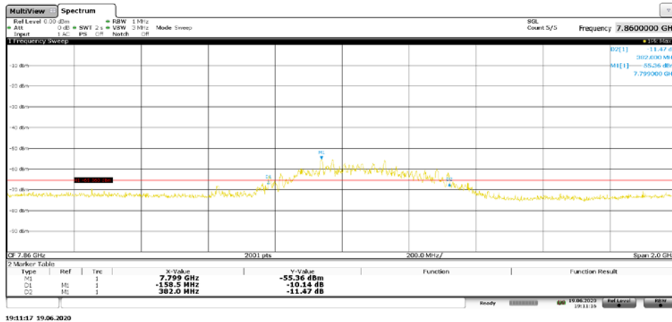
Plot 7-10. BANDWIDTH Plot – ANT2 - CH.9 - SP0 – Preamble 10
