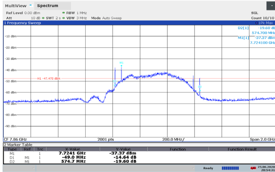
Plot 7-21. BANDWIDTH Plot 7-- ANT1 - CH.9 – SP3 – Preamble 12
