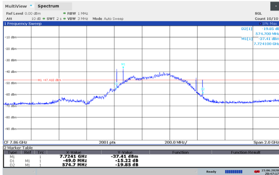
Plot 7-14. BANDWIDTH Plot - ANT1 - CH.9 – SP1 – Preamble 11
