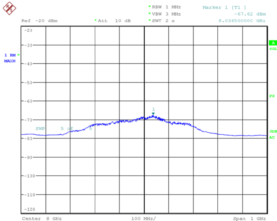
Plot 7-46. UWB Peak Power Measurement - ANT 1 - CH.9 – SP1 – HPRF
