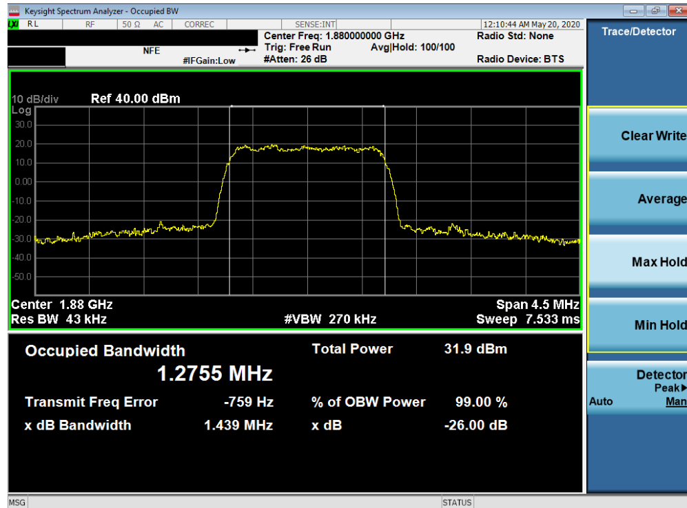
Plot 7-6. Occupied Bandwidth Plot (PCS CDMA Mode)
