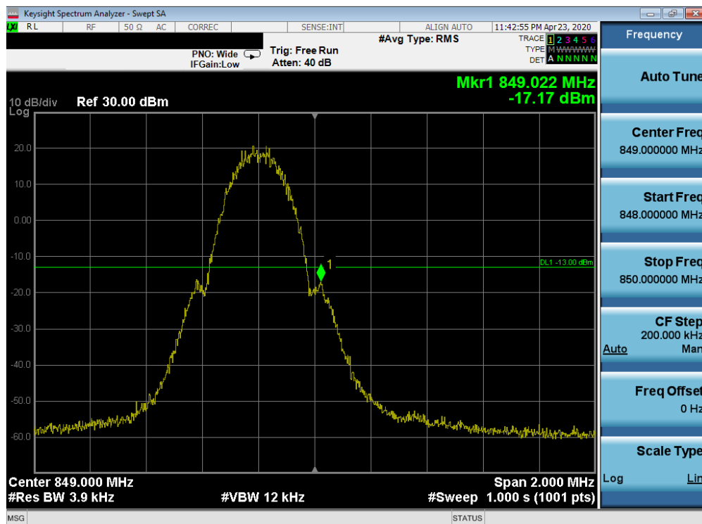
Plot 7-74. Band Edge Plot (CELL GPRS Mode - High Channel)
