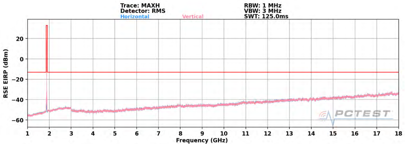
Plot 7-739. Radiated Spurious Plot above 1GHz (n2+ Anchor B13 EN-DC)
