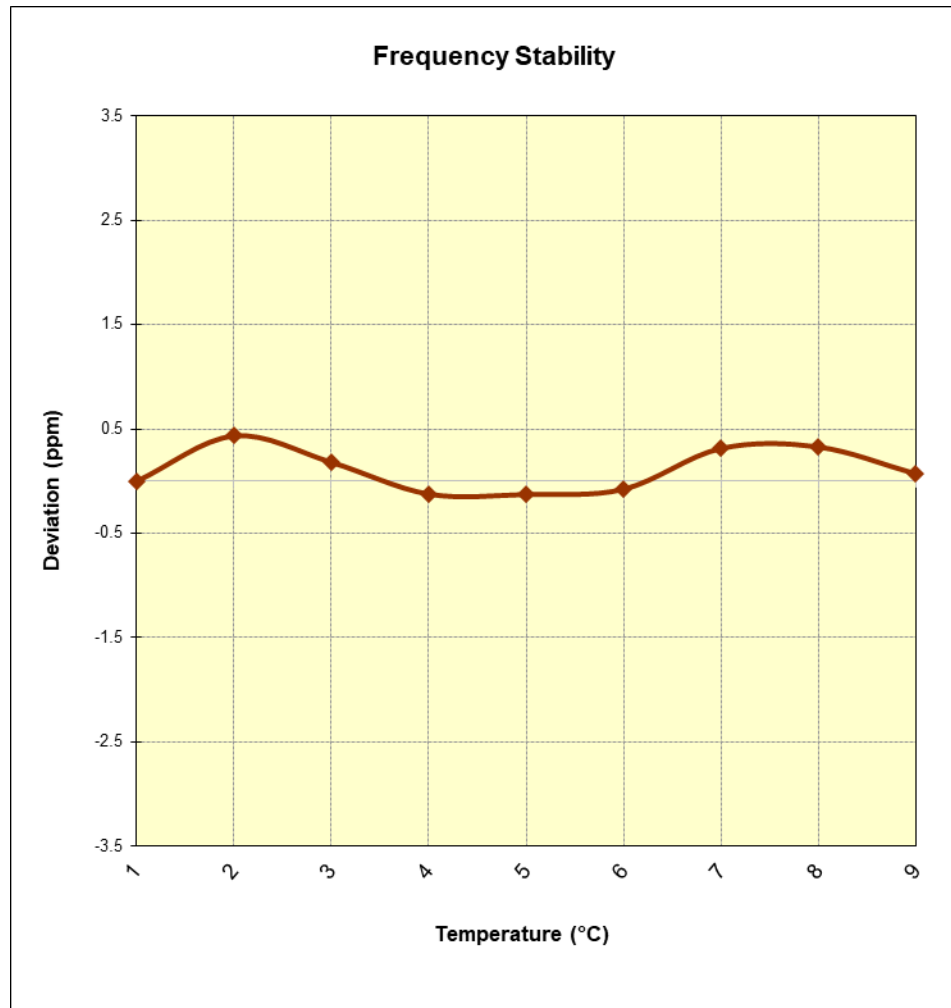
Figure 7-15. Frequency Stability Graph (Band 26/5)
