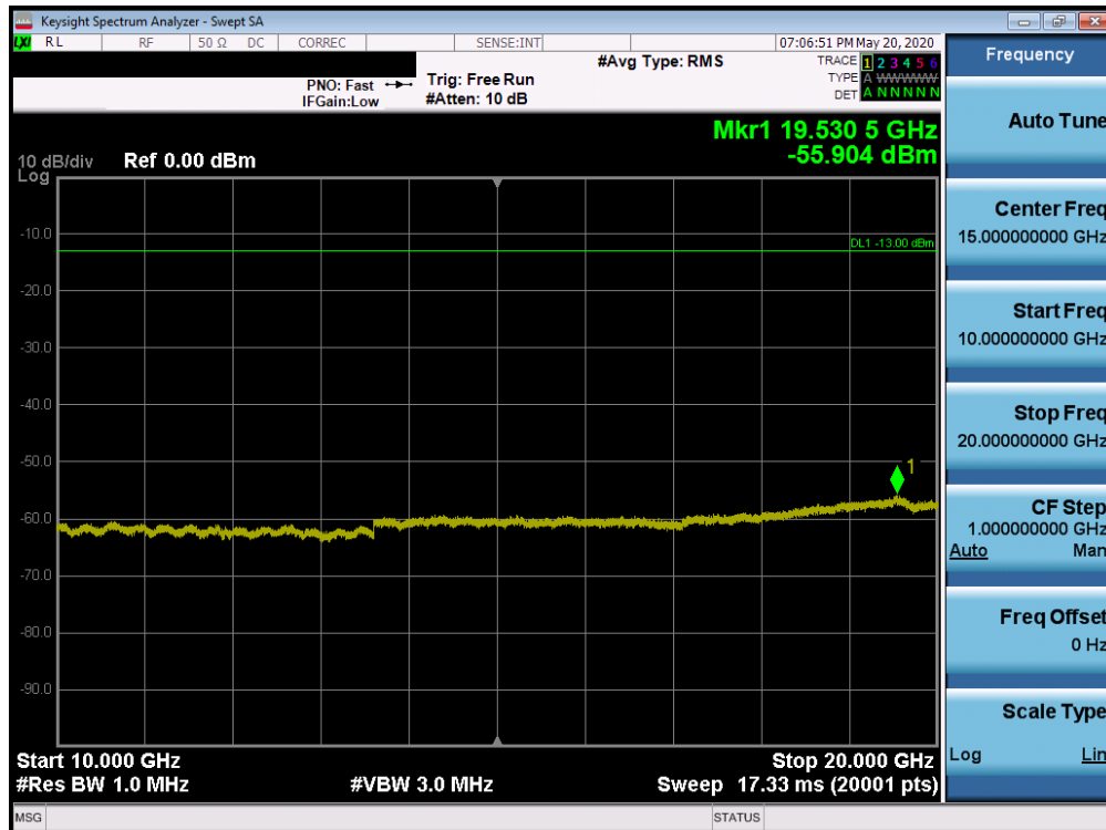
Plot 7-708. Conducted Spurious Plot (Band 66 – 20.0MHz QPSK – PCC 1/99 SCC 1/0 – Mid Channel)
