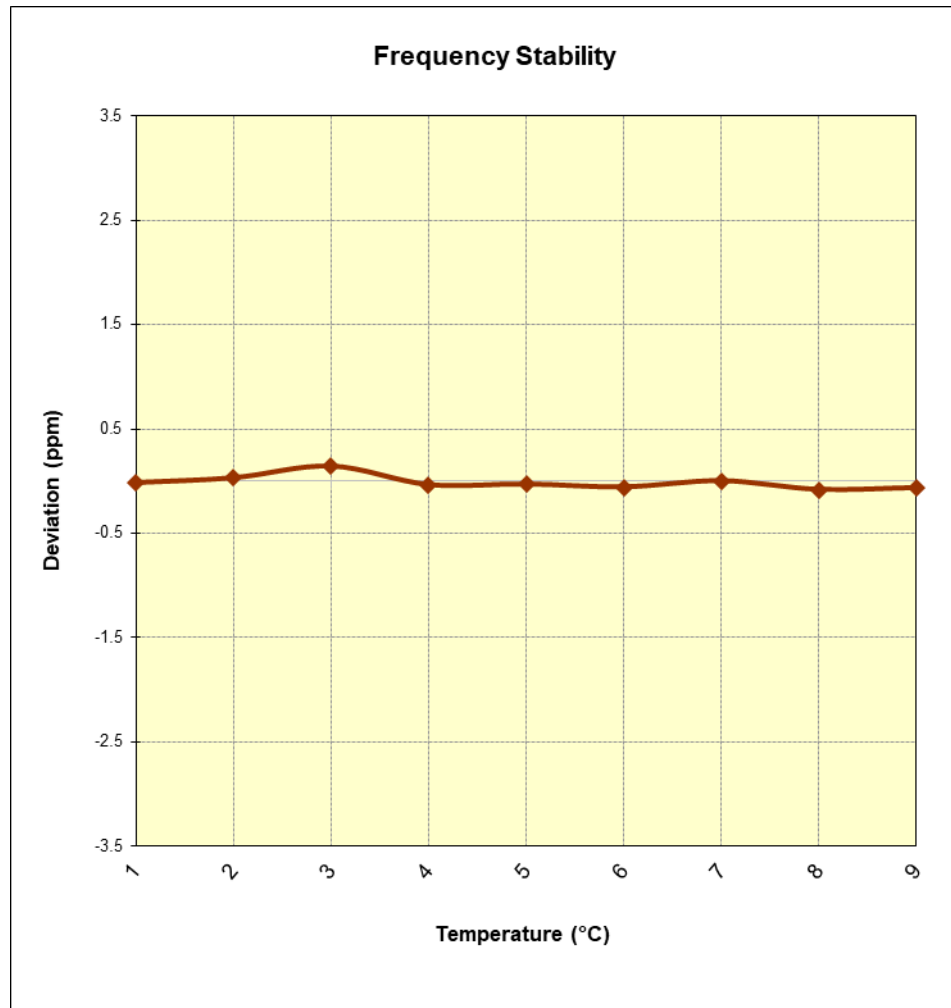
Figure 7-21. Frequency Stability Graph (Band 30)
