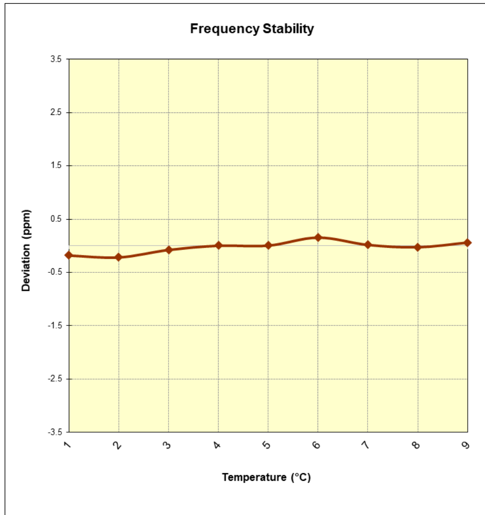
Figure 7-17. Frequency Stability Graph (Band 66/4)
