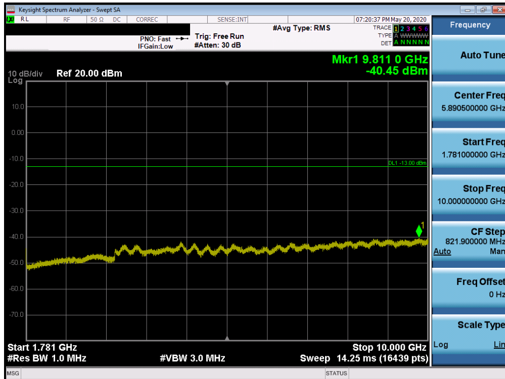
Plot 7-710. Conducted Spurious Plot (Band 66 – 20.0MHz QPSK – PCC 1/0 SCC 1/99 – High Channel)
