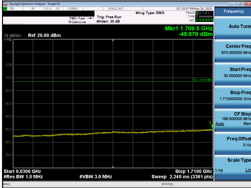
Plot 7-709. Conducted Spurious Plot (Band 66 – 20.0MHz QPSK – PCC 1/0 SCC 1/99 – High Channel)
