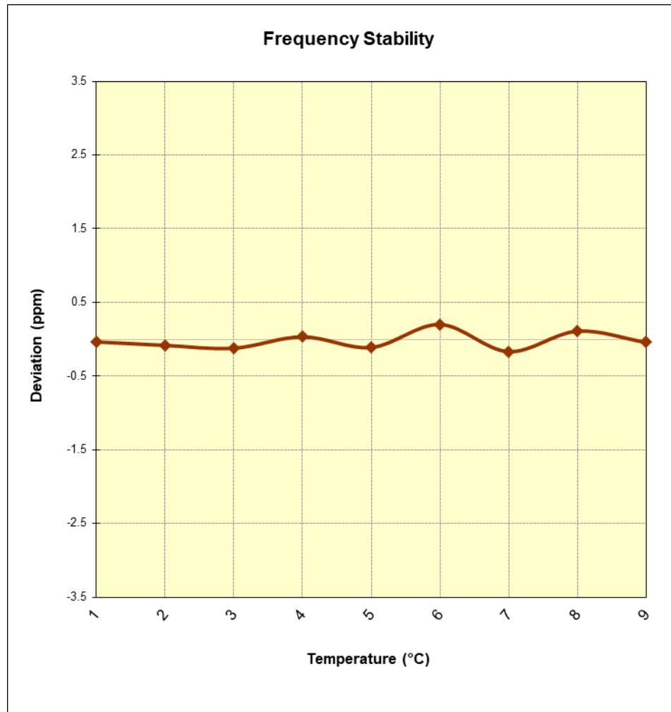
Figure 7-18. Frequency Stability Graph (Band n66)
