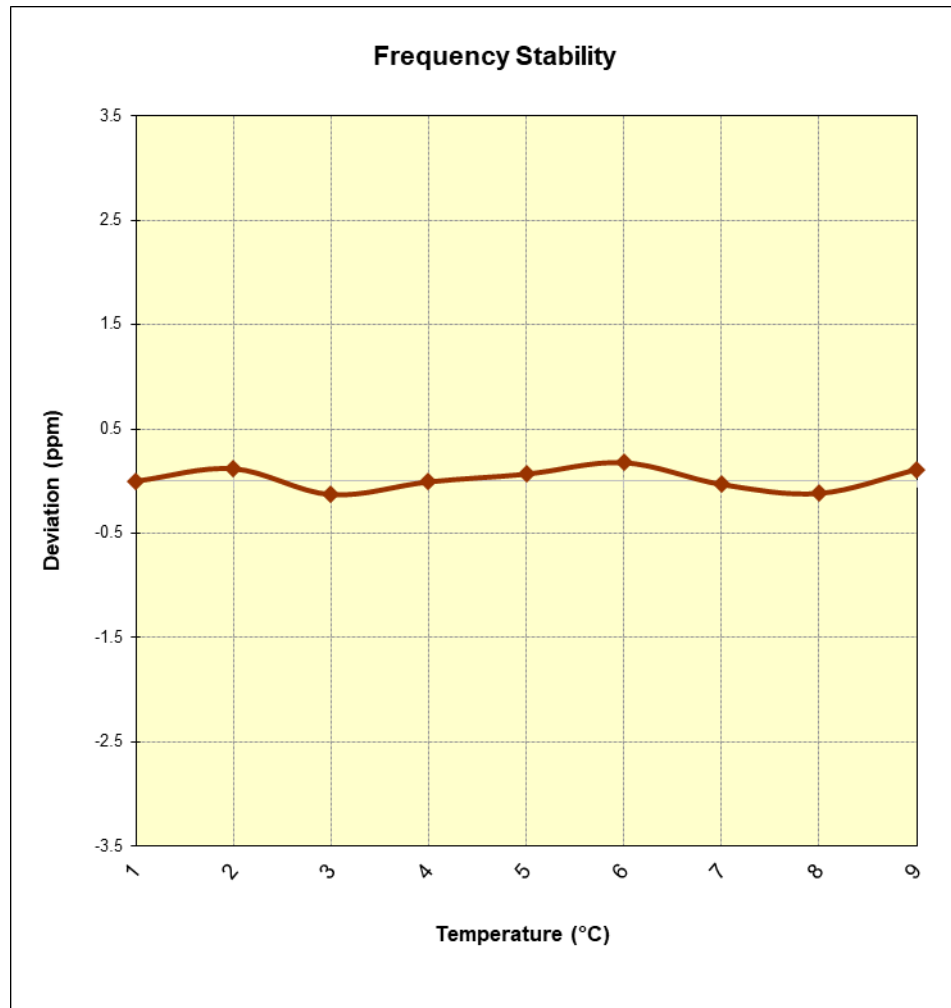
Figure 7-22. Frequency Stability Graph (Band 41)
