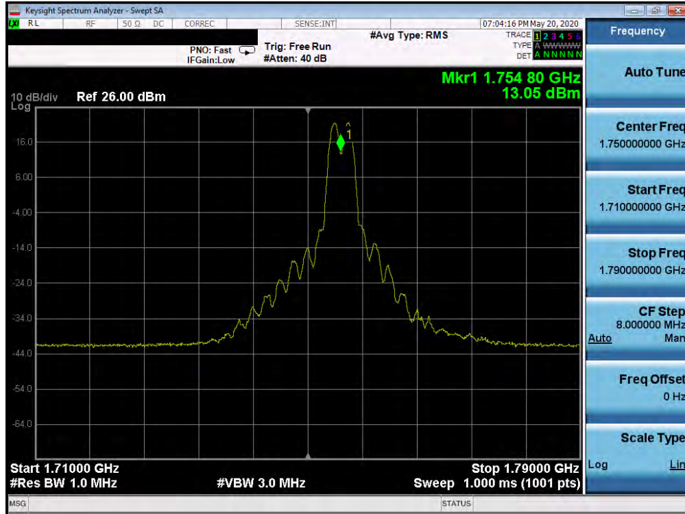
Plot 7-707. Conducted Spurious Plot (Band 66 – 20.0MHz QPSK – PCC 1/99 SCC 1/0 – Mid Channel)
