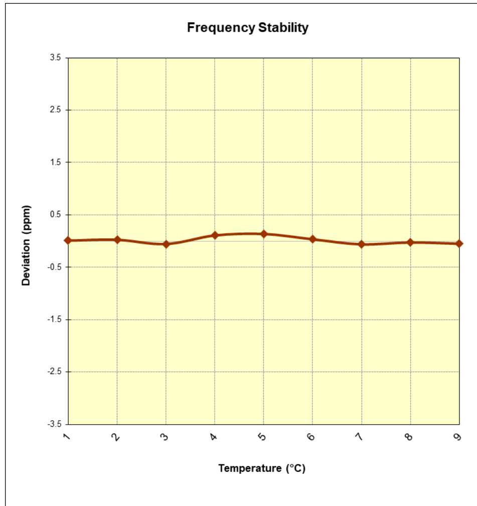
Figure 7-23. Frequency Stability Graph (Band n41)
