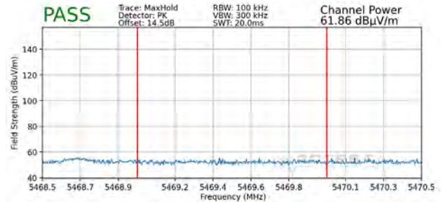
Plot 7-374. Radiated Lower Band Edge Plot SISO ANT1 (Peak - UNII Band 2C - 996 Tones)
