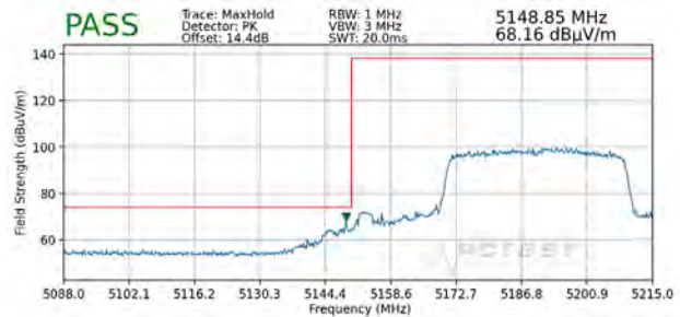
Plot 7-384. Radiated Lower Band Edge Plot SISO ANT2 (Peak - UNII Band 1 - 484 Tones)
