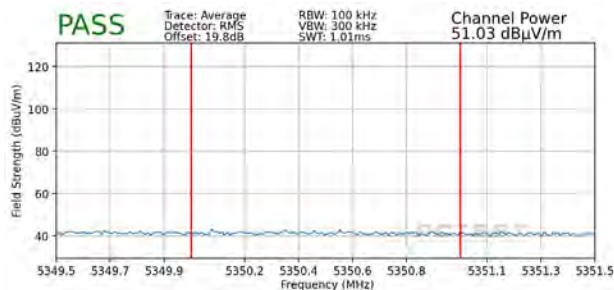
Plot 7-364. Radiated Upper Band Edge Plot SISO ANT1 (Average - UNII Band 2A - 484 Tones)
