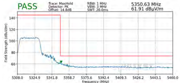
Plot 7-400. Radiated Upper Band Edge Plot MIMO (Peak - UNII Band 2A - 242 Tones)
