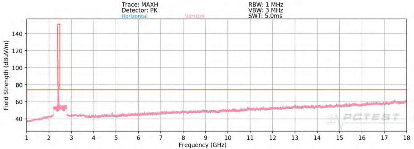
Plot 7-60. Radiated Spurious Plot above 1GHz SISO ANT1 (802.11ax OFDMA - 242 Tones - Ch. 1)
