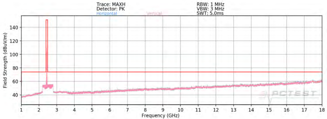
Plot 7-66. Radiated Spurious Plot above 1GHz SISO ANT2 (802.11ax OFDMA – 106 Tones – Ch. 6)
