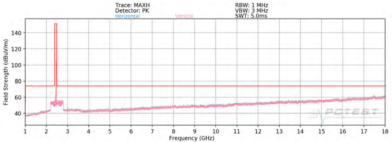
Plot 7-62. Radiated Spurious Plot above 1GHz SISO ANT1 (802.11ax OFDMA - 242 Tones - Ch. 11)
