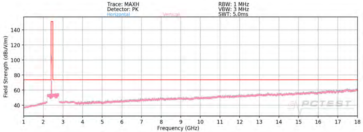
Plot 7-65. Radiated Spurious Plot above 1GHz SISO ANT2 (802.11ax OFDMA – 106 Tones – Ch. 1)
