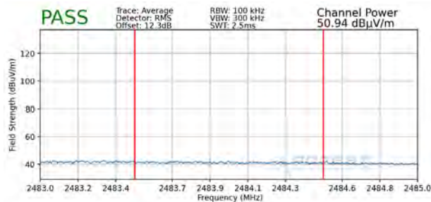
Plot 7-103. Radiated Restricted Upper Band Edge Measurement SISO ANT2 (Average – 242 Tones)
