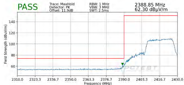
Plot 7-88. Radiated Restricted Lower Band Edge Measurement SISO ANT1 (Peak - 242 Tones)
