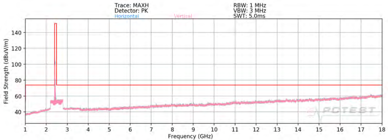
Plot 7-68. Radiated Spurious Plot above 1GHz SISO ANT2 (802.11ax OFDMA - 242 Tones - Ch. 1)
