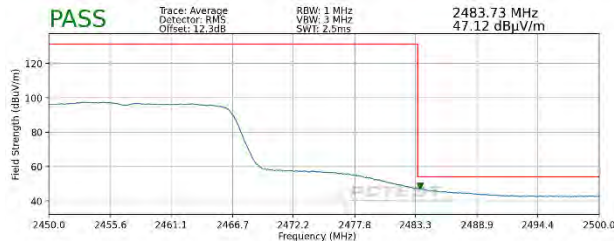
Plot 7-113. Radiated Restricted Upper Band Edge Measurement MIMO (Average – 242 Tones)
