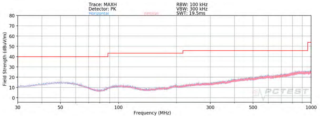
Plot 7-118. Radiated Spurious Plot below 1GHz MIMO (242 Tones)
