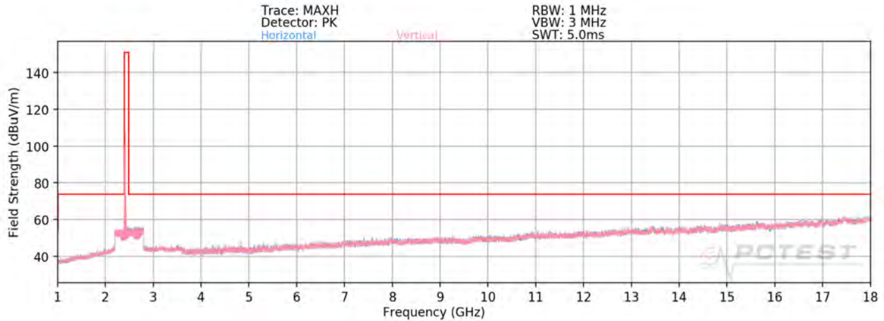
Plot 7-73. Radiated Spurious Plot above 1GHz MIMO (802.11ax OFDMA – 106 Tones – Ch. 1)
