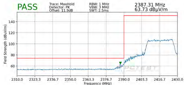
Plot 7-100. Radiated Restricted Lower Band Edge Measurement SISO ANT2 (Peak - 242 Tones)
