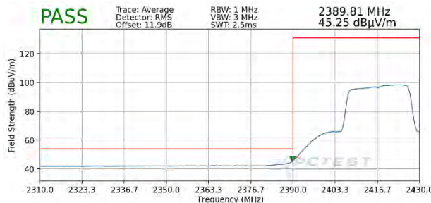
Plot 7-87. Radiated Restricted Lower Band Edge Measurement SISO ANT1 (Average - 242 Tones)
