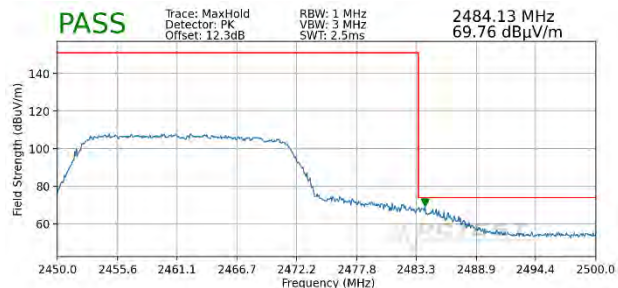
Plot 7-116. Radiated Restricted Upper Band Edge Measurement MIMO (Peak – 242 Tones)
