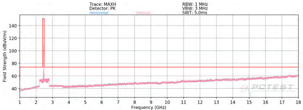
Plot 7-75. Radiated Spurious Plot above 1GHz MIMO (802.11ax OFDMA – 106 Tones – Ch. 11)
