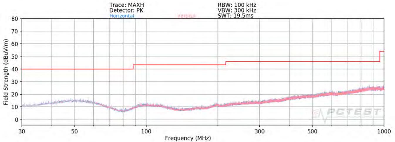
Plot 7-117. Radiated Spurious Plot below 1GHz MIMO (106 Tones)
