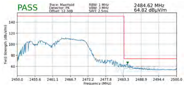
Plot 7-108. Radiated Restricted Upper Band Edge Measurement MIMO (Peak – 106 Tones)
