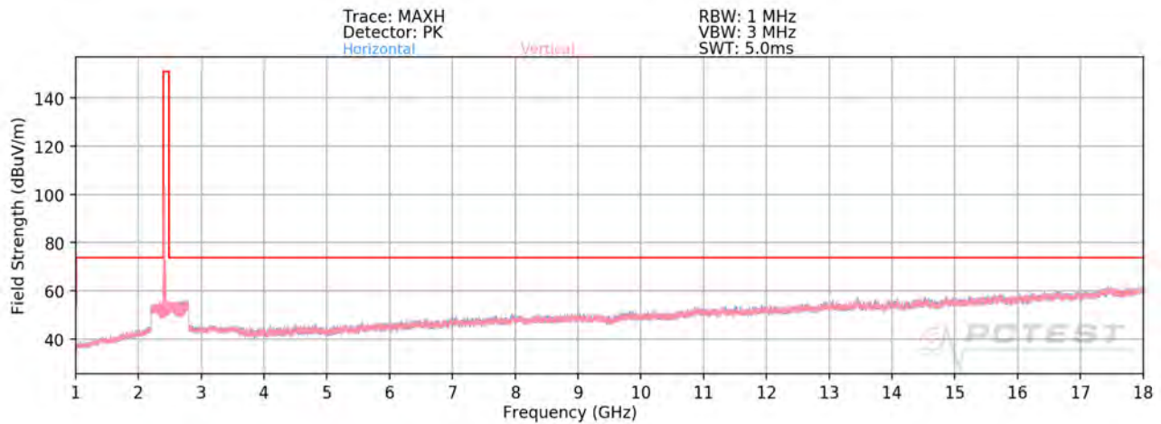
Plot 7-76. Radiated Spurious Plot above 1GHz MIMO (802.11ax OFDMA – 242 Tones – Ch. 1)
