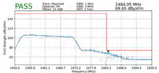
Plot 7-92. Radiated Restricted Upper Band Edge Measurement SISO ANT1 (Peak - 242 Tones)
