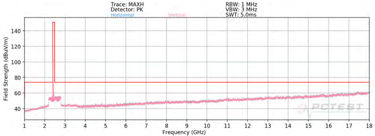
Plot 7-57. Radiated Spurious Plot above 1GHz SISO ANT1 (802.11ax OFDMA – 106 Tones – Ch. 1)
