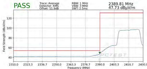
Plot 7-99. Radiated Restricted Lower Band Edge Measurement SISO ANT2 (Average - 242 Tones)
