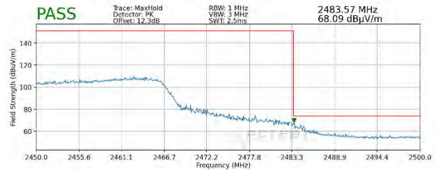
Plot 7-102. Radiated Restricted Upper Band Edge Measurement SISO ANT2 (Peak – 242 Tones)
