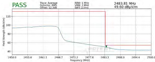
Plot 7-101. Radiated Restricted Upper Band Edge Measurement SISO ANT2 (Average – 242 Tones)
