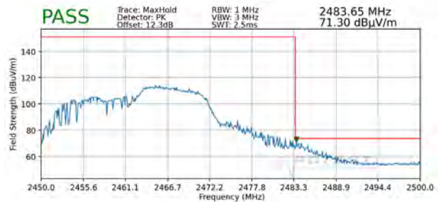
Plot 7-96. Radiated Restricted Upper Band Edge Measurement SISO ANT2 (Peak – 106 Tones)
