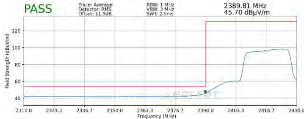
Plot 7-111. Radiated Restricted Lower Band Edge Measurement MIMO (Average – 242 Tones)
