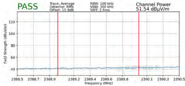
Plot 7-97. Radiated Restricted Lower Band Edge Measurement SISO ANT2 (Average - 242 Tones)
