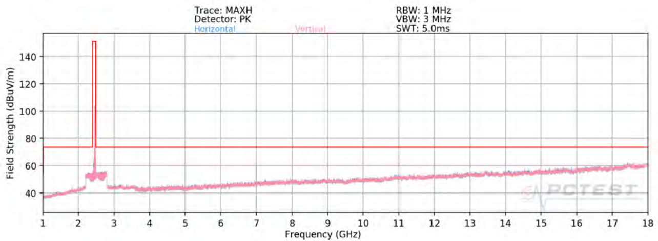
Plot 7-78. Radiated Spurious Plot above 1GHz MIMO (802.11ax OFDMA – 242 Tones – Ch. 11)
