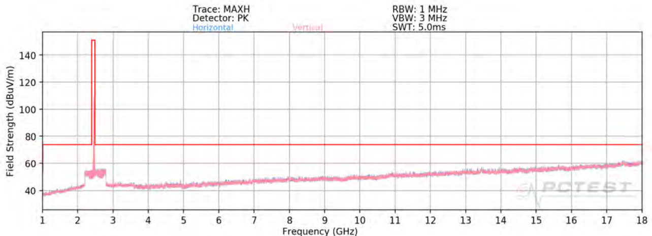
Plot 7-59. Radiated Spurious Plot above 1GHz SISO ANT1 (802.11ax OFDMA – 106 Tones – Ch. 11)
