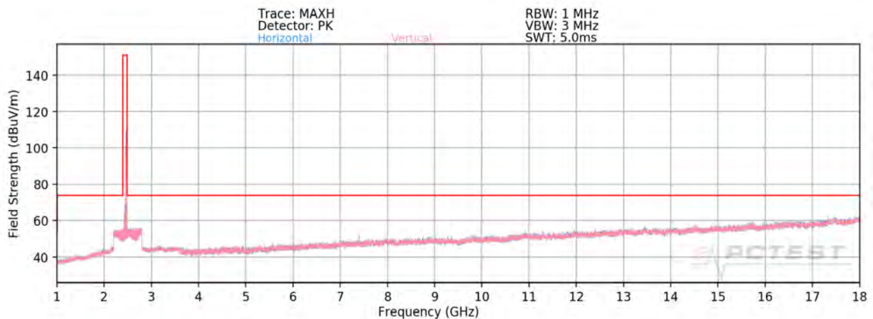
Plot 7-67. Radiated Spurious Plot above 1GHz SISO ANT2 (802.11ax OFDMA – 106 Tones – Ch. 11)
