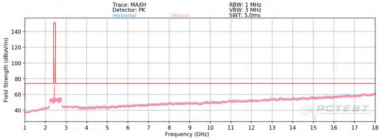
Plot 7-74. Radiated Spurious Plot above 1GHz MIMO (802.11ax OFDMA – 106 Tones – Ch. 6)
