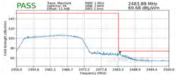
Plot 7-114. Radiated Restricted Upper Band Edge Measurement MIMO (Peak – 242 Tones)
