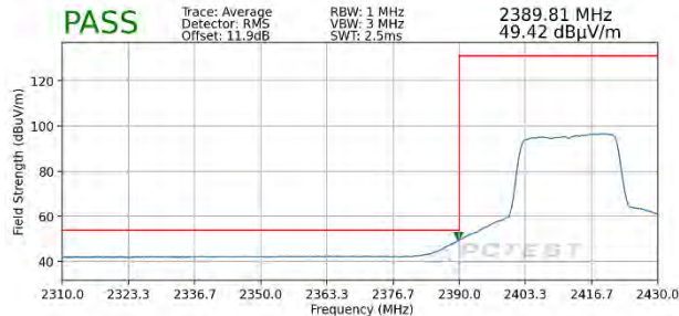
Plot 7-109. Radiated Restricted Lower Band Edge Measurement MIMO (Average – 242 Tones)
