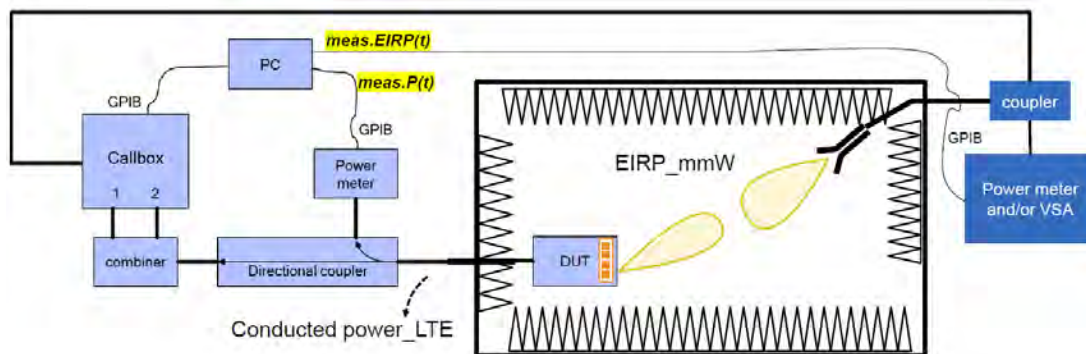
Figure 7-1 mmW NR radiated power measurement setup – Test Setup Photo 7
