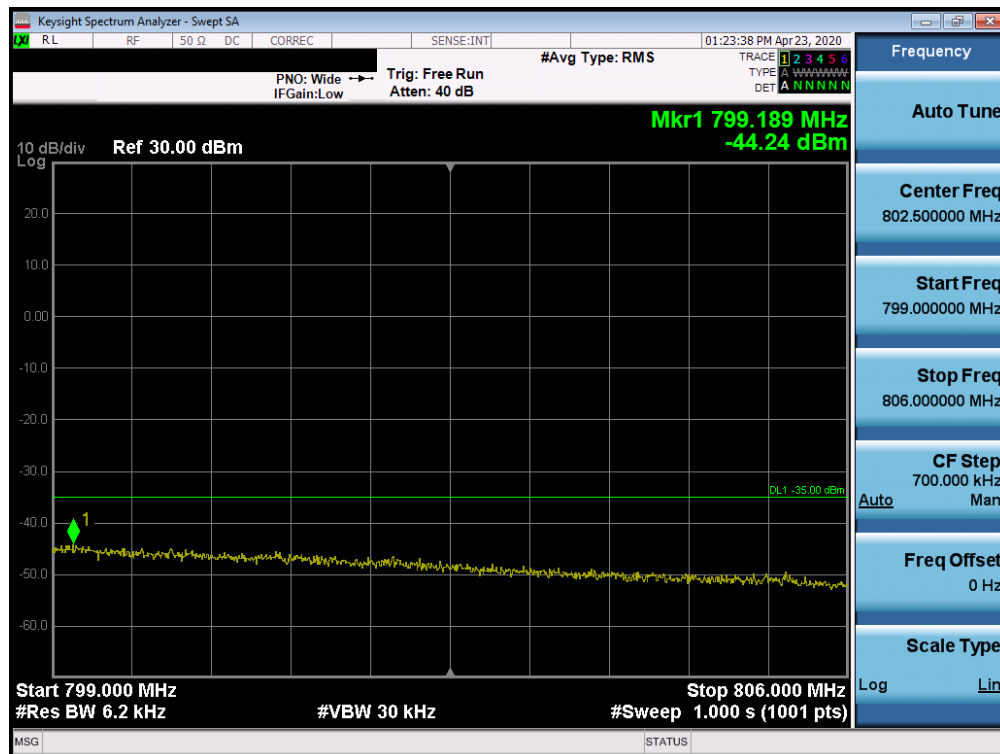
Plot 7-54. Upper Extended Band Edge Plot (Band 14 - 10MHz QPSK - Full RB Configuration)
