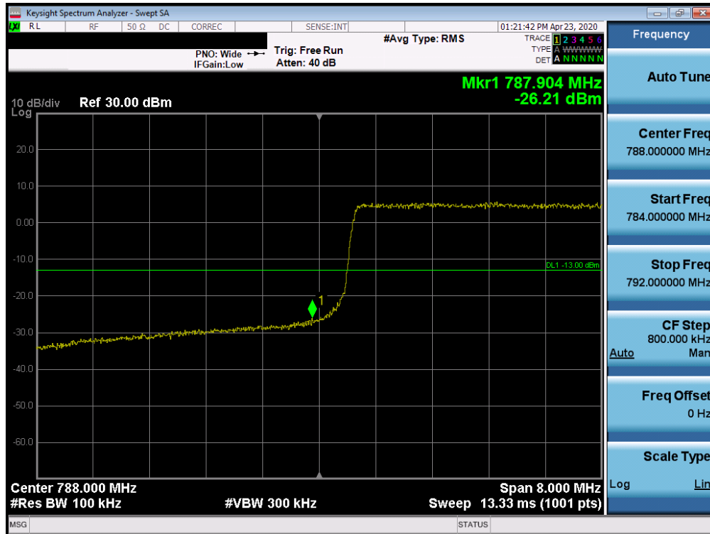
Plot 7-51. Lower Band Edge Plot (Band 14 - 10MHz QPSK - Full RB Configuration)
