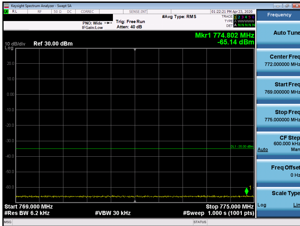
Plot 7-52. Lower Extended Band Edge Plot (Band 14 - 10MHz QPSK - Full RB Configuration)
