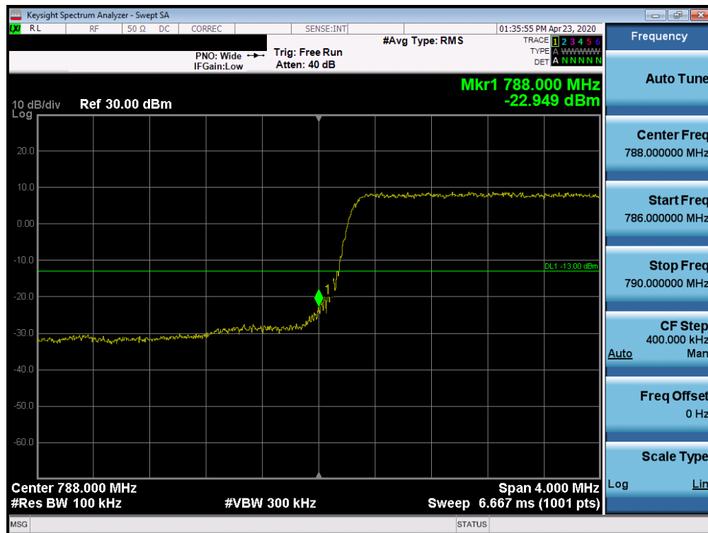
Plot 7-55. Lower Band Edge Plot (Band 14 - 5MHz QPSK - Full RB Configuration)
