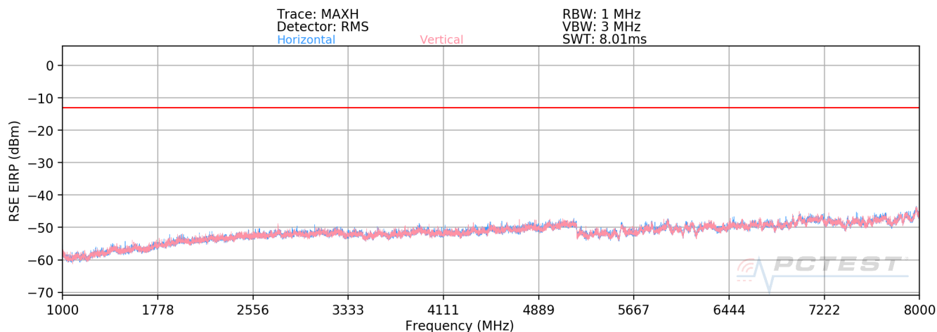
Plot 7-63. Radiated Spurious Plot (Band 14)
