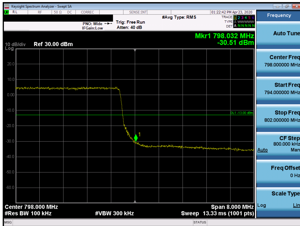
Plot 7-53. Upper Band Edge Plot (Band 14 - 10MHz QPSK - Full RB Configuration)
