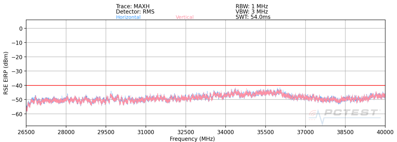
Plot 7-71. Radiated Spurious Plot 26.5 - 40GHz (Band 48)
