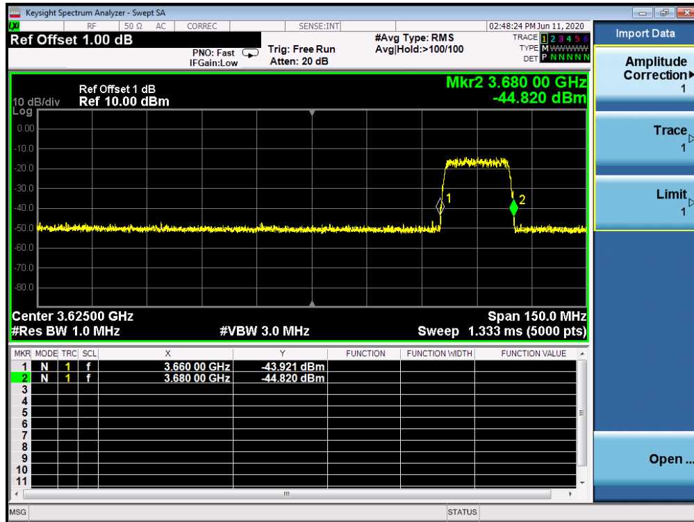
Plot 7-78. Run#2 End User Device Frequency of Operations
