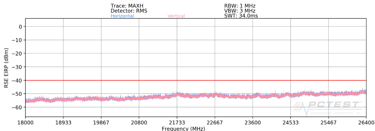
Plot 7-75. Radiated Spurious Plot 18GHz – 26.5GHz (ULCA Band 48)
