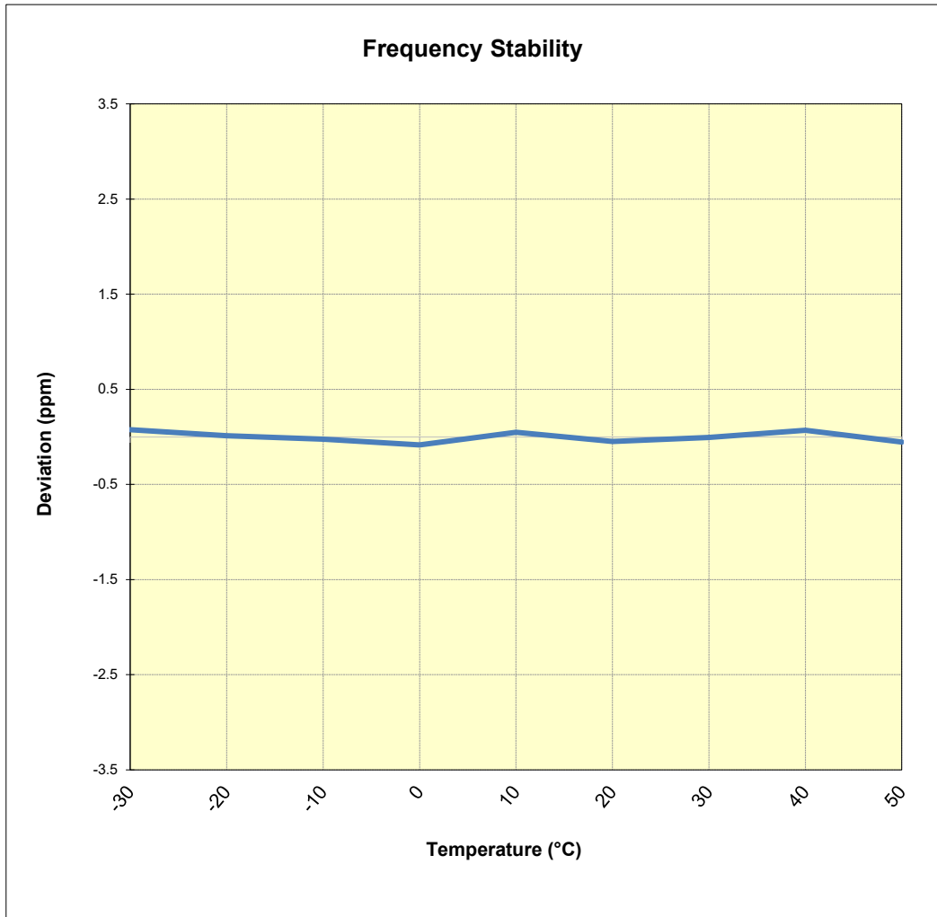
Figure 7-9. Frequency Stability Graph (LTE Band 48)
