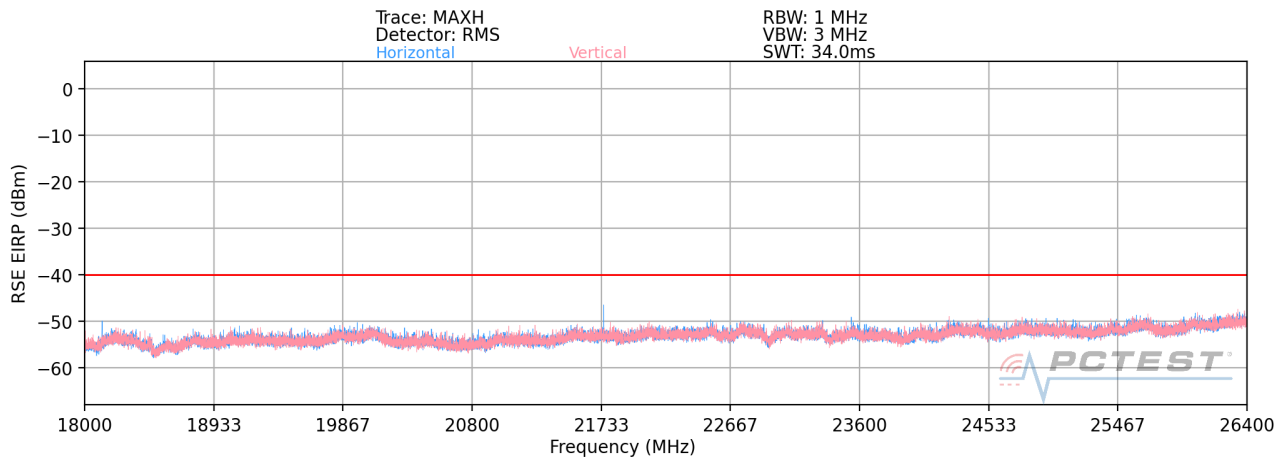
Plot 7-70. Radiated Spurious Plot 18 - 26.5GHz (Band 48)
