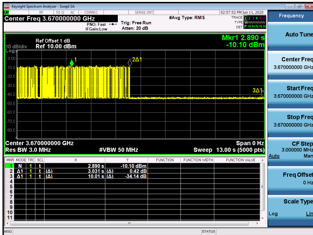
Plot 7-79. Run#2 End User Device Discontinues Operations within 10s
