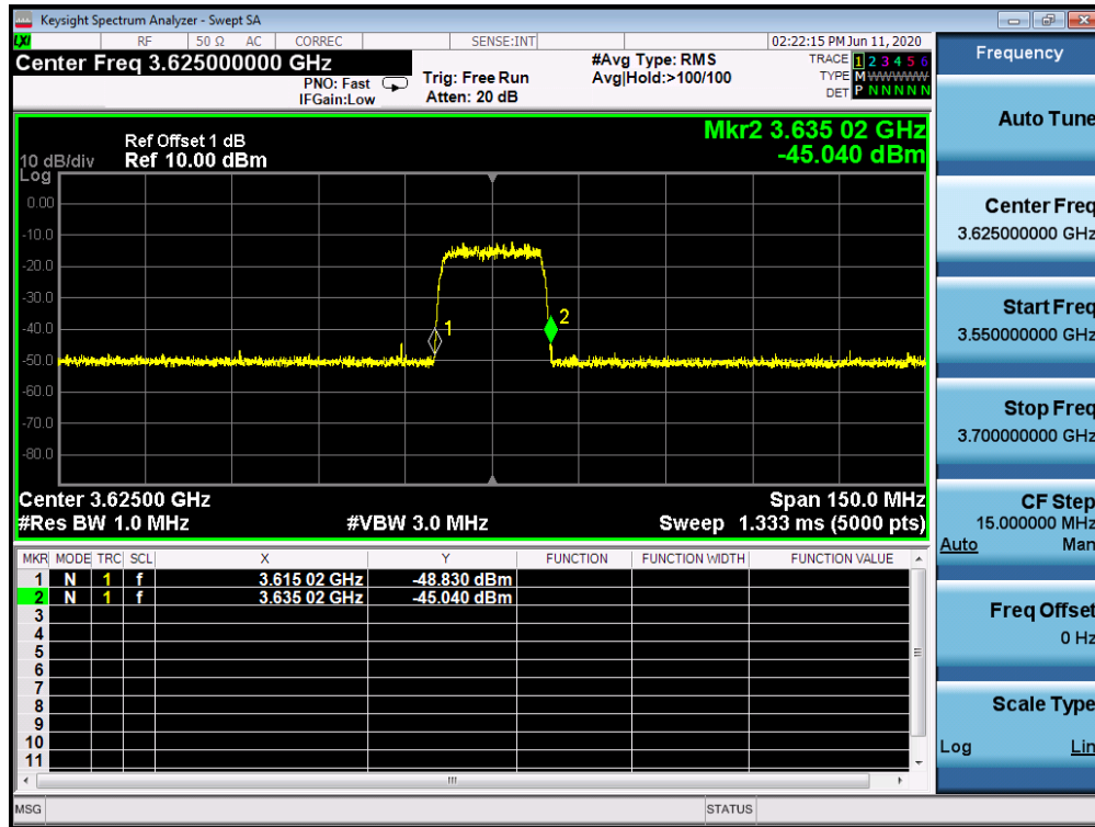
Plot 7-76. Run#1 End User Device Frequency of Operations
