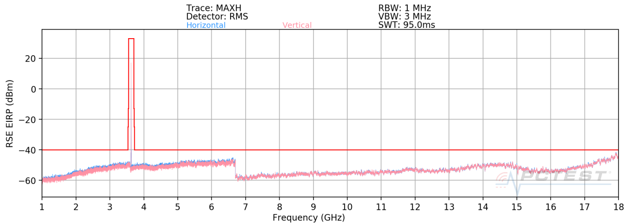
Plot 7-69. Radiated Spurious Plot 1 - 18GHz (Band 48)
